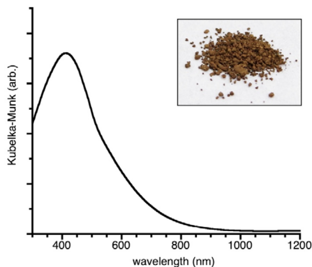
Figure 4. Diffuse reflectance spectrum of conjugated imine polymer 17 . Inset shows the picture of polymer 17 under ambient light.
