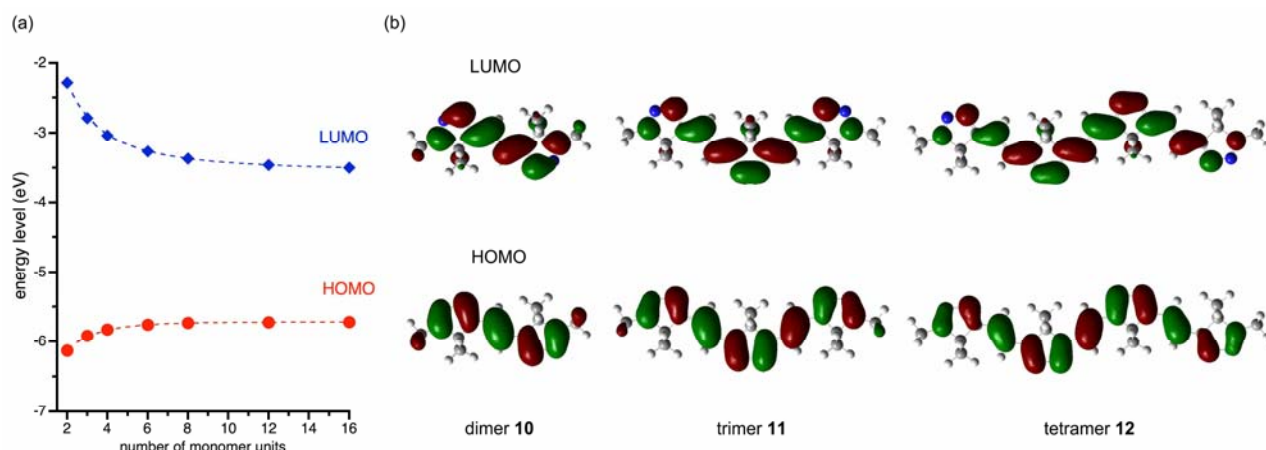
Figure 5. (a) Energy levels of frontier orbitals for conjugated oligoimines 10–12 . (b) Kohn–Sham orbitals (top: LUMO, bottom: HOMO) of 10–12 .
