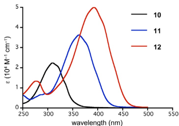
Figure 2. UV-Vis absorption spectra of conjugated imines 10–12 in \text{CH}_2\text{Cl}_2 .
