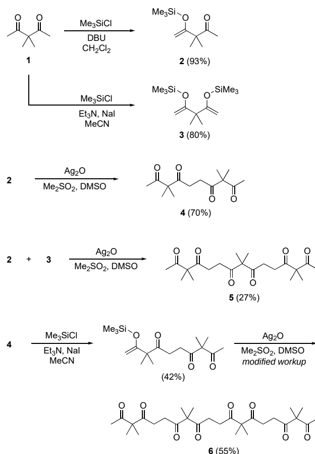
Scheme 1. Synthesis of discrete oligoketones 4–6 .
