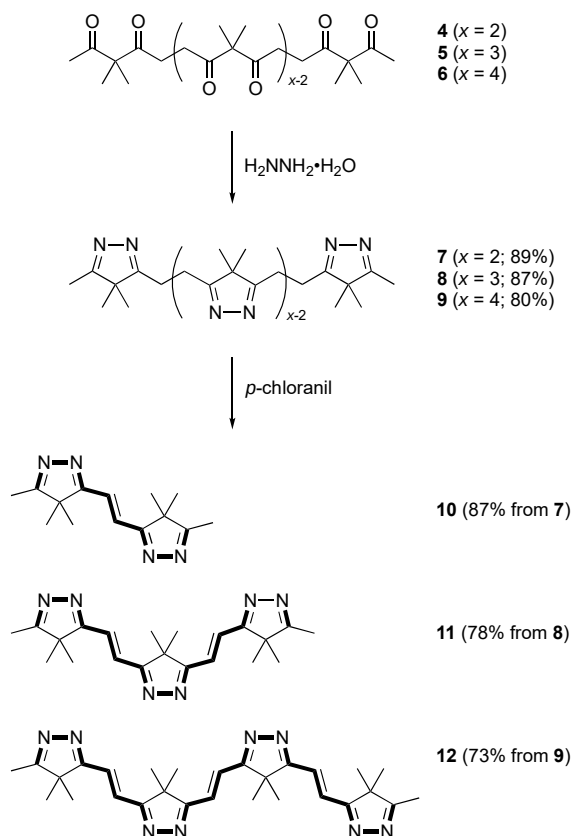
Scheme 2. Two-step transformation of oligoketones 4–6 into conjugated imines 10–12 .
