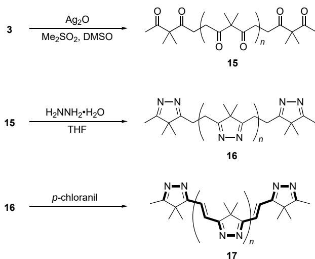
Scheme 4. Synthesis of polyketone 15 and its transformation into conjugated polyimine 17 .
