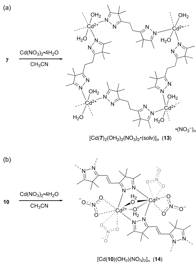
Scheme 3. Complexation of \text{Cd}(\text{NO}_3)_2 \cdot 4\text{H}_2\text{O} with (a) ligand 7 and (b) 10 .
