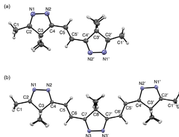
Figure 1. X-ray crystal structures of conjugated oligoimines (a) 10 and (b) 11 . Selected bond lengths (Å): N1–N2 1.4421(17), N2–C4 1.2919(18), C4–C5 1.449(2), C5–C5' 1.339(3) for 10 ; N1–N2 1.4487(18), N2–C4 1.297(2), C4–C5 1.453(2), C5–C6 1.346(2), C6–C7 1.452(2), C7–N3 1.302(2), N3–N3' 1.436(2) for 11 .
