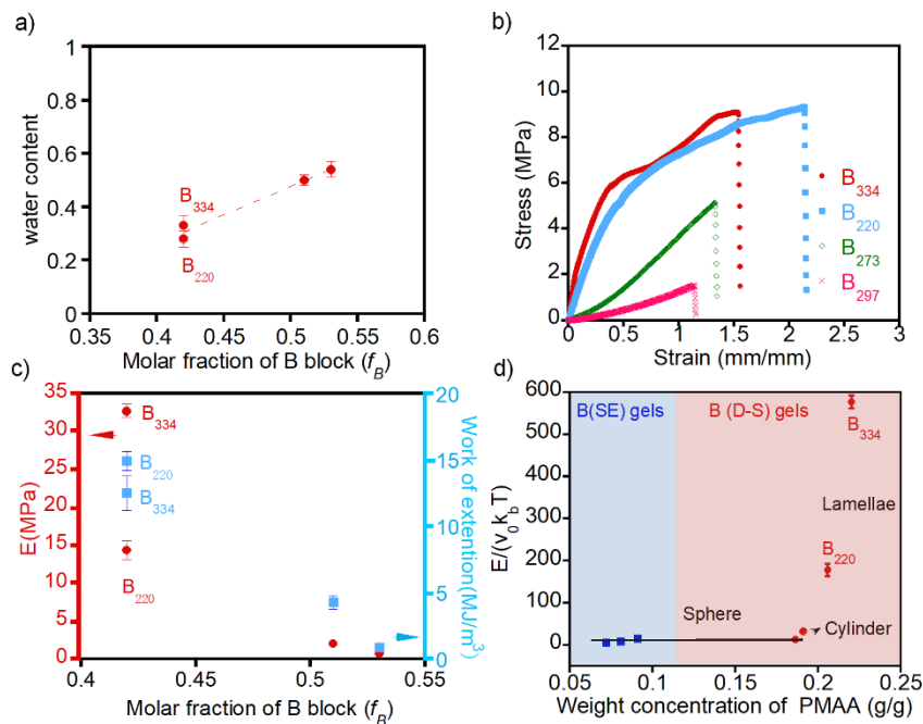
Figure 3 a) Water content of the B(D-S) gels with different molar fraction of the B block ( f_B ) in ABA block copolymers; b) Tensile stress-strain curves of different B(D-S) gels; c) the modulus ( E ) and work of extension of the B(D-S) gels plotted as a function of the molar fraction of the B block in ABA block copolymers; d) Reduced modulus, E/v_{mid}k_B T , of B(SE) gels and B(D-S) gels as a function of the weight concentration of the B-block in the gel.
