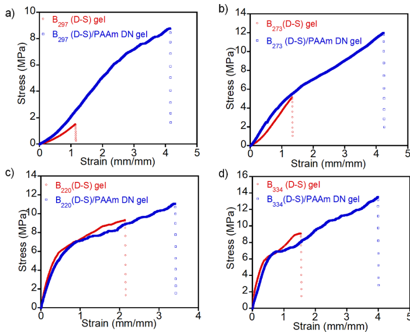
Figure 4 Tensile stress-strain curves of B(D-S)/PAAm DN gels and corresponding mother B(D-S) gels based on different PBMA- b -PMAA- b -PBMA block copolymers: a) B 297 , b) B 273 , c) B 220 , and d) B 334 .
