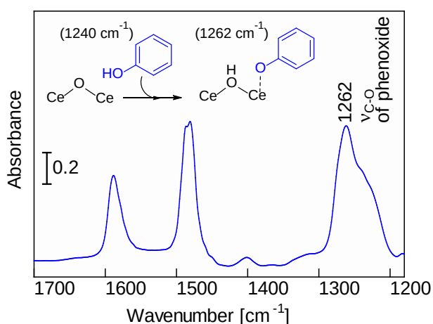
Figure 5. IR spectrum of phenoxide species on the \text{CeO}_2 surface at 120^\circ\text{C} ( t = 700 \text{ s} ). Phenol ( 1 \mu\text{L} ) was introduced to \text{CeO}_2 , followed by purging with He ( 700 \text{ s} ).
