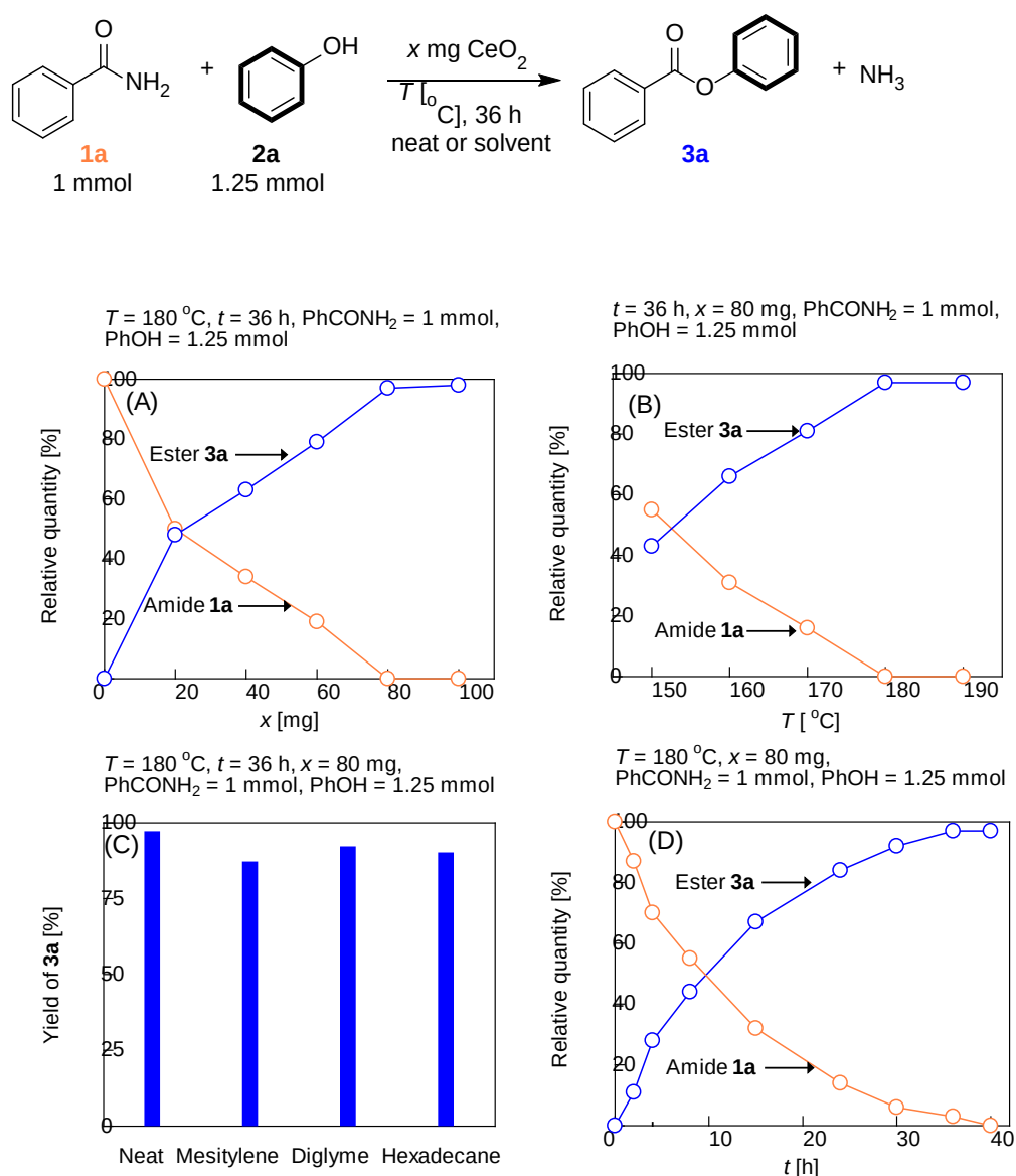
Figure 2. Optimization of the reaction conditions for the phenolysis of benzamide ( 1a ) with phenol ( 2a ) to produce phenyl benzoate ( 3a ). The relative quantities of 1a and 3a are shown as a function of the (A) amount of CeO 2 , (B) temperature, (C) solvent ( V_{\text{solvent}} = 0.5 \text{ mL} ), and (D) reaction time. The percentage yield of 3a was analyzed by GC using n -dodecane as an internal standard.
