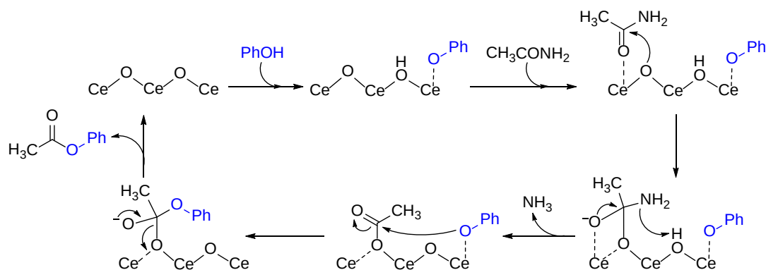
Figure 9. Plausible reaction mechanism for the CeO 2 -catalyzed phenolysis of acetamide with phenol.
