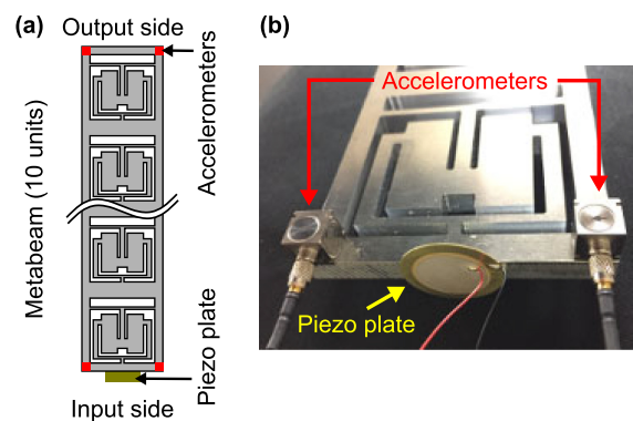
FIG. 4. Experimental setup. (a) Schematic diagram of the setup for compressional mode propagation measurements. (b) Image showing the compressional mode excitation.
