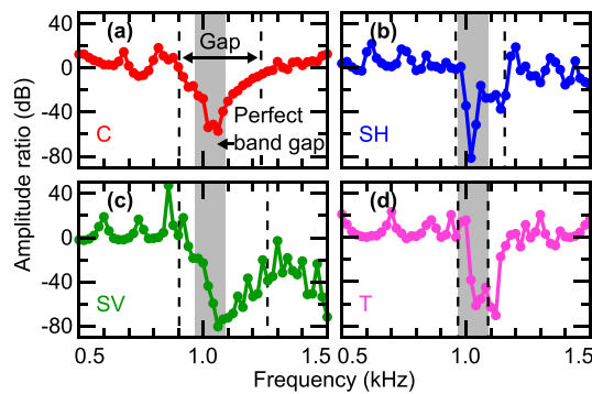
FIG. 5. Experimentally observed output/input acoustic amplitude ratio for each acoustic mode. (a)–(d) correspond to the compressional, shear-horizontal, shear-vertical (flexural), and torsional modes, respectively. The vertical dashed lines indicate the band edges for each mode expected from the simulations, whereas the gray shaded region in each case corresponds to the perfect band gap expected from the simulations.
