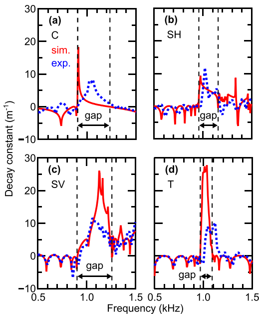
FIG. 6. Results of simulations and experiments for a metabeam of 10 unit cells. Comparison of the experimentally obtained decay constants (dotted blue lines) with those obtained from simulation (solid red lines) for the four modes. (a)–(d) show the results for the compressional (C) mode, shear horizontal (SH) mode, shear vertical (SV) mode, and torsional (T) mode, respectively. The vertical dashed lines indicate the band edges obtained from the simulated dispersion relations. sim.: simulation; exp.: experiment.
