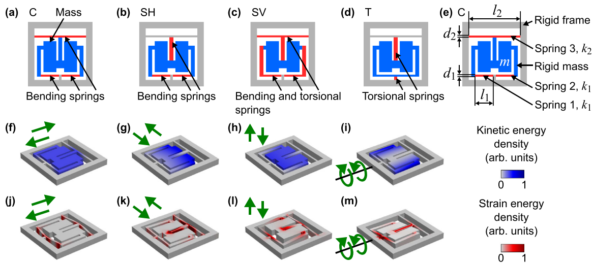
FIG. 2. Approximate analytical interpretation of the beam geometry in terms of masses and springs and simulated single-cell acoustic eigenmodes with rigid boundary conditions. (a)–(d) Geometries used for the models. The blue regions and red ribs act as masses and springs, respectively, shown for the following modes: (a) compressional (C, motion along the axial direction), (b) shear-horizontal (SH, motion along the width direction), (c) shear-vertical (SV, out-of-plane flexural motion), and (d) torsional (T, rotation about the axis along the axial direction). The gray regions are assumed to be rigid in the analytical models. (e) Detailed geometry for the compressional mode, showing the rigid inner mass m and springs 1, 2, and 3. The gray region is considered to be a rigid frame. Only in-plane motion along the axial direction is considered. (f)–(i) and (j)–(m): simulated kinetic- and strain-energy distributions for the lowest four eigenmodes, respectively. The green arrows show the displacements.
