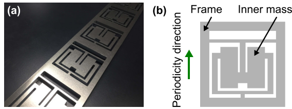
FIG. 1. Metabeam design. (a) Photograph of the metamaterial beam. (b) Schematic of the top view of the unit cell. The gray region is aluminum, and the inner white areas are holes. The unit-cell geometry comprises a frame, an inner mass, and several ribs.
