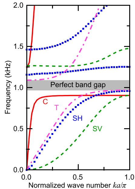
FIG. 3. Acoustic dispersion relation for axial propagation in the metabeam; k and a are the wavevector and unit-cell length, respectively. The solid red, dotted blue, dashed green, and dashed-dotted pink curves correspond to compressional (C), shear-horizontal (SH), shear-vertical (SV), and torsional (T) modes, respectively.
