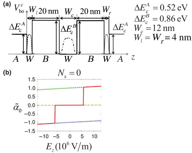
FIG. 1. (a) A triple-QW structure and the potential due to the conduction-band offset V_{\text{bo}}(z) . (b) The dependence on the applied electric field E_z perpendicular to QWs of the normalized Rashba coefficient \tilde{\alpha}_0 for an electron in the ground subband at the electron sheet density N_s = 0 . The dashed, dashed-dotted, and dotted lines represent \tilde{\alpha}_0 of A/W/B (left), B/W/B (center), and B/W/A (right) QWs, respectively, where A = \text{In}_{0.52}\text{Al}_{0.48}\text{As} , B = \text{Al}_x\text{Ga}_{1-x}\text{As}_y\text{Sb}_{1-y} ( x = 0.3 ), and W = \text{In}_{0.53}\text{Ga}_{0.47}\text{As} . In the triple-QW structure \tilde{\alpha}_0 (solid line) shows a discontinuous change when the electron makes a transfer between adjacent QWs. Here \tilde{\alpha}_0 is normalized so that \tilde{\alpha}_0 = 1 for A/W/B at E_z = 0 .
