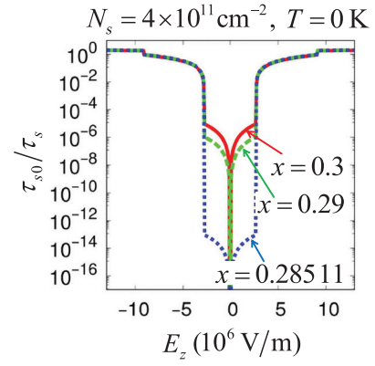
FIG. 4. Decreased spin-relaxation rate 1/\tau_s (plotted in semilogarithmic scale) as the Al fraction x in barrier material B ( \text{Al}_x\text{Ga}_{1-x}\text{As}_y\text{Sb}_{1-y} ) approaches the exact value, x_0 (\approx 0.28511) , which gives the vanishing Rashba SOI in the B/W/B single QW. Barrier material A is \text{In}_{0.52}\text{Al}_{0.48}\text{As} .
