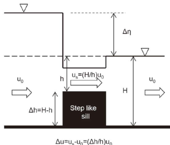
Fig. 11. One-dimensional channel model for the step like sill-topography (Iino et al., 2009). When sill-depth is h (< H; \text{channel depth}) , \Delta\eta is net sea level difference due to form drag, u_0 is velocity of passage-flow, \Delta u is the shear flow before and after sill-topography.
