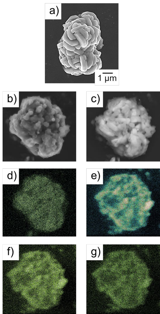
Figure 4. SEM morphology of NMC a) pristine particle and b) coated with \text{Li}_6\text{PS}_5\text{Cl} -layer from SSE-solution containing 0.1 wt% dispersant. c) Backscattering image and d)-g) EDS mapping of manganese, sulfur, phosphorus and chlorine, respectively. Weight ratio NMC: \text{Li}_6\text{PS}_5\text{Cl} of 89:9.
