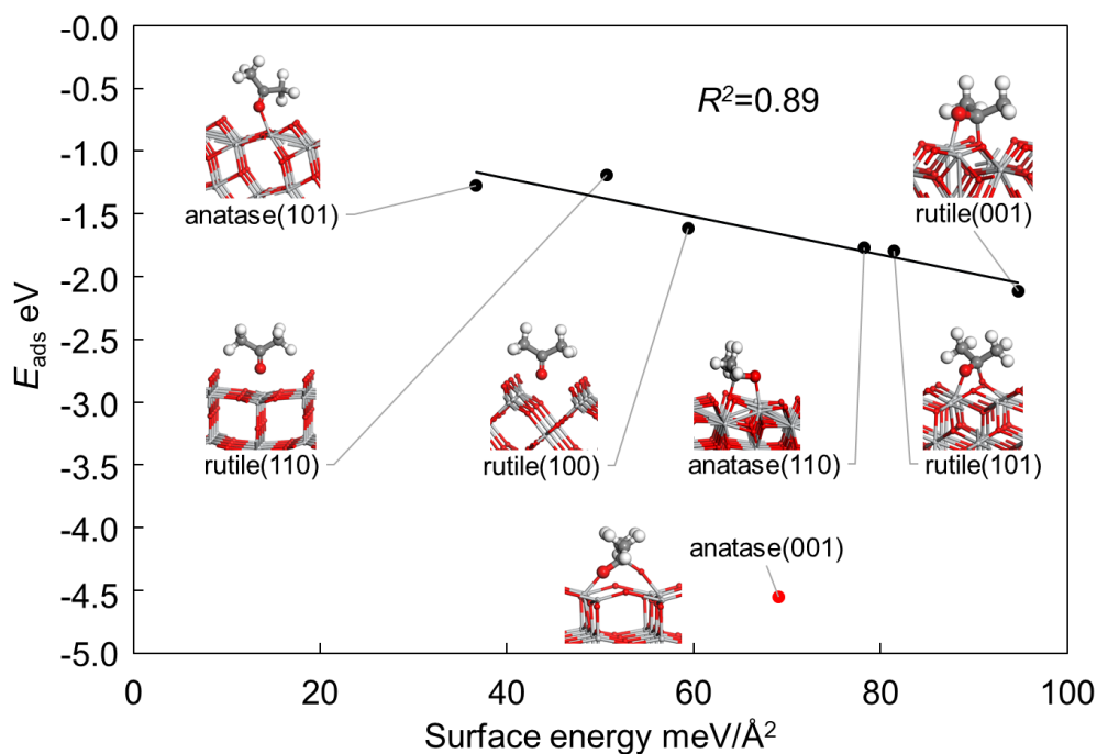
Figure 6. Adsorption energies E_{\text{ads}} for acetone as a function of surface energies of seven \text{TiO}_2 surfaces.
