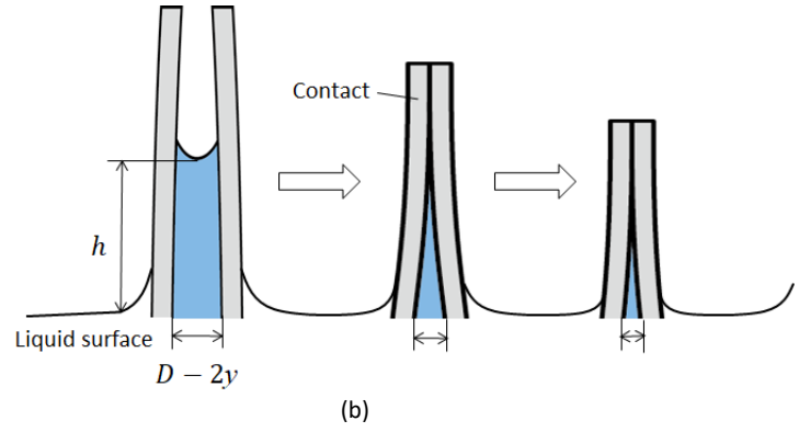
Fig. 1. Schematic diagrams showing (a) the experimental setup to observe the capillary rise between a pair of plates and (b) the measured gap between plate pairs during plate deflection and plate contact after complete coalescence.
