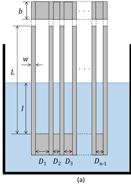
Fig. 1. Schematic diagrams showing (a) the experimental setup to observe the capillary rise between a pair of plates and (b) the measured gap between plate pairs during plate deflection and plate contact after complete coalescence.
