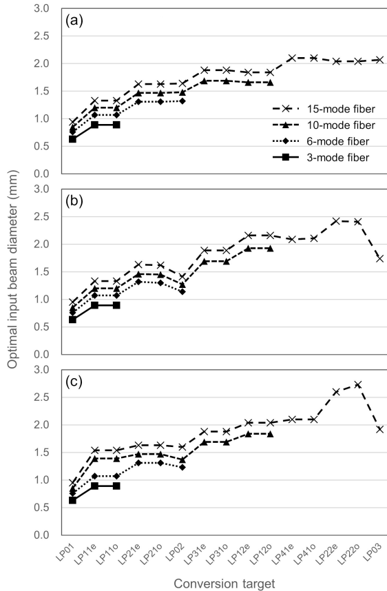
Fig. 6. Optimal input beam diameter for each fiber and each method.
