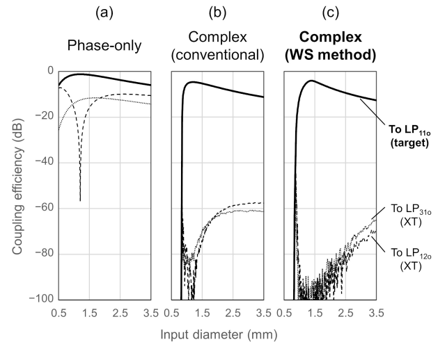
Fig. 5. Input diameter dependence for each of the methods: (a), (b), and (c). Here, values of coupling efficiency to the modes not displayed in the figure are less than -100 dB. The conversion target is \text{LP}_{110} of a 10-mode fiber.
