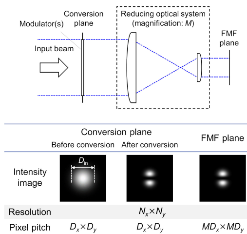
Fig. 4. Simulation model and intensity images on each plane. The spatial distribution of light on the FMF plane was obtained by redefining the pixel pitch of the image as a reduced one with the magnification of the optical system.
