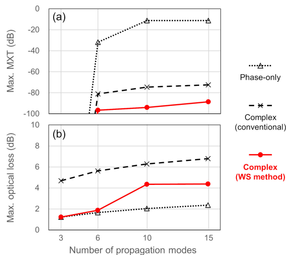
Fig. 8. Maximum value of (a) MXT and (b) optical loss occurring during conversion (for each fiber and each method). In all the methods, an MXT much lower than -100 dB is obtained for the 3-mode fiber.
