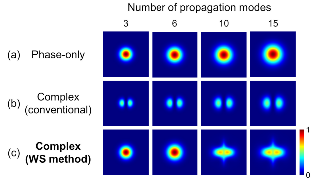
Fig. 7. Intensity distribution of the output beam modulated by each method. Each image is normalized by the peak value of input intensity. The conversion target is LP_{11o} for each fiber.
