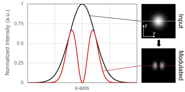
Fig. 1. Relationship between an input and output intensity profile obtained by intensity modulation in the mode conversion from a fundamental mode to LP 11o .
