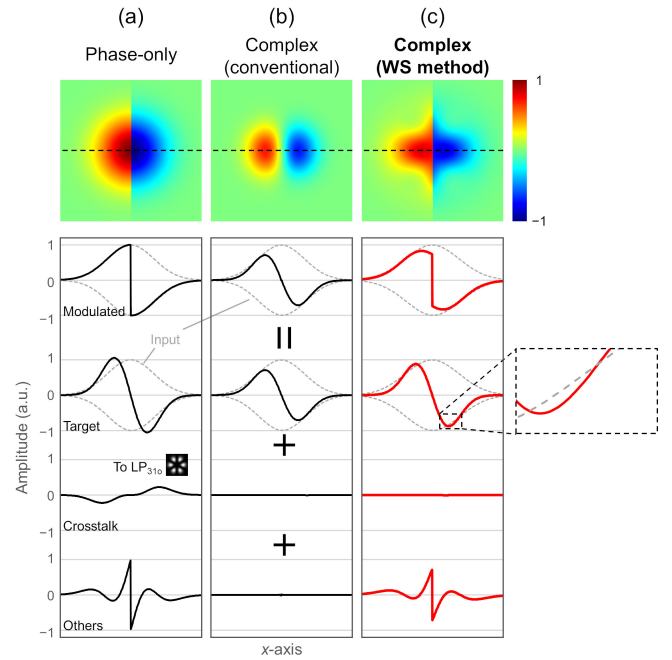
Fig. 3. Images of the real part of the complex amplitude distribution and the cross-sectional profiles of the converted beam and its components such as target, crosstalk, and others for the three methods: (a), (b), and (c). The conversion target for the 10-mode fiber is LP_{11o} . The gray dotted lines in the modulated and target profiles represent the input amplitude. The crosstalk component in (a) mainly excites LP_{31o} . The enlarged view of the target component in (c) shows that the output by the WS method contains partially higher amplitude than the input.
