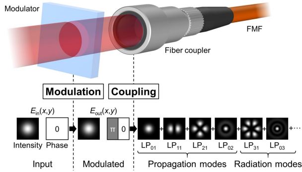
Fig. 2. Conceptual diagram of mode excitation in an FMF. The conversion method is based on phase-only modulation and the conversion target is LP_{11e} .
