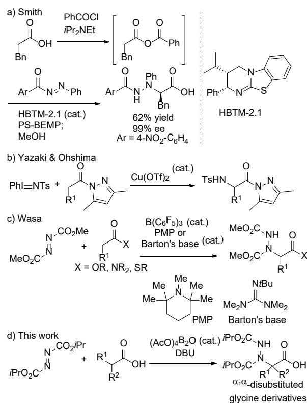
Scheme 1. Catalytic \alpha -Amination of Carboxylic Acid Derivatives.
