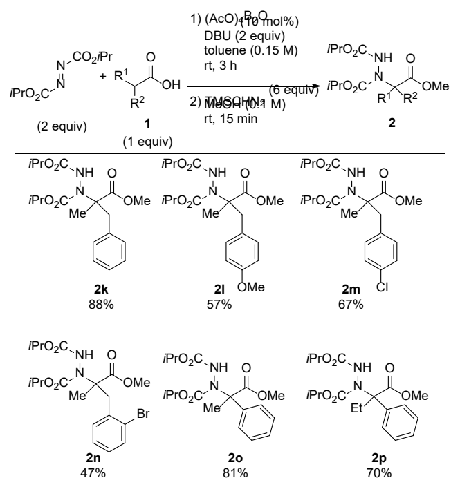
Scheme 3. Substrate Scope for \alpha,\alpha -Disubstituted Acetic Acids. a
