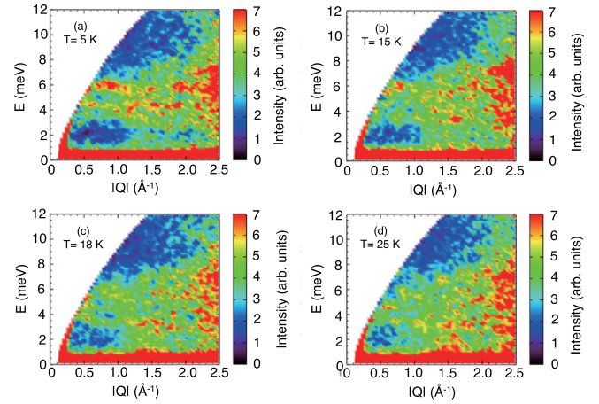
FIG. 6. Color contour maps of the inelastic neutron scattering intensity S(|Q|, E) for \text{Ag}_2\text{CoO}_2 powder measured with E_i = 15 \text{ meV} at T = 5 \text{ (a)} , 15 \text{ (b)} , 18 \text{ (c)} , and 25 \text{ K (d)} .
