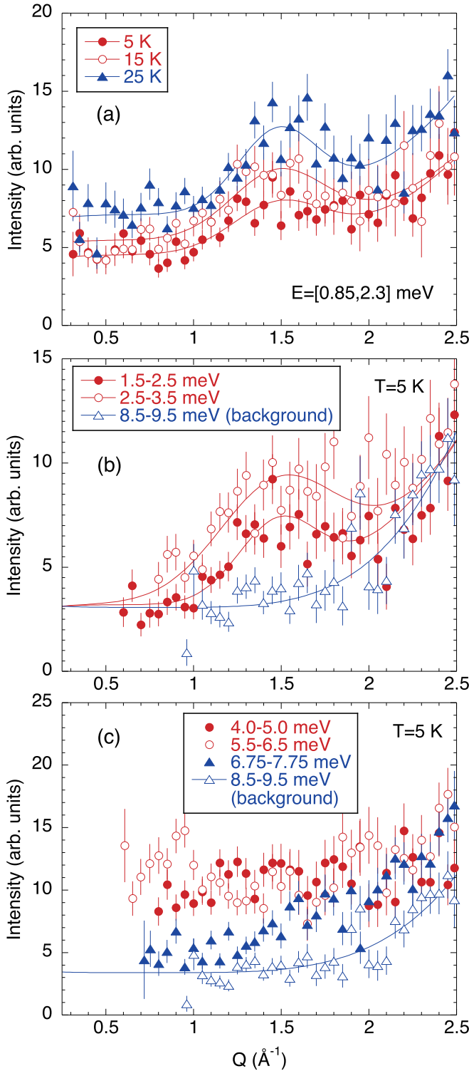
FIG. 7. (a) Q cuts of S(|Q|, E) integrated with respect of energy in the range of E = 0.85-2.3 meV measured with E_i = 15 meV at T = 5, 15 , and 25 K. (b) Q cuts of S(|Q|, E) integrated with respect of energy in the range of E = 1.5-2.5 meV and 2.5-3.5 meV (b) and 4.0-5.0 meV, 5.5-6.5 meV, and 6.75-7.75 meV (c) measured with E_i = 15 meV at T = 5 K. The scattering intensity averaged in the energy range between 8.5 and 9.5 meV can be regarded as a background. The solid lines are guides to the eye.
