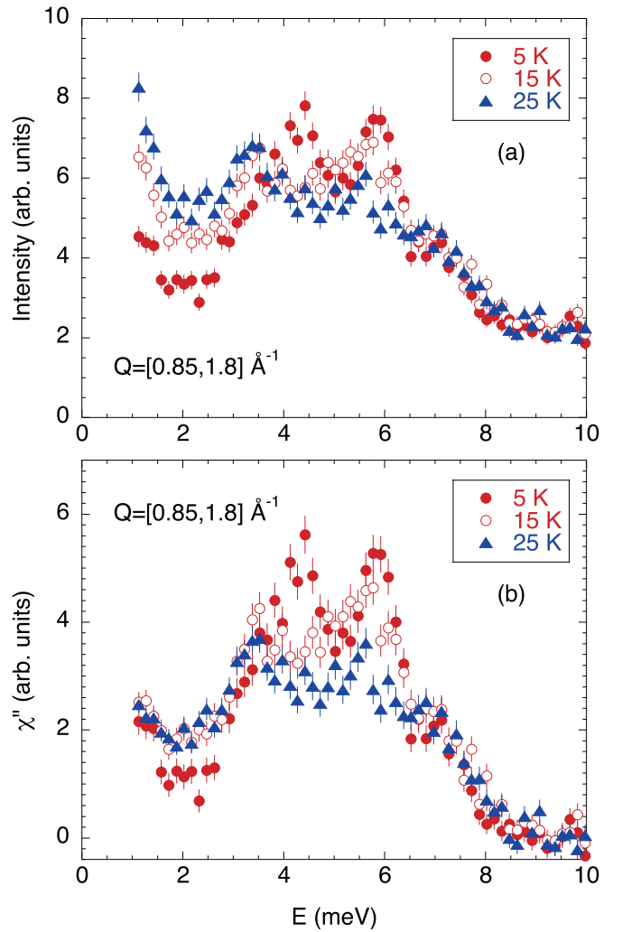
FIG. 8. (a) Energy cuts of S(|Q|, E) integrated with respect of |Q| in the range of |Q| = 0.85-1.8 \text{\AA}^{-1} at T = 5, 15 , and 25 K. (b) Energy cuts of \chi''(E) converted from the Q integrated S(|Q|, E) . The constant background intensity estimated in the energy range between 8.5 and 10 meV was subtracted before the conversion.
