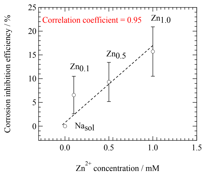
Fig. 6.13 Corrosion inhibition efficiency in the solutions with different concentrations of \text{Zn}^{2+} .
