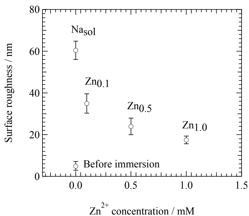
Fig. 6.5 Surface roughness of specimens versus \text{Zn}^{2+} concentration before and after immersion in the solutions for 3 d at 25°C.
