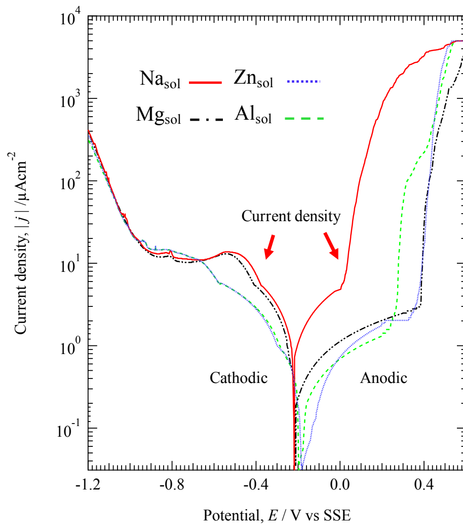
Fig. 3.10 Polarization curves of specimen immersed in the different solutions with metal cations.
