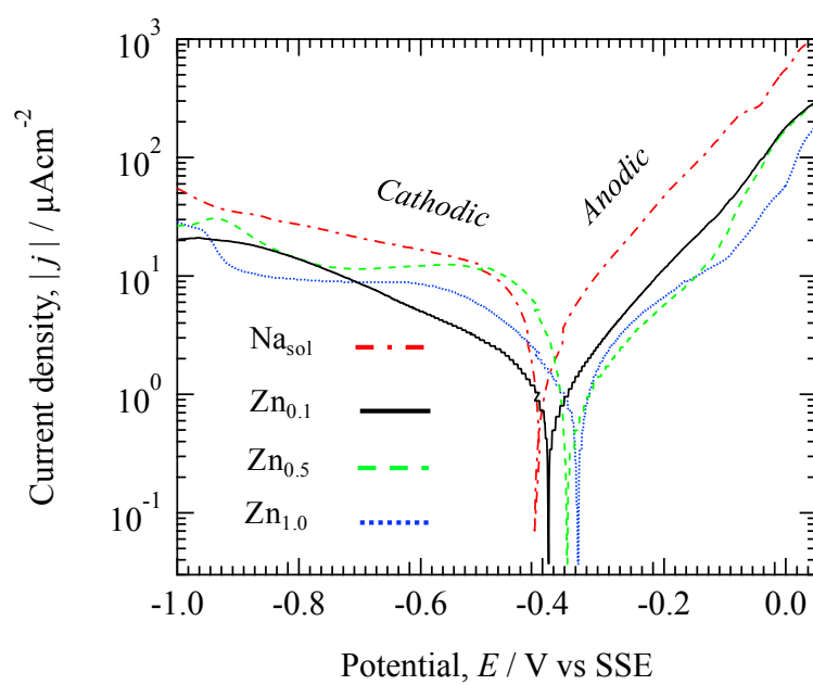
Fig. 6.10 Potentiodynamic a) cathodic and b) anodic polarization curves after immersion in the solutions for 1 h at room temperature.
