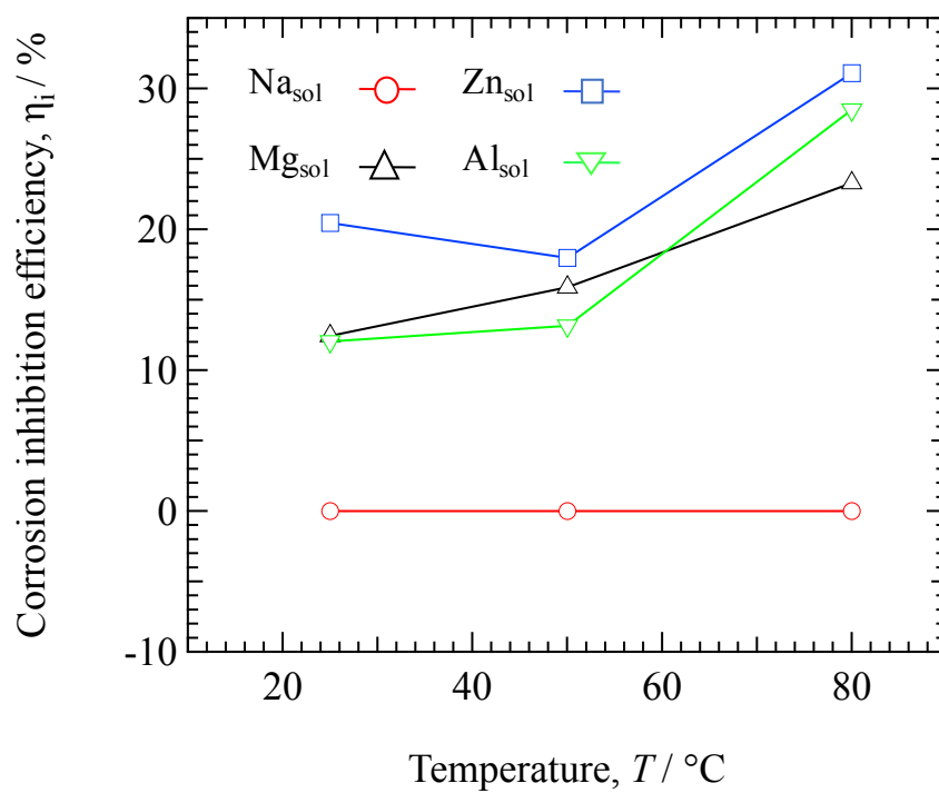
Fig. 5.13 Corrosion inhibition efficiency of metal cations as a function of temperature.
