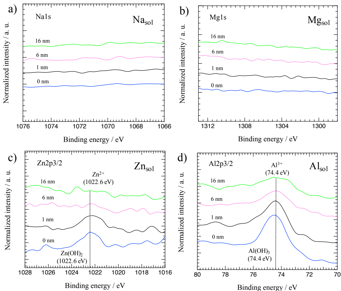
Fig. 3.6 XPS narrow spectra of metal cations with depth a) Na 1s peaks of specimen immersed in \text{Na}_{\text{sol}} , b) Mg 1s peaks of specimen immersed in \text{Mg}_{\text{sol}} , c) Zn 2p 3/2 peaks of specimen immersed in \text{Zn}_{\text{sol}} , d) Al 2p 3/2 peaks of specimen immersed in \text{Al}_{\text{sol}} .
