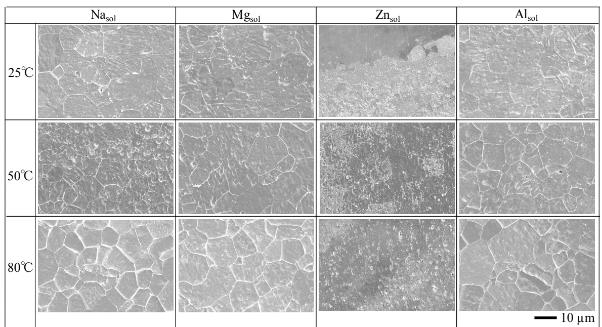
Fig. 5.5 Surface SEM images of specimen after immersion in the solutions for 3 d at 25, 50 and 80°C.
