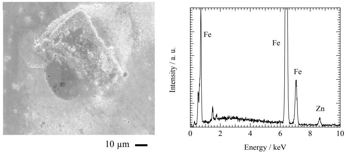
Fig. 2.10 SEM image of analysis area (left) and EDS results (right) of the specimen surface after immersion in the \text{Zn}_{\text{sol}} .
