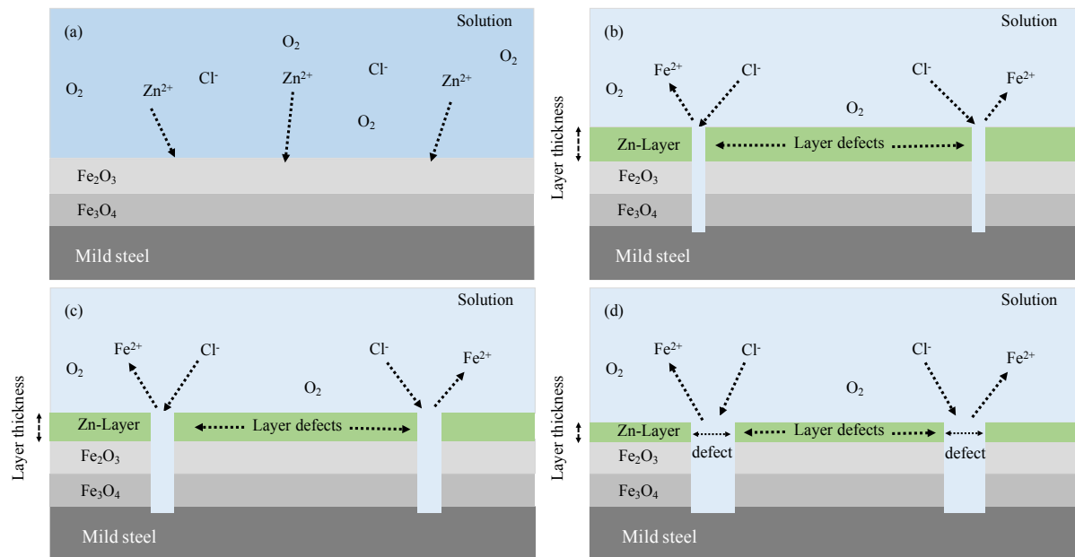
Fig. 5.14 Corrosion inhibition mechanism of mild steel by the Zn-layer at different temperatures, a) Formation of Zn-layer on the steel surface, b) \text{Cl}^- attack at the defect sites and initiation of metal dissolution at 25^\circ\text{C} , c) decreasing of Zn-layer thickness and increasing of defect area at 50^\circ\text{C} , d) decreasing of Zn-layer thickness and increasing of defect area at 80^\circ\text{C} .
