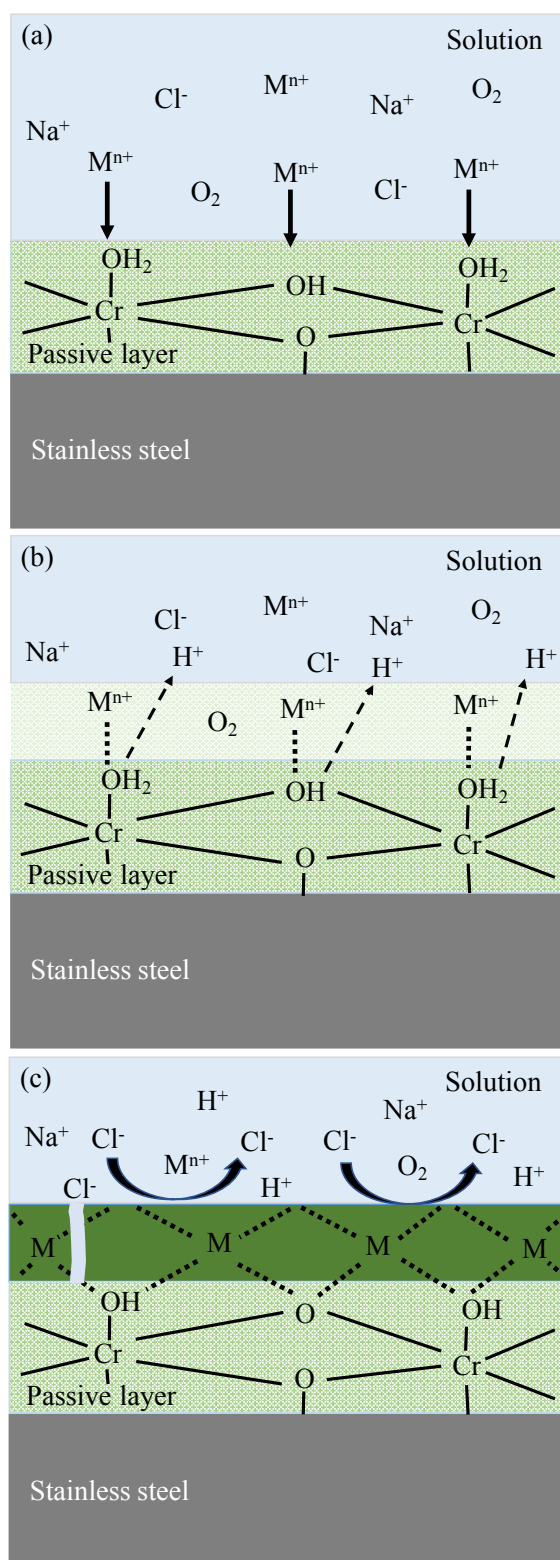
Fig. 3.13 (a) Schematic representation of the passive films structure with hard metal cations in 0.5 M Cl^- aqueous solution ( M^{n+} = Zn^{2+}, Al^{3+} ). (b) deprotonation process accelerated by hard metal cations, M^{n+} . (c) formation of metal cation layer on the passive films by hard metal cations.
