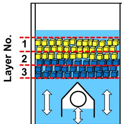
Figure 4-2. A schematic illustration of a desktop-type batch-wise RETAC jig and how the products were partitioned into 3 layers.
