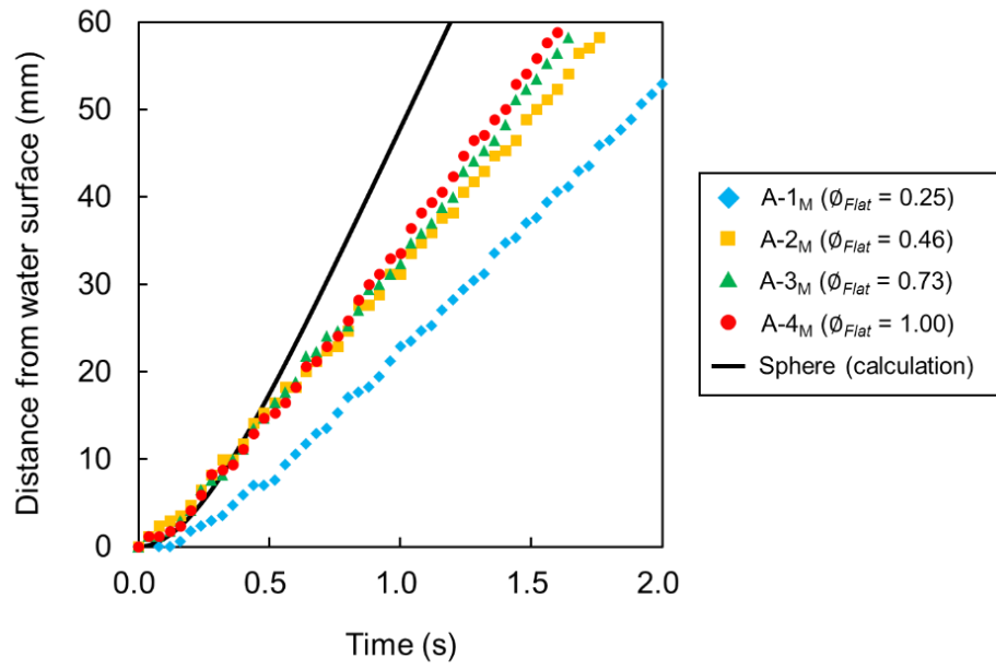
Figure 4-5. Settling distance of cut particles having equivalent volume from water surface by time.
