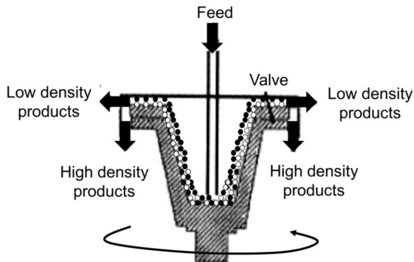
Figure 2-13. A schematic diagram of a Falcon concentrator
