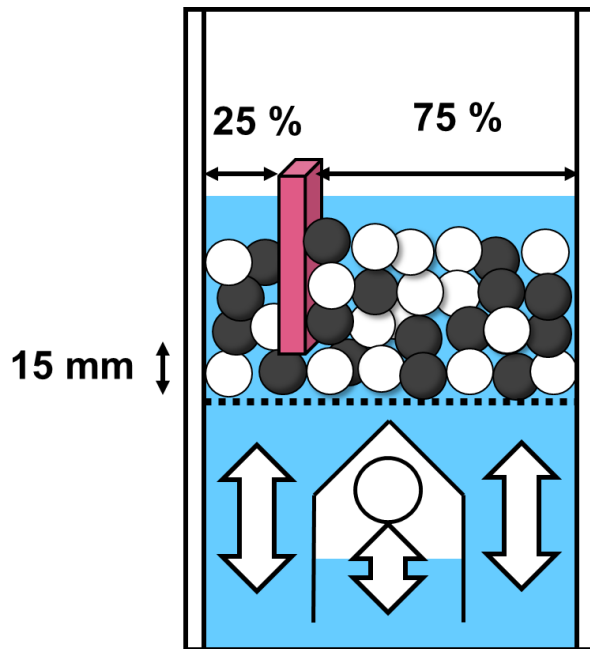
Figure 6-3. Schematic diagrams of a batch-type jig with a vertical restraining wall.
