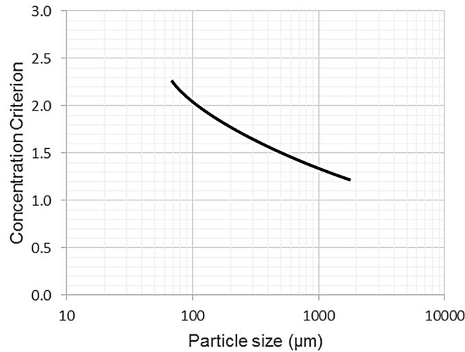
Figure 2-6. The graph shows the limit size curve of gravity separation from concentration criterion (CC) (Gupta and Yan, 2006).
