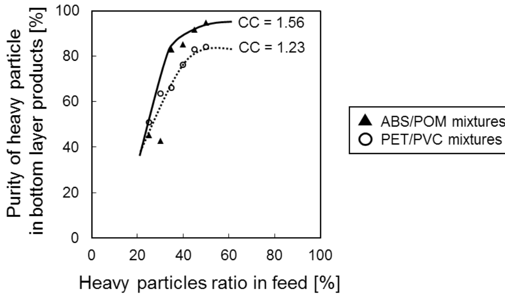
Figure 6-7. Separation curves of ABS/POM (CC of 1.56) and PET/PVC (CC of 1.23)
