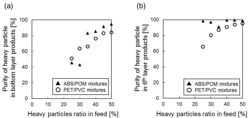
Figure 6-6. Relation between the heavy particles ratio in feed and (a) purity of heavy particles in bottom products from continuous-type jig test and (b) purity of heavy particles in 6 th layer products from batch-type jig test
