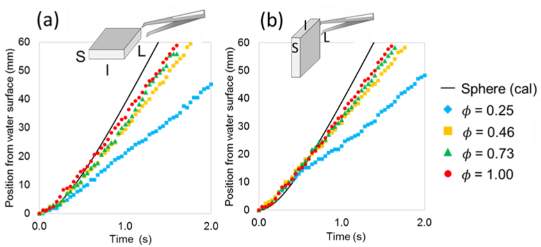
Figure 4-4. Settling distance of model plastic particles having equivalent volume from water surface by time at different initial orientations; (a) projection area ( A ) was parallel to the water surface (Fig. 4-3(b-1)) and (b) projection area ( A ) was perpendicular to the water surface (Fig. 4-3(b-2)).
