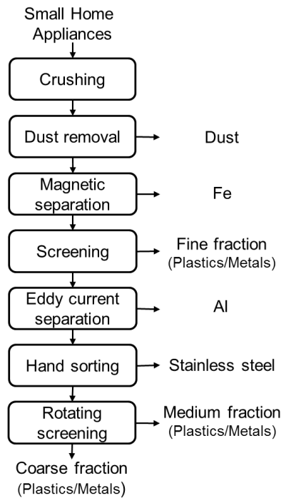
Figure 5-1. The treatment flowchart for discarded small home appliances of a recycling plant in Japan.
