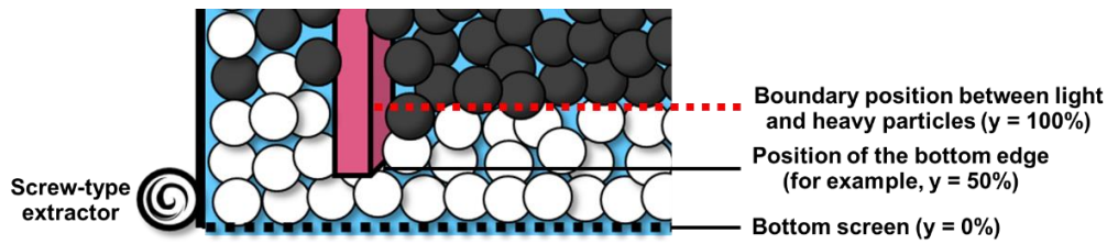
Figure 6-2. Wall position with the relation of boundary position between light and heavy particles.
