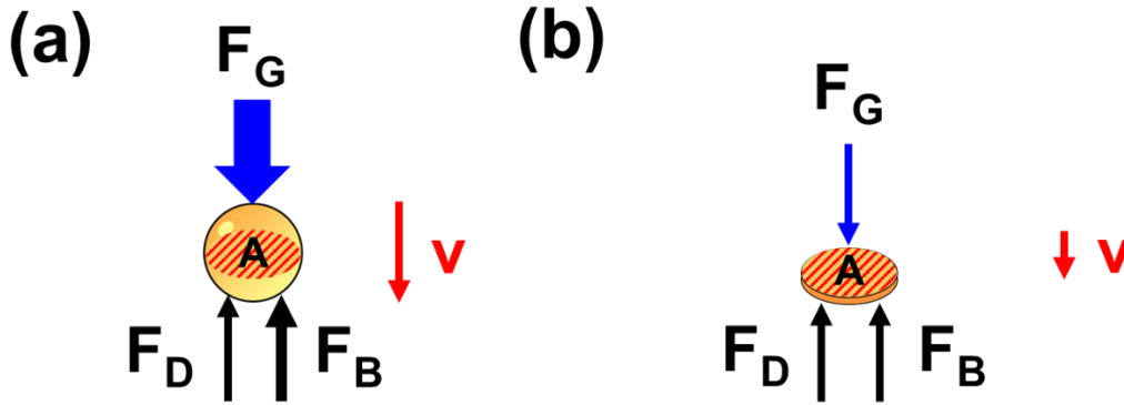
Figure 3-13. Schematic diagrams of the balances of forces acting on particles with the same projection area ( A ) and equivalent projection area diameter ( D_a ) but different shapes: (a) sphere-like, and (b) disk-like.
