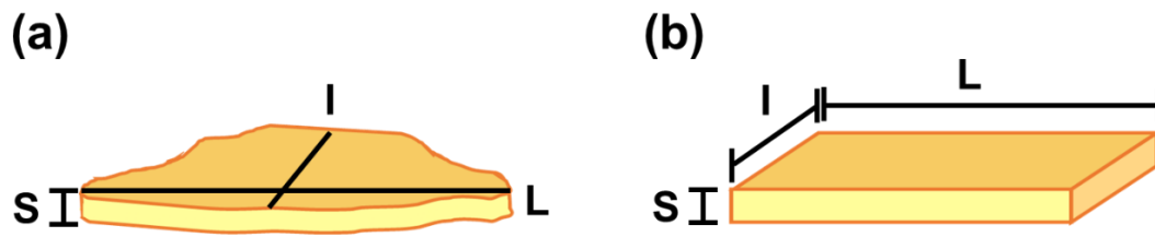
Figure 4-1. A schematic diagram showing the short ( S ), intermediate ( I ) and long ( L ) axes of plastic particles; (a) crushed plastic sample and (b) model plastic sample.
