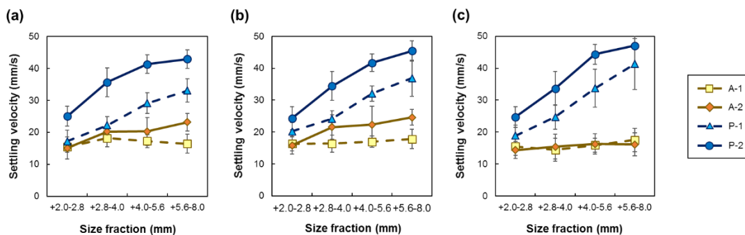
Figure 3-9. Average settling velocities of samples at different size fractions with initial orientation: (a) Fig. 3-3a, (b) Fig. 3-3b and (c) Fig. 3-3c.
