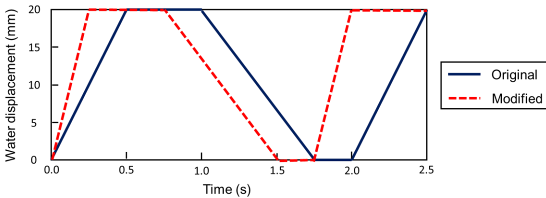
Figure 4-12. Waveform of RETAC jig separation.
