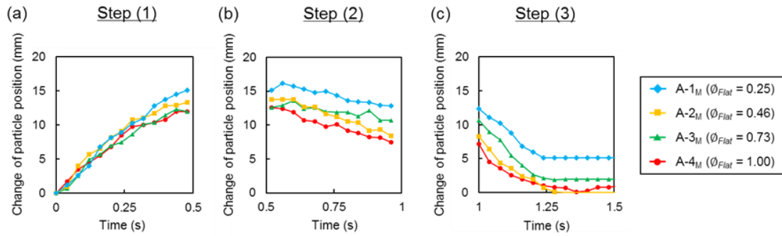
Figure 4-11. Particle position change with time from initial position of (a) step 1, (b) step 2, (c) step 3. Note : step (4), the particles have already reached the bottom surface so, no motion was occurred.
