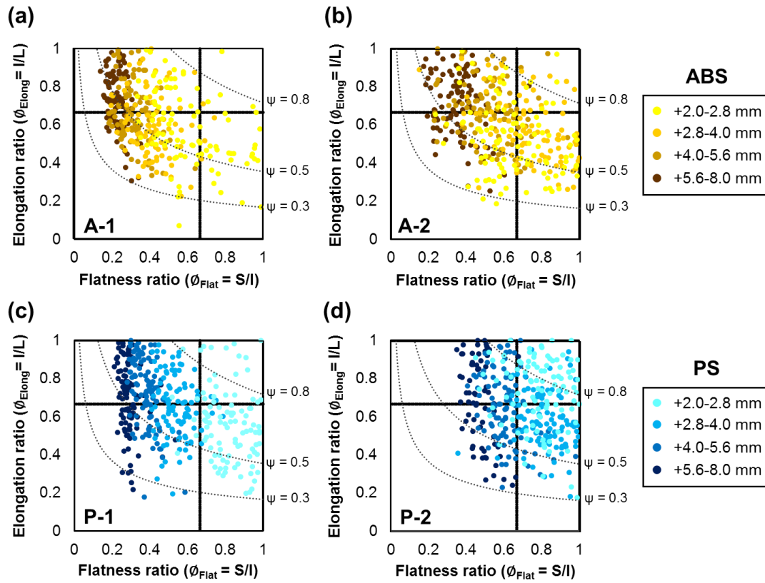
Figure 3-5. Zingg diagrams showing the particle shape distribution and operational sphericity of samples (a) A-1, (b) A-2, (c) P-1, and (d) P-2.
