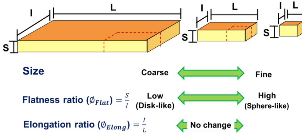
Figure 3-7. A schematic diagram of particle shape changes during crushing.
