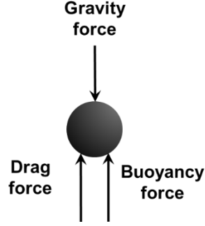
Figure 2-3. Force balance of the gravitational, buoyancy, and drag forces on a settling particle.
