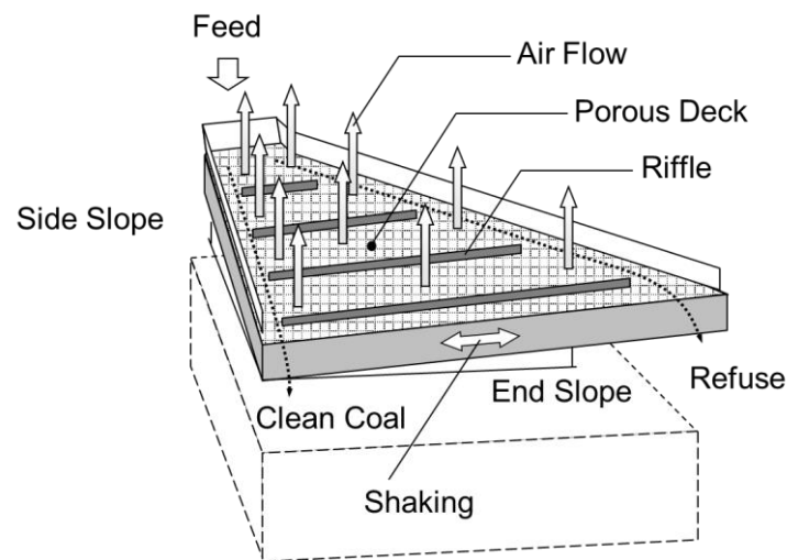
Figure 2-10. A schematic diagram of an air table.
