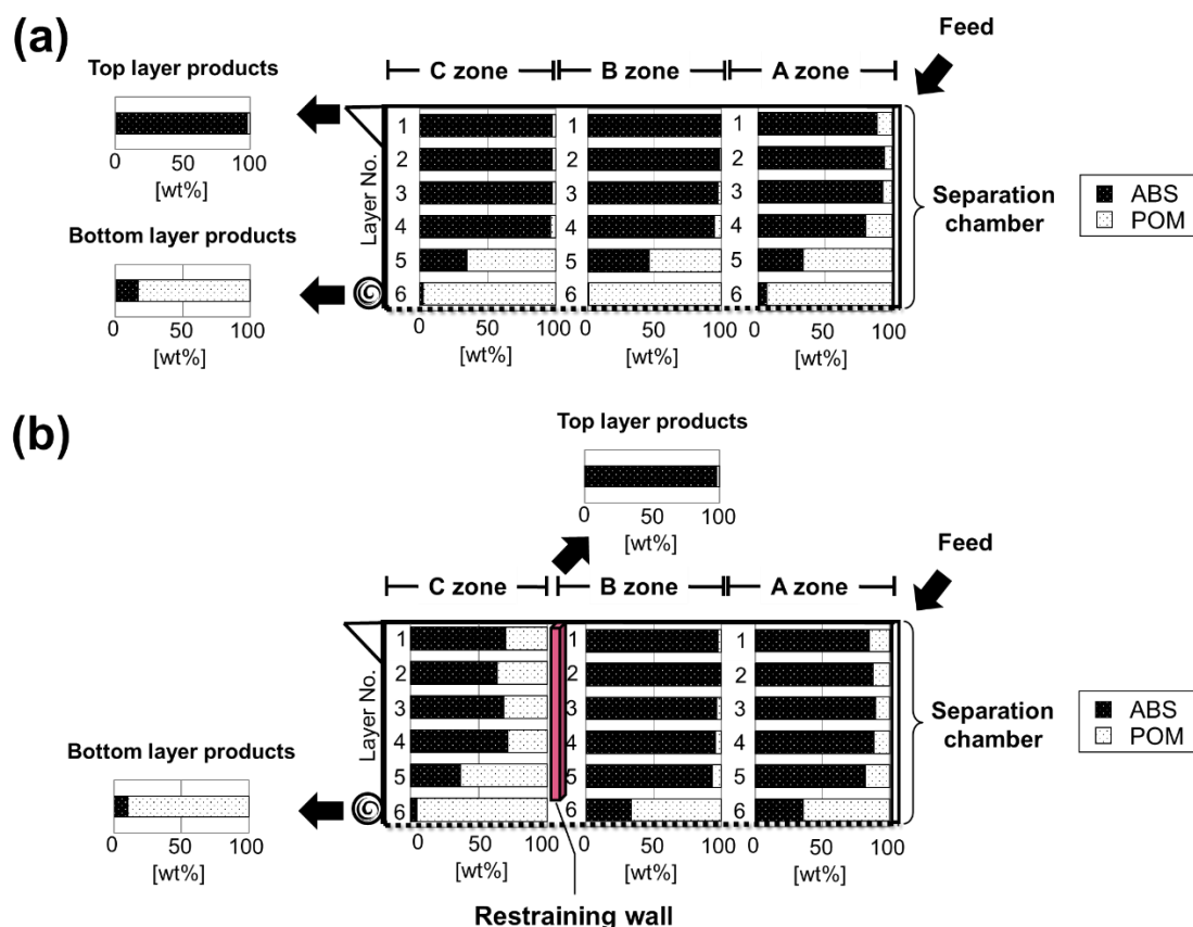
Figure 6-4. Distributions of ABS and POM in in top and bottom layer products, and particles remained in each zone and layer after the equilibrium state of continuous-type jig experiments (a) without, and (b) with a vertical restraining wall.
