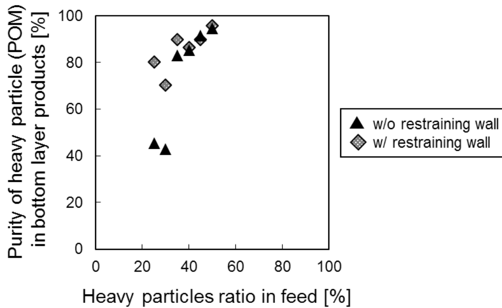
Figure 6-8. Relation between the heavy particle ratio in feed and purity of heavy particles purity of heavy particles in bottom products from continuous-type jig experiments of ABS/POM mixtures with and without restraining wall.
