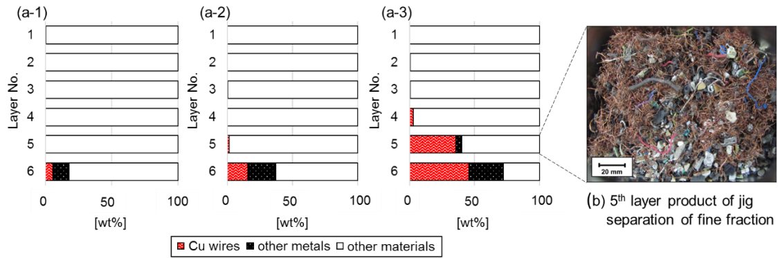
Figure 5-3. (a) The proportion of Cu wires, other metals, and other materials in each layer with the jig separation of real samples at different size fraction; (a-1) coarse, (a-2) medium, (a-3) fine and (b) 5 th layer product of jig separation of the fine fraction.
