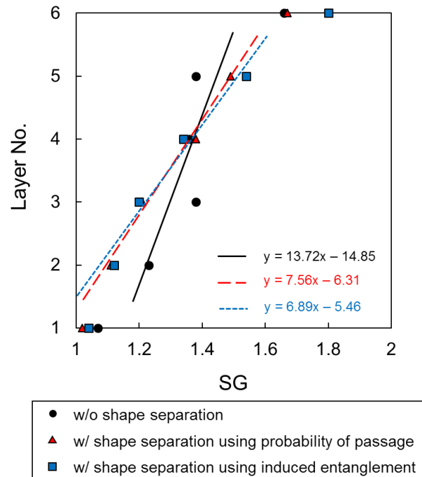
Figure 5-7. Specific gravity of other materials fractions (e.g. plastics, glasses, woods and papers) of products in each layer after jig separation.
