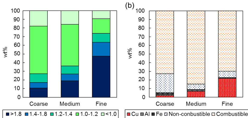
Figure 5-2. (a) Specific gravity distribution, and (b) material compositions of coarse, medium, and fine fractions.
