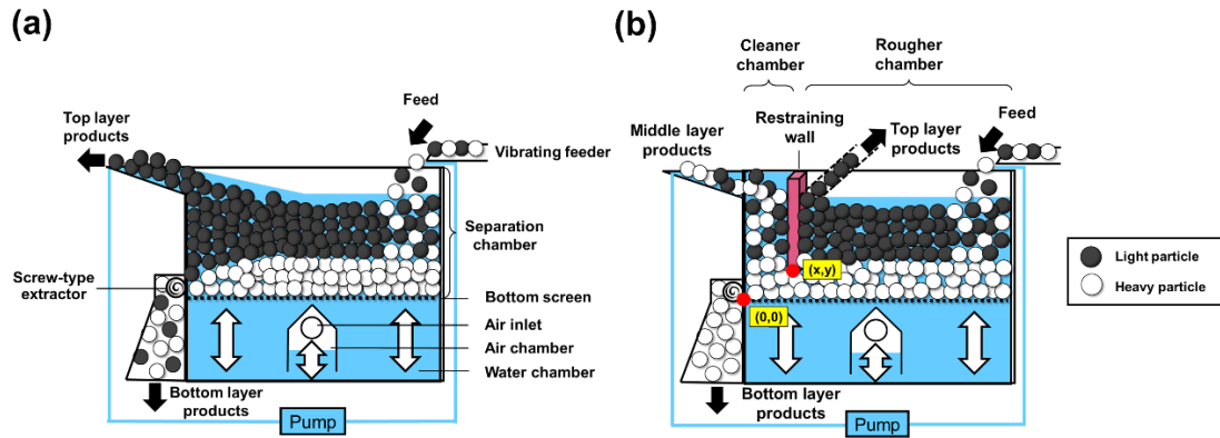
Figure 6-1. Schematic diagrams of a continuous-type jig (a) without, and (b) with a vertical restraining wall.
