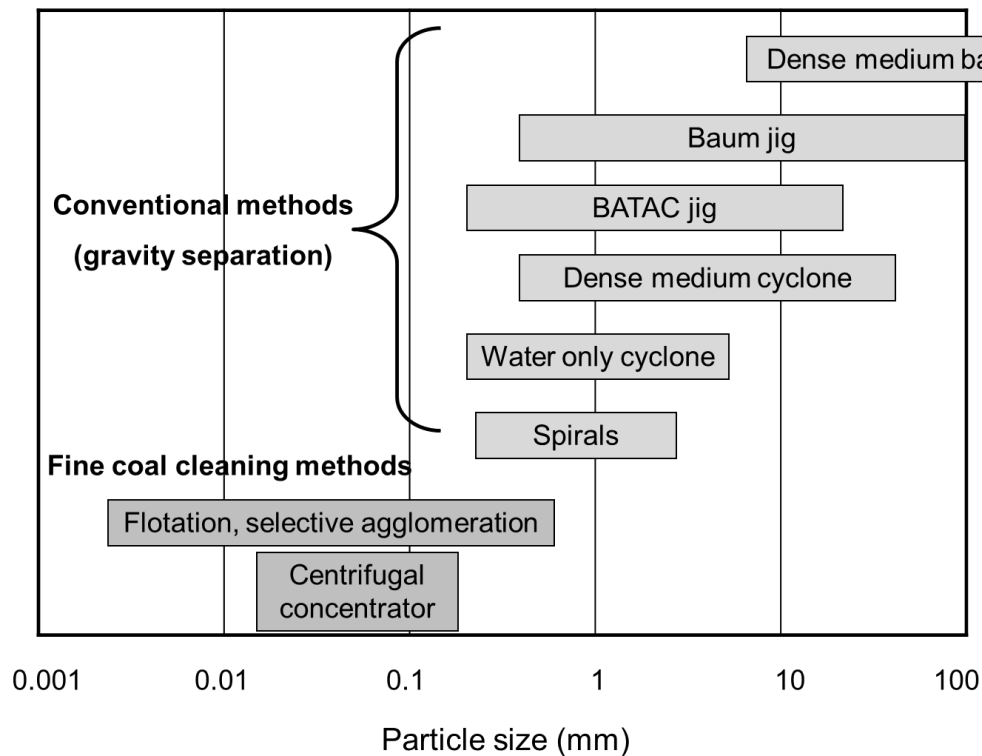
Figure 2-8. Particle size dependence of coal cleaning methods (Ito, 2008).
