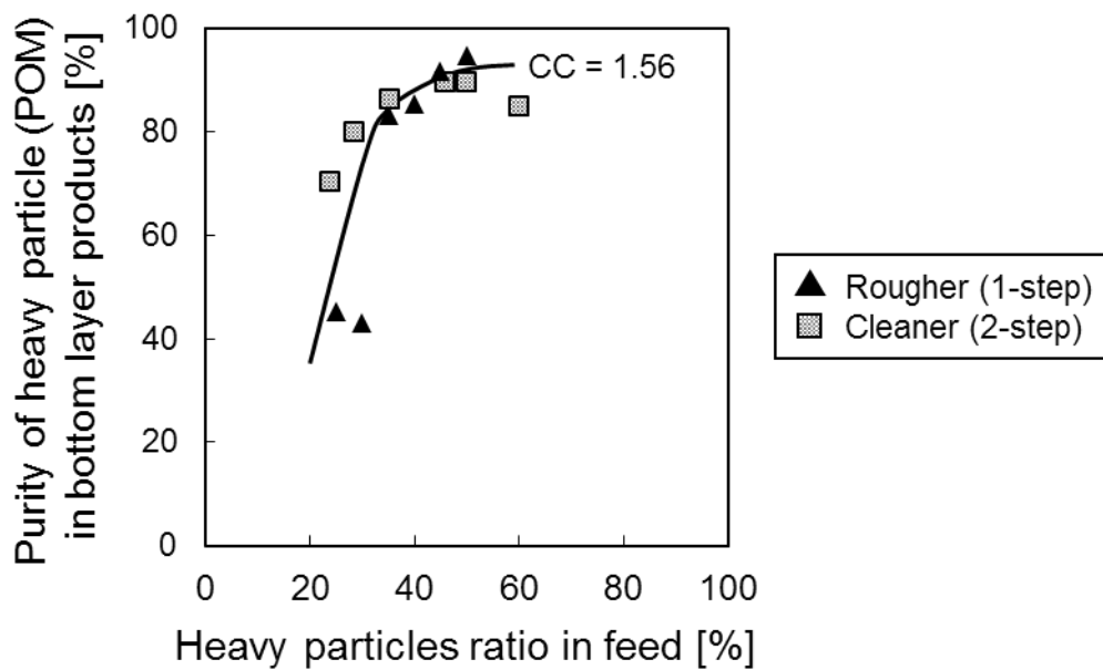
Figure 6-9. Relation between the ratio of POM in the cleaner chamber (C zone) and purity of POM in bottom layer products recovered by a screw-type extractor of continuous-type jig test with restraining wall fitted with the separation curve of ABS/POM (CC of 1.56) in Fig. 6-7.
