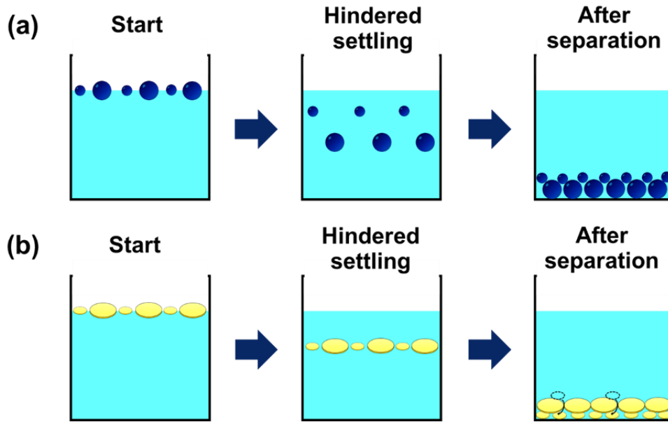
Figure. 3-15. Schematic diagrams of size segregation during jig separation of (a) sphere-like particles (i.e., P-2), and (b) disk-like particles (i.e., A-1).
