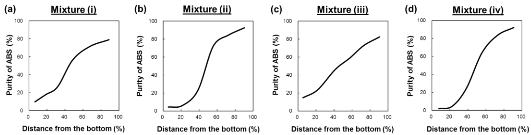
Figure 3-17. Partial separation efficiency curves after jig separation of (a) mixture (i) (A-1 and P-1), (b) mixture (ii) (A-1 and P-2), (c) mixture (iii) (A-2 and P-1) and (d) mixture (iv) (A-2 and P-2).
