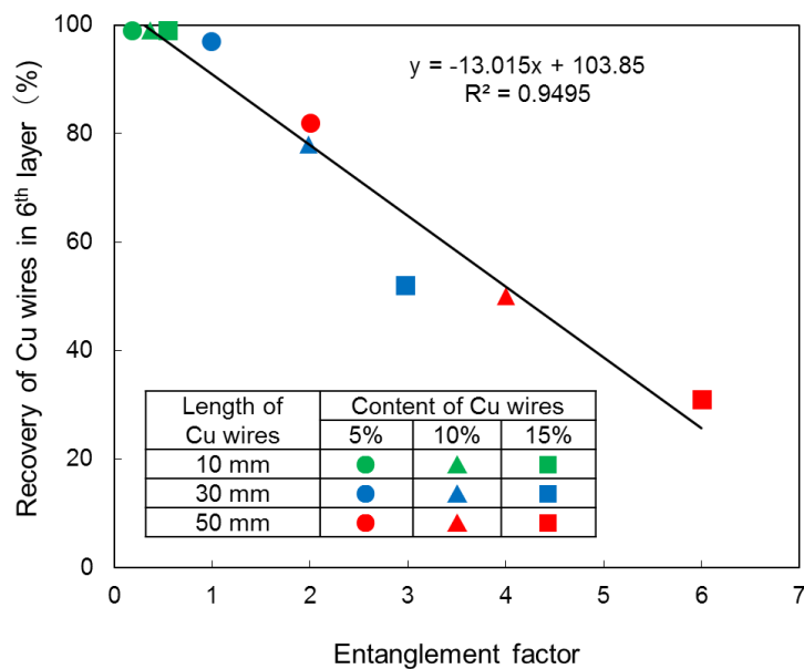
Figure 5-11. Relationship between entanglement factor and recovery of Cu wires in 6 th layer of model samples.
