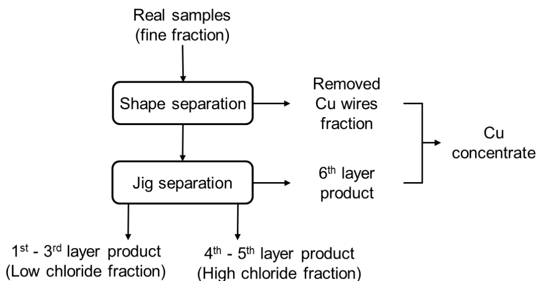
Figure 5-8. Proposed treatment flowchart including shape separation for plastic-dominated residues with Cu wires.
