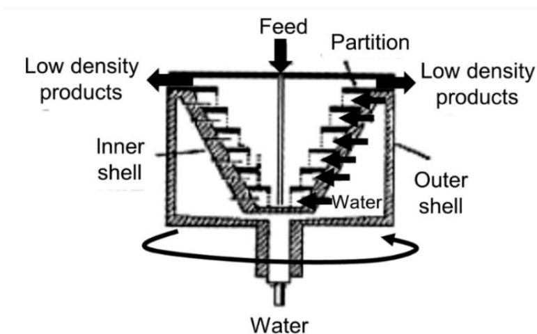
Figure 2-12. A schematic diagram of a Knelson concentrator.
