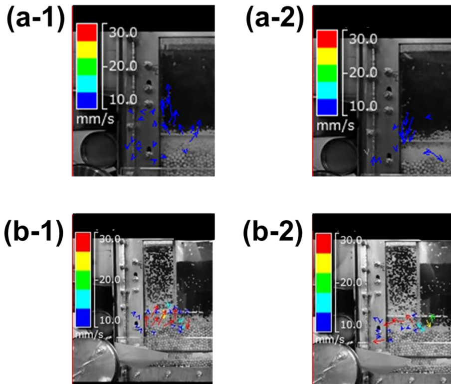
Figure 6-10. Particle flow velocities during continuous-type separations without a vertical restraining wall: (a-1) upward flow period, and (a-2) downward flow period, and with a vertical restraining wall: (b-1) upward flow period, and (b-2) downward flow period.
