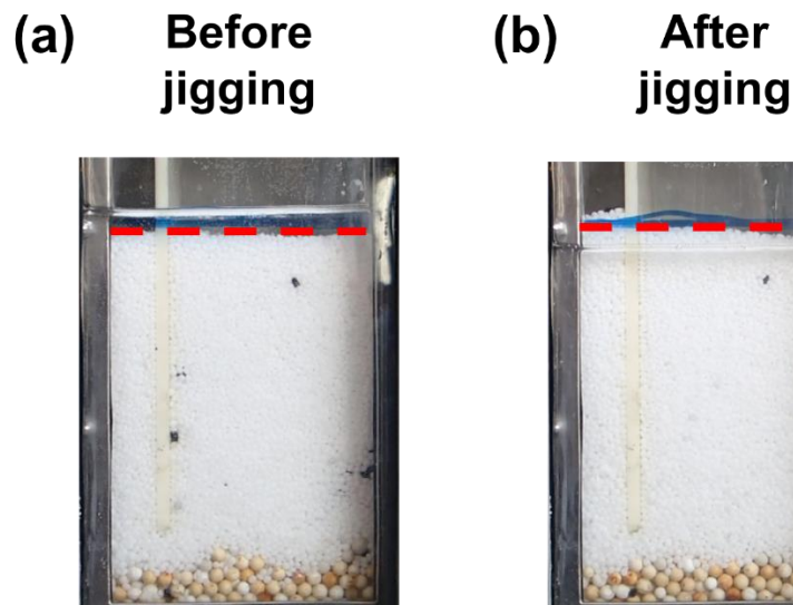
Figure 6-13. Photographs of batch-type jig experiment of POM with a vertical restraining wall; (a) before and (b) after jigging.
