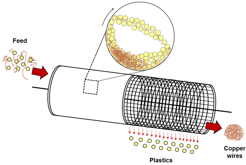
Figure 5-9. A schematic diagram of a modified rotating screen.
