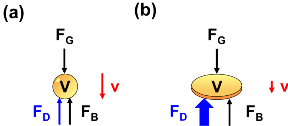
Figure 3-11. Schematic diagrams of the balances of forces acting on particles with the same volume ( V ) but different shapes: (a) sphere-like, and (b) disk-like.
