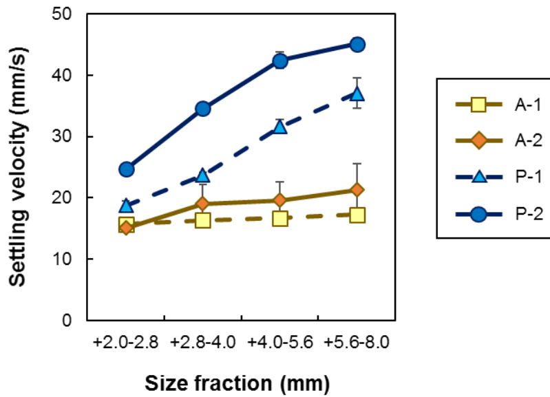
Figure 3-10. Average settling velocities of random particles from different size fractions.
