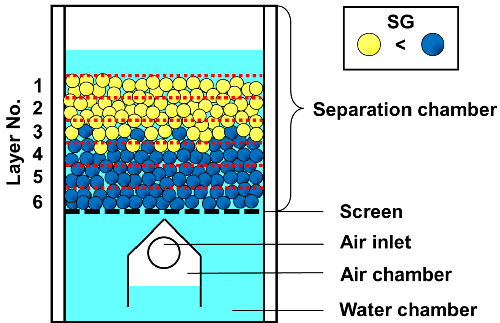
Figure 3-2. A schematic illustration of a desktop-type batch-wise RETAC jig and how the products were partitioned into 6 layers.
