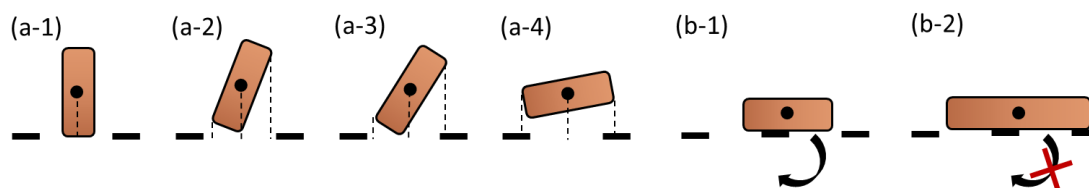
Figure 5-5. A schematic diagram of probability of passage of rod-like particle (a) particle orientations during screening; (a-1, a-2, and a-3) can pass through screen and (a-4) cannot and (b) rolling during screening; (b-1) can turn over and pass through screen and (b-2) cannot (Beunder, 2000; Beunder and Rem, 1999).
