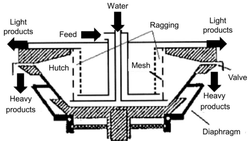
Figure 2-11. A schematic diagram of a Kelsey jig.
