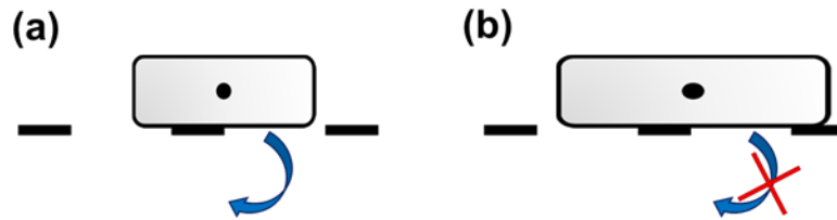
Figure 2-5. (a) Particles with a length less than or equal to twice the mesh size may turn over the edge of the mesh, whereas (b) longer particles cannot (Beunder and Rem, 1999).
