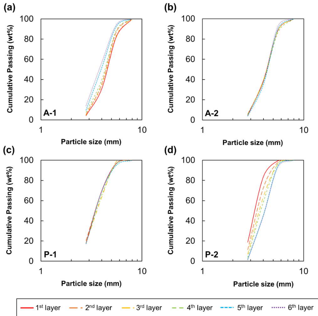
Figure. 3-14. Size distribution of each layer after jig separation of (a) A-1, (b) A-2, (c) P-1, and (d) P-2.
