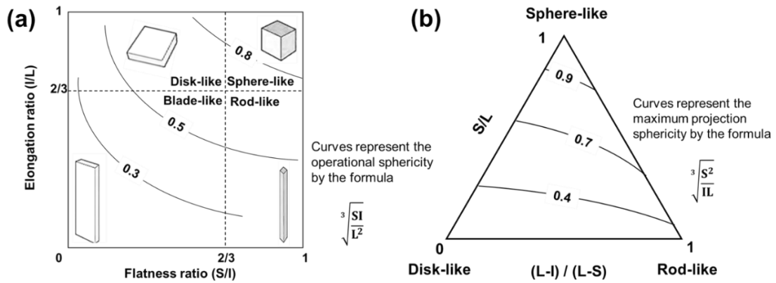
Figure 2-1. (a) Zingg diagram with the curves of operational sphericity and (b) Sneed-Folk diagram with the curves of maximum projection sphericity (Lewis and McConchie, 1994; Sneed and Folk, 1958; Zingg, 1935).
