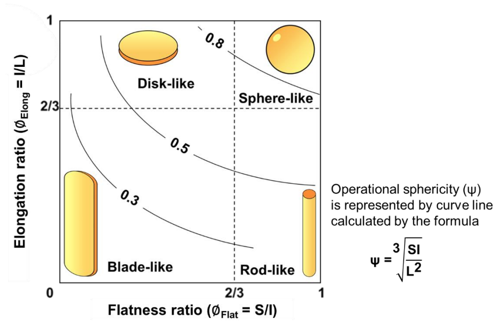
Figure 3-4. The Zingg diagram superimposed with operational sphericity (Zingg, 1935).
