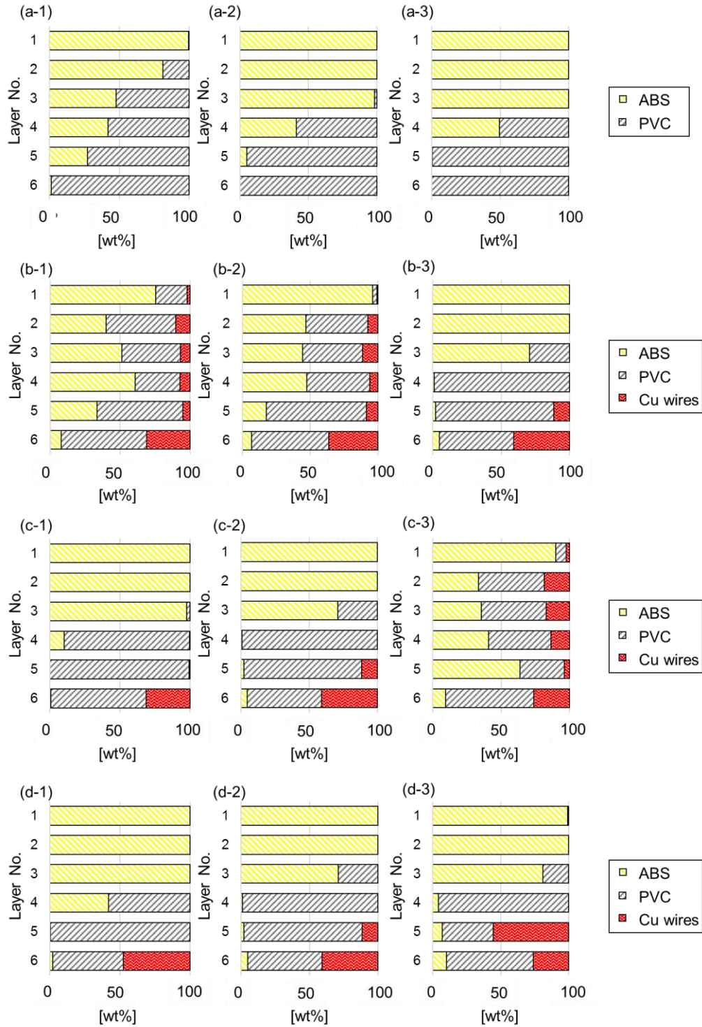
Figure 5-4. The proportion of ABS, PVC and Cu wires in each layer after the jig separation of model samples: (a) without Cu wires at separation time of (a-1) 1 min, (a-2) 2 min, and (a-3) 3 min; (b) with 10% Cu wires of 30-mm long at separation time (b-1) 1 min, (b-2) 2 min, and (b-3) 3 min; (c) with 30-mm Cu wires at Cu wire content of (c-1) 5%, (c-2) 10%, and (c-3) 15% (separation time 3 min); (d) with 10% Cu wires at Cu wire length of (d-1) 10 mm, (d-2) 30 mm, and (d-3) 50 mm (separation time 3 min).
