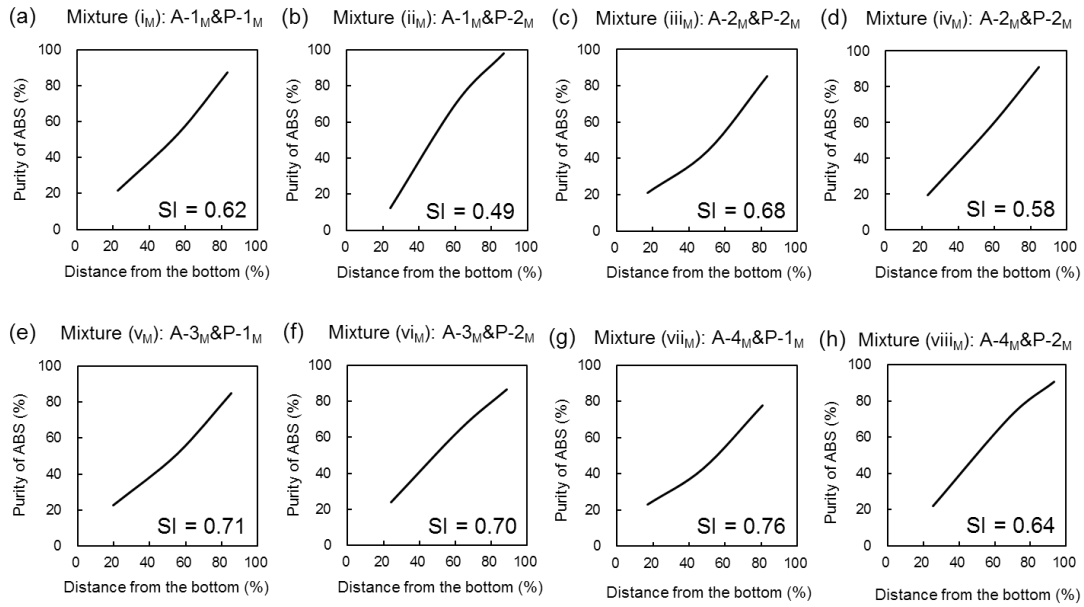
Figure 4-9. The relationship between distance from the bottom and purity of ABS after jig separation using normal waveform of (a) mixture (i M ), (b) mixture (ii M ), (c) mixture (iii M ), (d) mixture (iv M ), (e) mixture (v M ), (f) mixture (vi M ), (g) mixture (vii M ), and (h) mixture (viii M ) with the values of sharpness index (SI).
