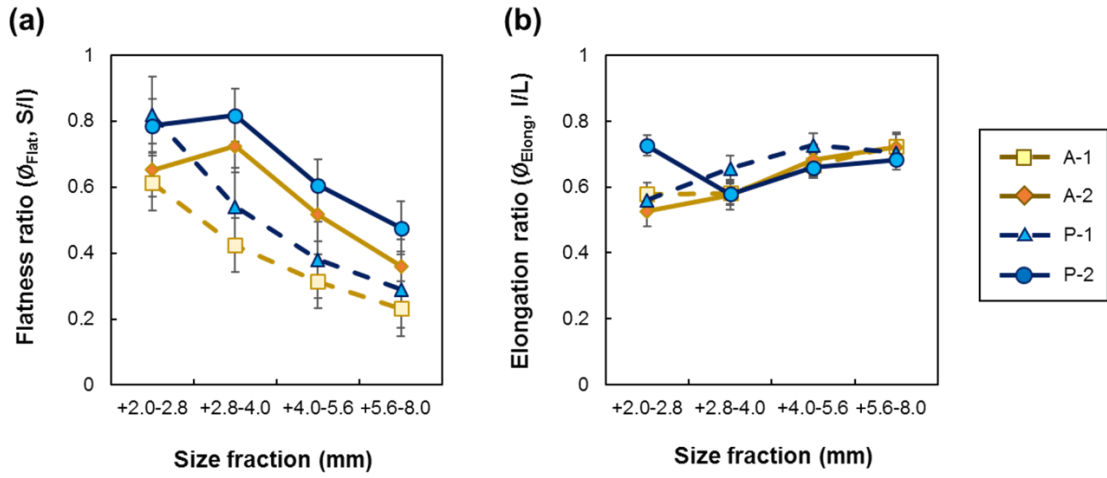
Figure 3-6. Changes in the average values of (a) flatness ratio ( \phi_{Flat} ) and (b) elongation ratio ( \phi_{Elong} ) of plastic samples as a function of particle size distribution.
