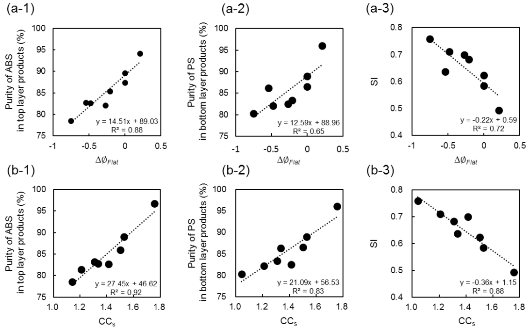
Figure 4-10. (a) The relationship of \Delta\phi_{Flat} with (a-1) purity of light plastic (ABS) in top layer product, (a-2) purity of heavy plastic (PS) in bottom layer products, and (a-3) sharpness index and (b) the relationship of CC_s with (b-1) purity of light plastic (ABS) in top layer products, (b-2) purity of heavy plastic (PS) in bottom layer products, and (b-3) sharpness index (SI).
