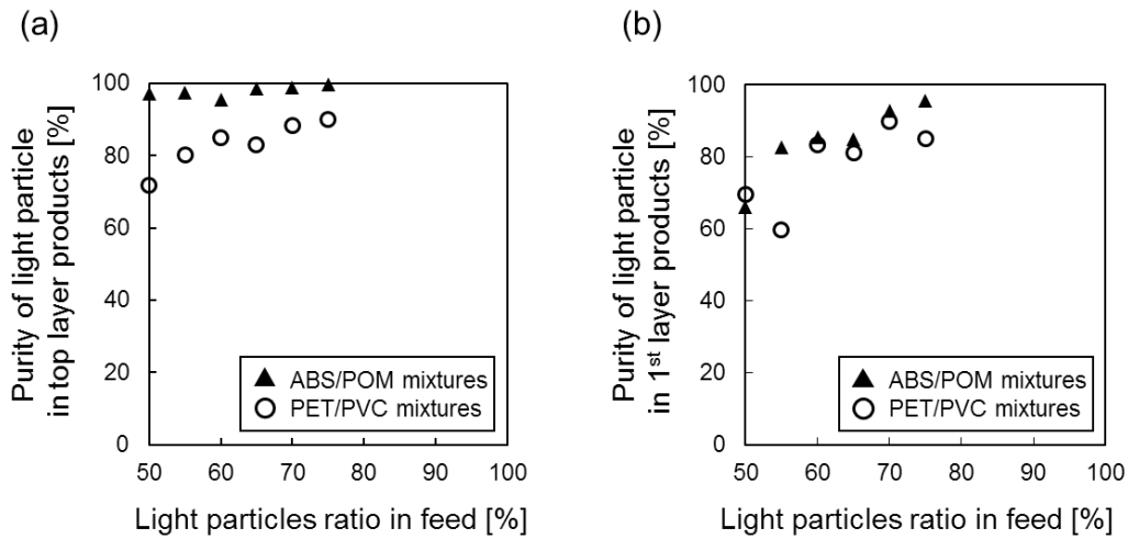
Figure 6-5. Relation between the light particles ratio in feed and (a) purity of light particles in top layer products from continuous-type jig experiments and (b) purity of light particles in 1 st layer products from batch-type jig experiments.
