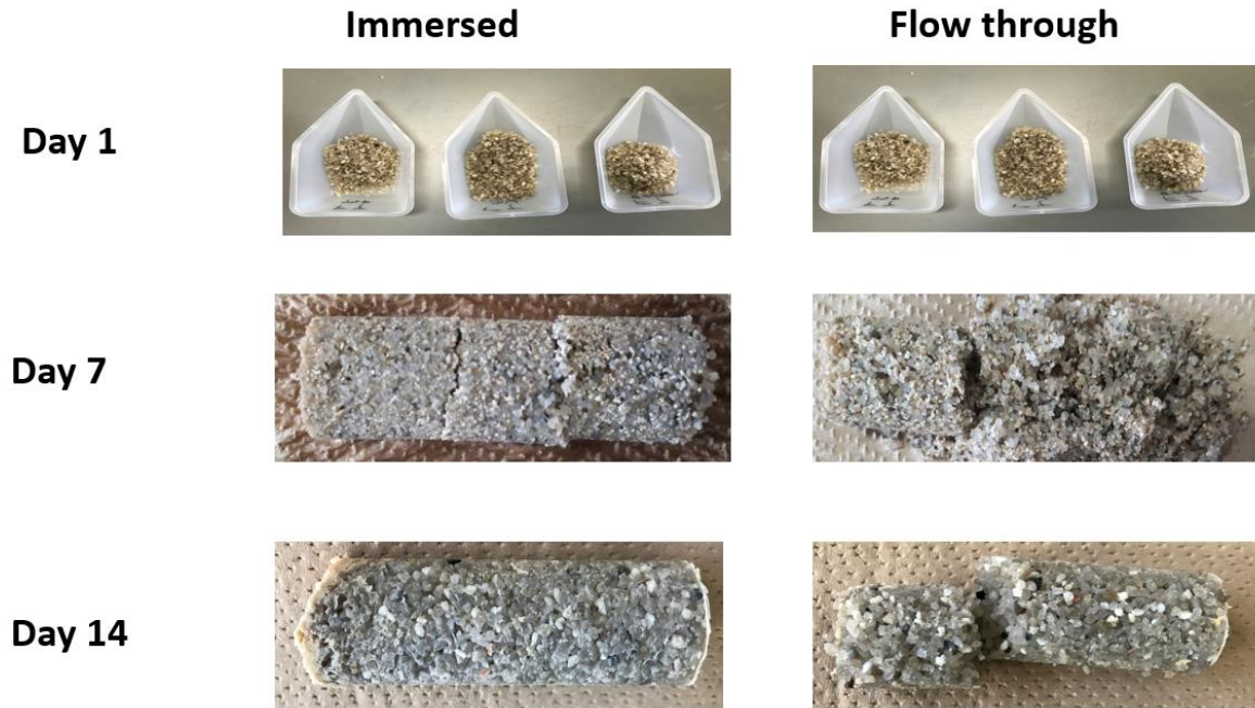
Fig. 3.11: Visualization of biocemented sand mediated by O. profundus KBZ 1-3 treated by both immersed and flow through treatment methods at day 1, 7 and 14 days
