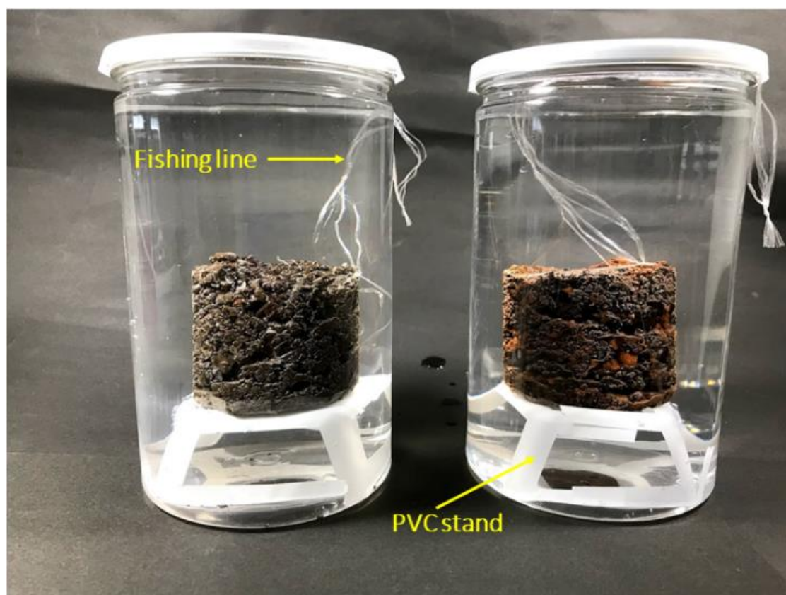
Fig. 2.14 USA EPA Method 1315 setup of the 3D leaching configuration of (a) biocemented KS and (b) biocemented KS/LPR
