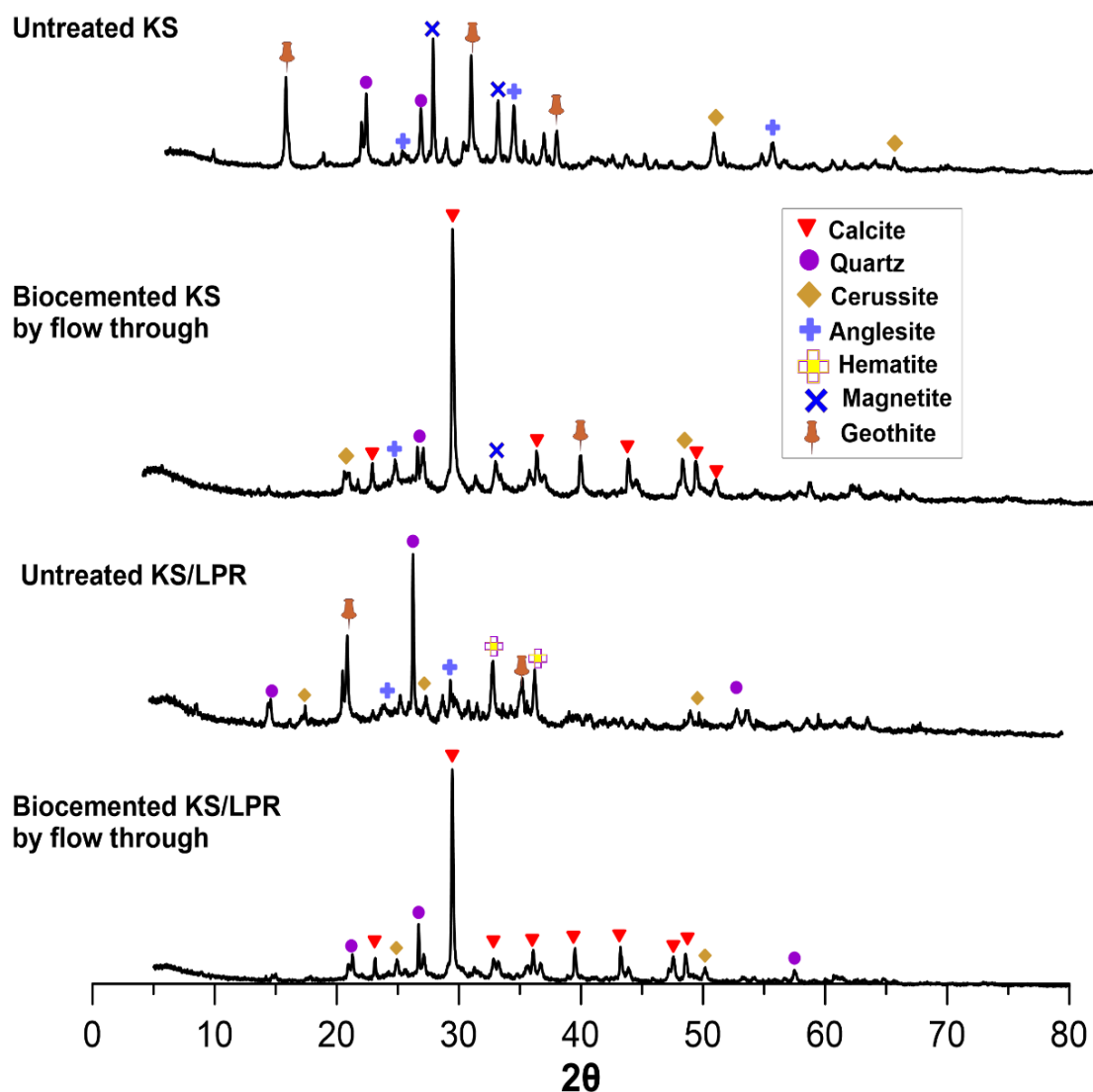
Fig. 2.24: Typical XRD patterns of untreated and biocemented KS and KS/LPR
