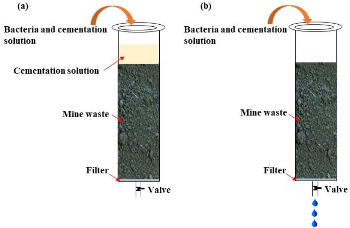
Fig. 2.12: Experimental setups for (a) immersed and (b) flow through methods for biocementation mine wastes
