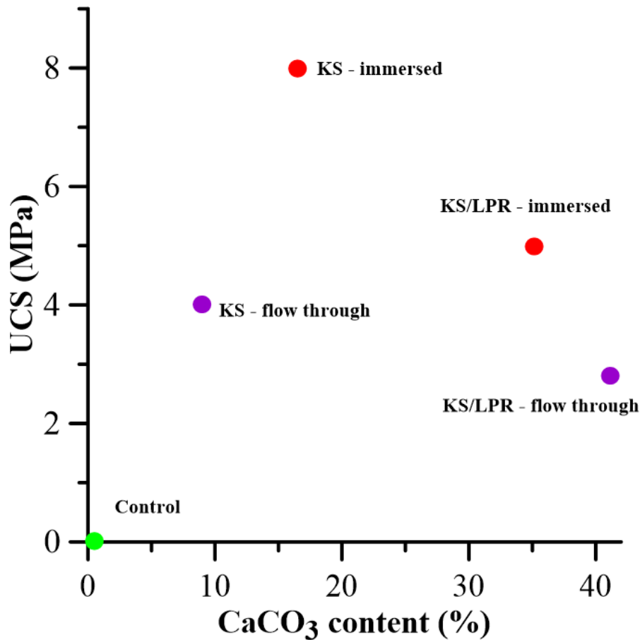
Fig. 2.23. Effect of \text{CaCO}_3 content on the UCS of on untreated, biocemented KS and KS/LPR treated by immersed and flow through methods.
