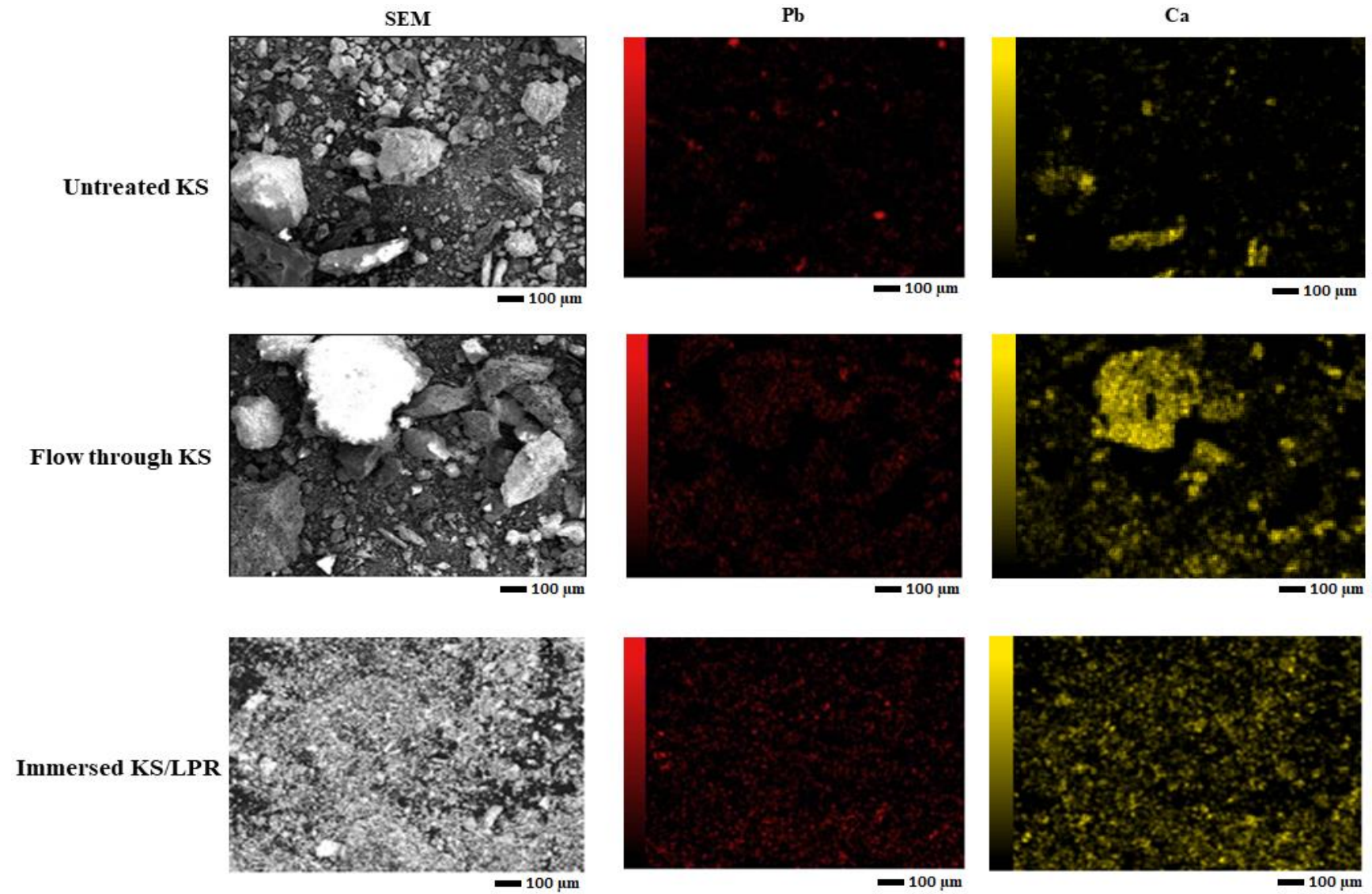
Fig. 2.26: SEM and EDS images of untreated and biocemented KS and KS/LPR
