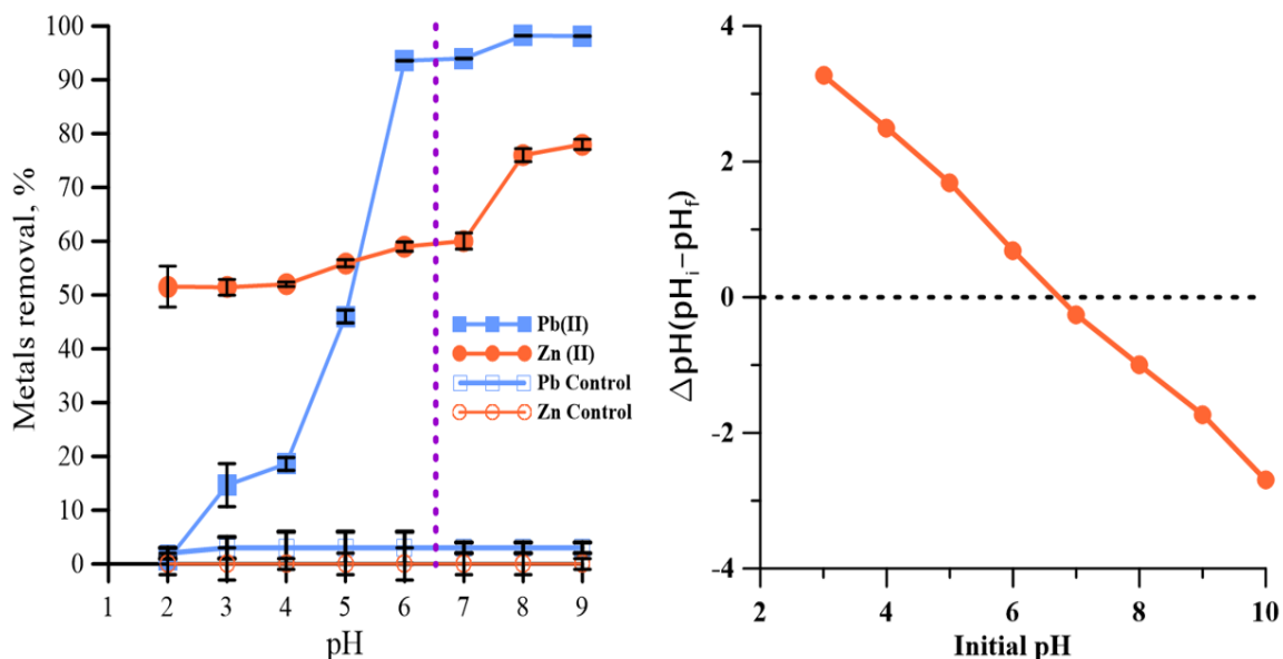
Fig. 5.16: Effect of pH (Initial metal ions were same - 20 mg/L at room temperature)
