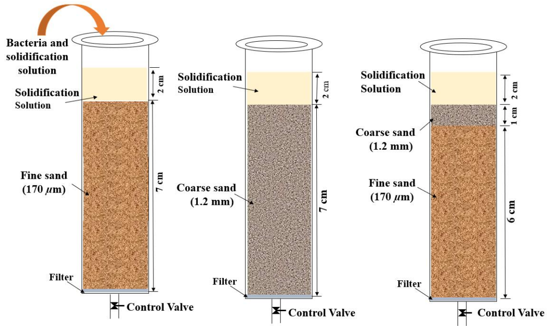
Fig. 2.11: Conceptual setup and of the syringe biocementation of coarse- and fine-grained sand
