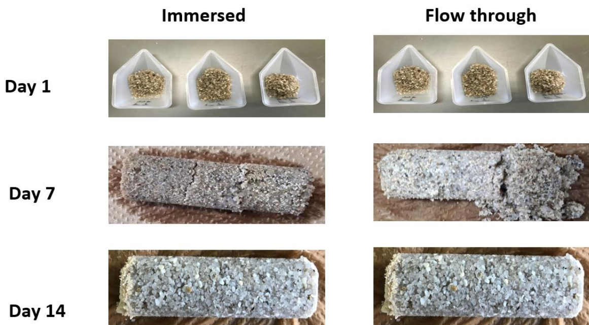
Fig. 3.12: Visualization of biocemented sand mediated by O. profundus KBZ 2-5 treated by both immersed and flow through treatment methods at day 1, 7 and 14 days.
