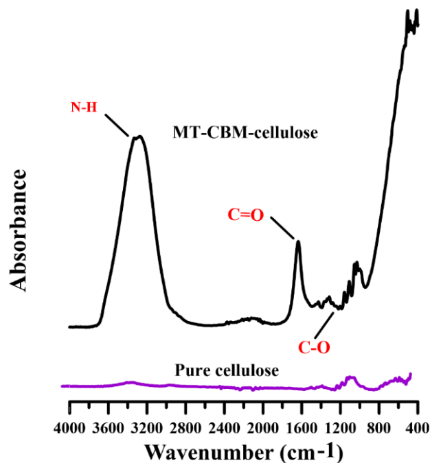
Fig. 5.15: FTIR analysis of pure cellulose (Whatman Paper No. 1) compared to cellulose-MT-CBM
