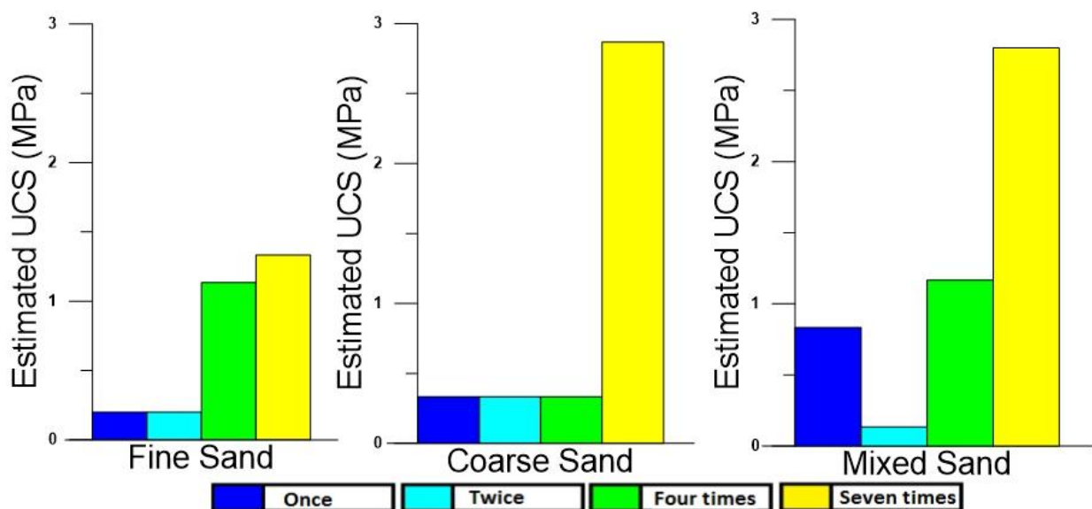
Fig. 2.18: UCS comparison of the results obtained when varying the bacteria injection for fine, coarse and mixed sand.
