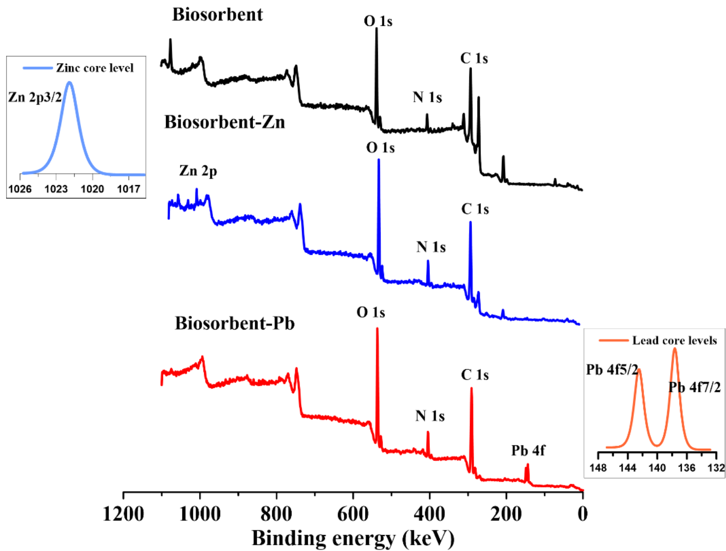
Fig. 5.21: The typical XPS wide scan spectra of cellulose-MT-CBM before and after Pb (II) and Zn (II) adsorption
