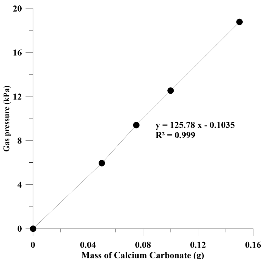
Fig. 2.13: Relationship between gas pressure and mass of calcium carbonate.
