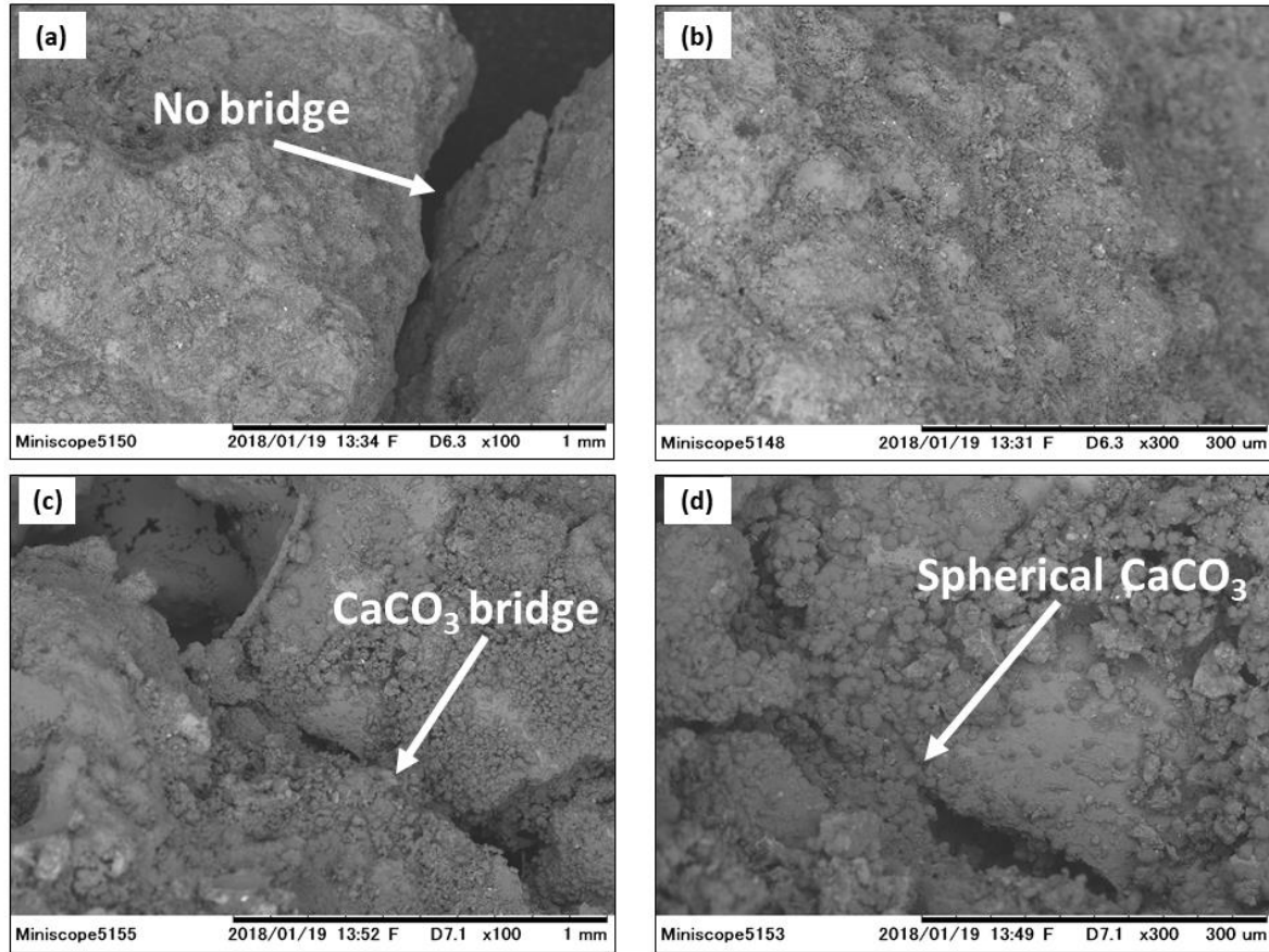
Fig. 2.25: SEM images of (a) untreated KS at x100 magnification, (b) untreated KS at x300 magnification, (c) biocemented KS prepared by immersed method at x100 magnification, and (d) biocemented KS prepared by immersed method at x300 magnification
