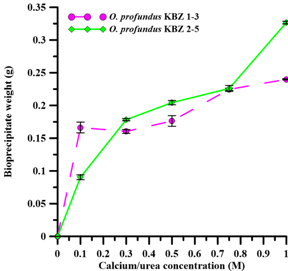
Fig. 3.8: Weight of \text{CaCO}_3 bioprecipitated by O. profundus KBZ 1-3 and O. profundus KBZ 2-5 at different equimolar concentrations of calcium and urea. Error bars indicate the standard deviation of three independent replicates.
