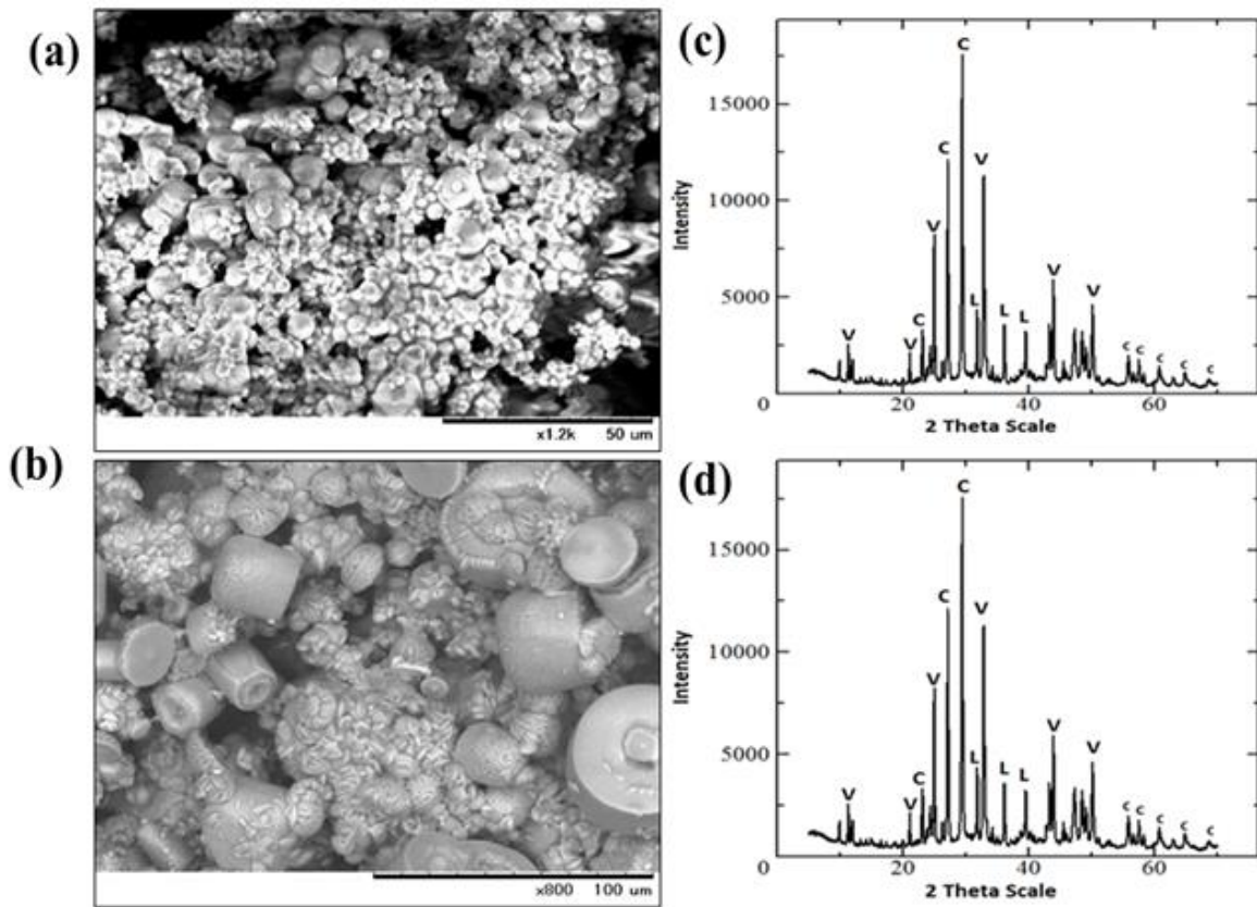
Fig. 2.17: SEM images (a, b) and XRD data (c, d) of precipitates formed by Pararhodobacter sp. in the absence (a, c) and presence of 5 mM Pb (b, d). (C = Calcite ( \text{CaCO}_3 ); V = Vaterite ( \text{CaCO}_3 ); L = Lead Oxide ( \text{PbO} )).
