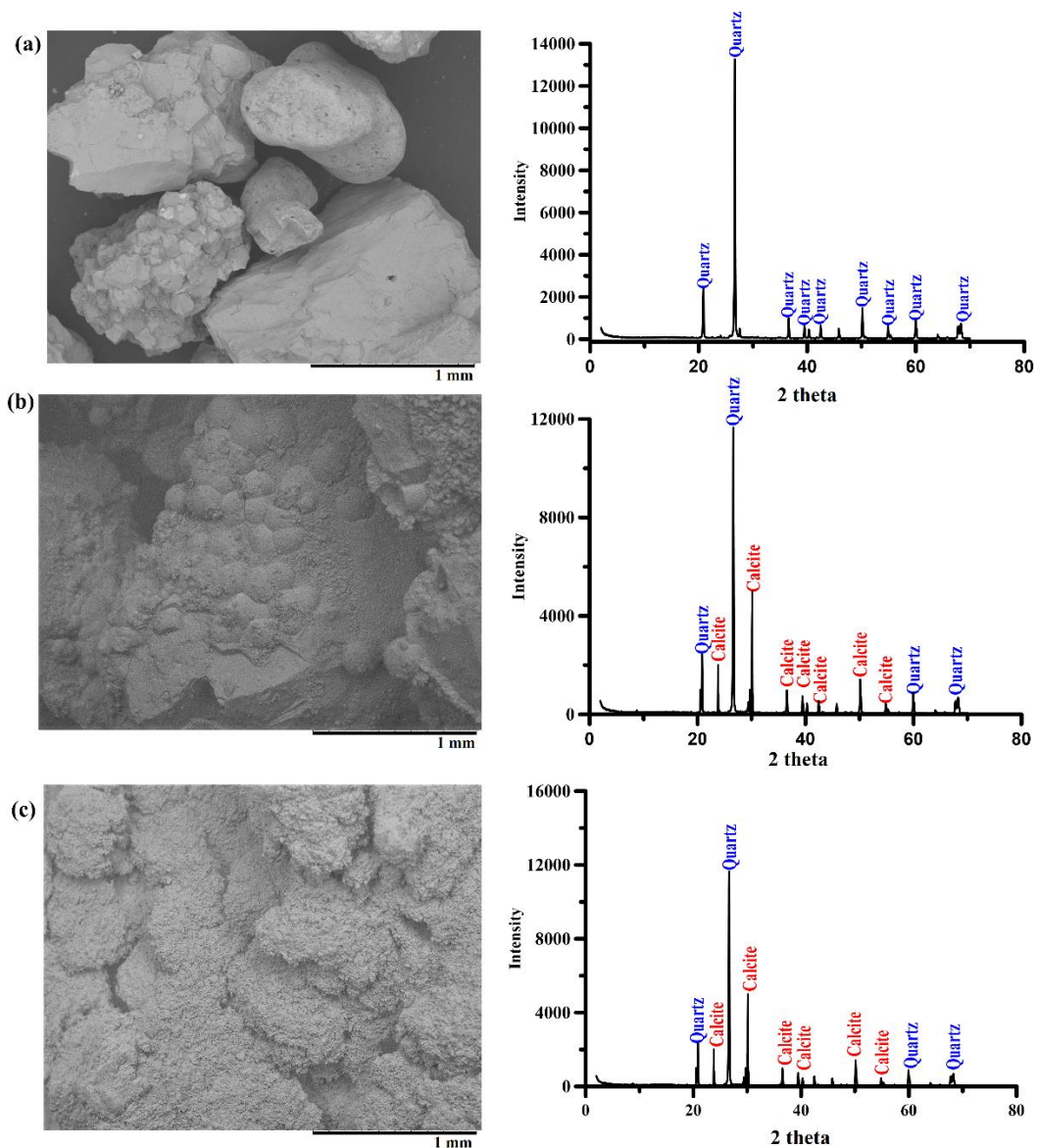
Fig. 3.10: SEM view and the corresponding XRD analysis comparing (a) control specimen, (b) biocemented sand prepared by the flow-through method using O. profundus KBZ 1-3, and (c) biocemented sand prepared by the flow-through method using O. profundus KBZ 2-5.
