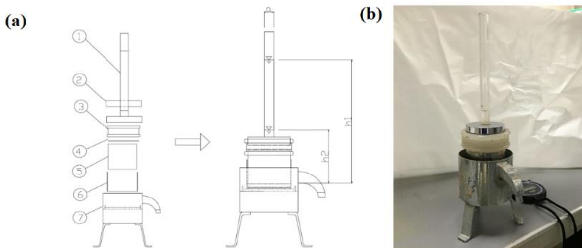
Fig. 2.7. (a) DIK 4000 system for measuring hydraulic conductivity where 1 = scale tube; 2 = weight for supporting scale tube; 3 = silicon rubber ring; 4 = O ring; 5 = cylindrical sample holder; 6 = casing for sample holder; 7 = water tank. (b) DIK 4000 system used in this study with a stopwatch
