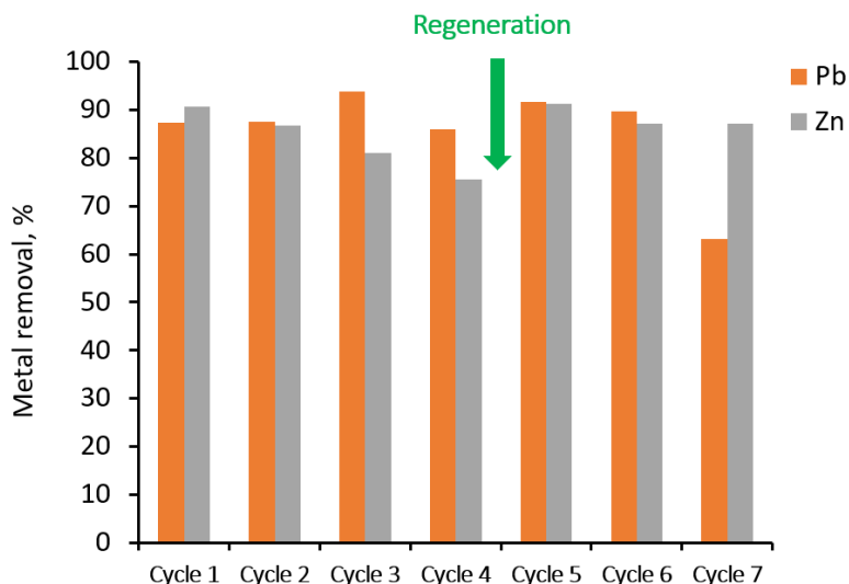
Fig. 5.20: Pb (II) and Zn (II) removal efficiency of Cellulose-MT-CBM at different cycles (Initial metal ions were same - 20 mg/L, pH = 6.5 at room temperature).
