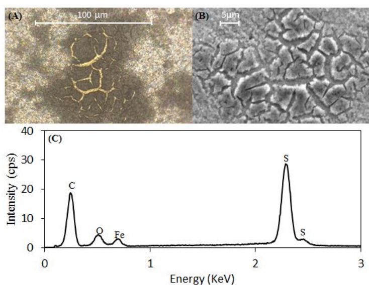
Fig. 3-3 Surface analysis of pyrite after treatment in [\text{Fe}(\text{cat})_2]^{-} for 4 days: (A) optical microscope photomicrograph, (B) SEM photomicrograph, and (C) EDX spectrum of observed area in (B)
