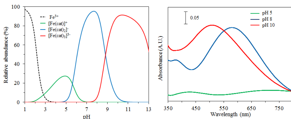
Fig. 3-1 (A) The speciation diagram with pH of \text{Fe}^{3+} and its catecholate species ( [\text{Fe}^{3+}] = 1 \text{ mM} and [\text{cat}] = 0.3 \text{ mM} ) and (B) UV-Vis spectra of solutions containing 0.1 mM \text{Fe}^{3+} and 0.3 mM catechol under various pH conditions
