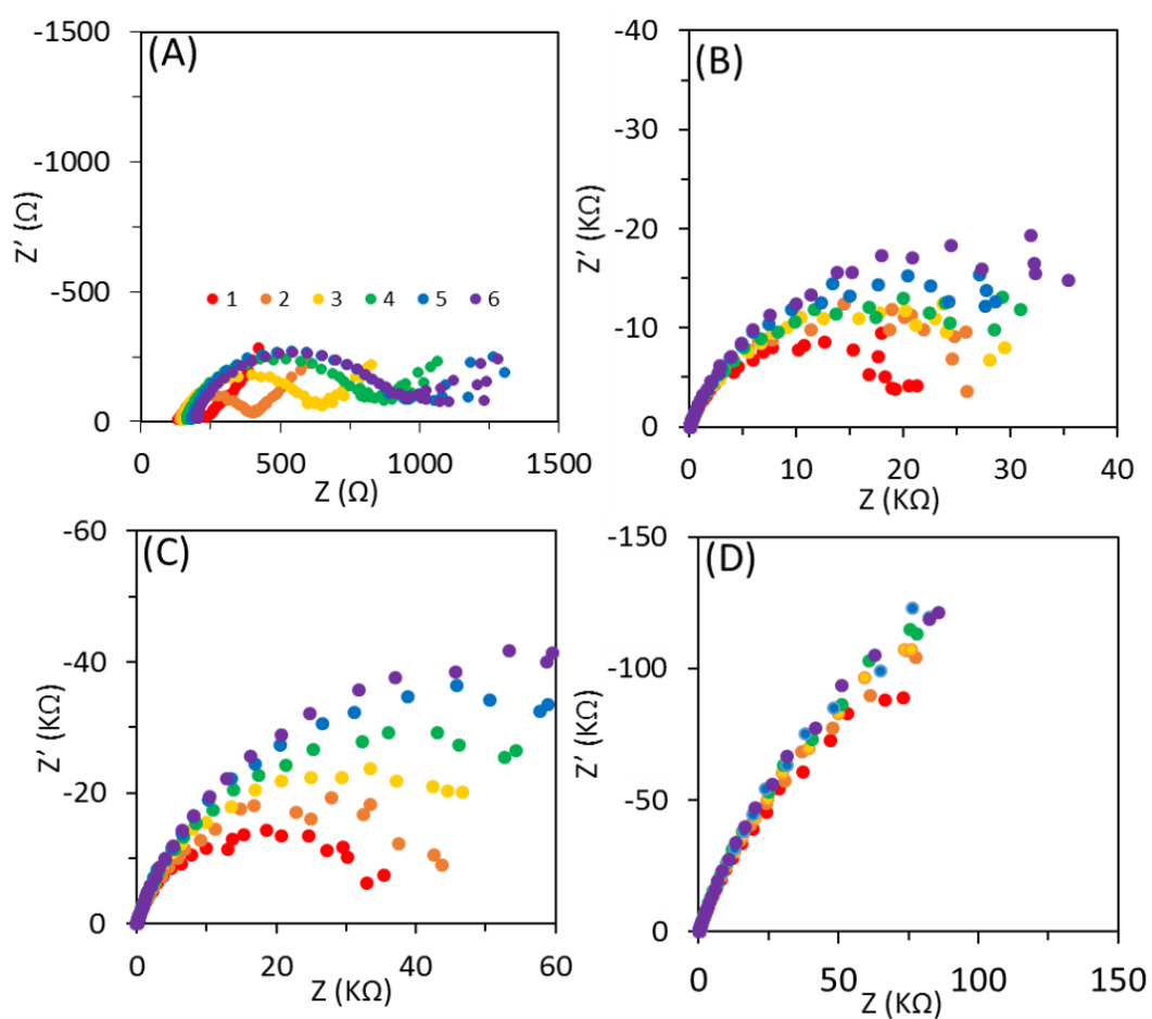
Fig. 2-6 Results of EIS after each set of 10-min polarization with (A) \text{Fe}^{3+} -catecholate complex, (B) \text{Al}^{3+} -catecholate complex, (C) \text{Ti}^{4+} -catecholate complex and (D) without metal-catecholate complex solutions
