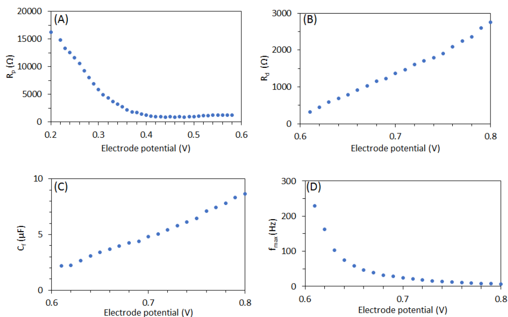
Fig. 4-12 Fitting results of impedance spectra measured after oxidative decomposition of \text{Fe}^{3+} -catecholate complexes
