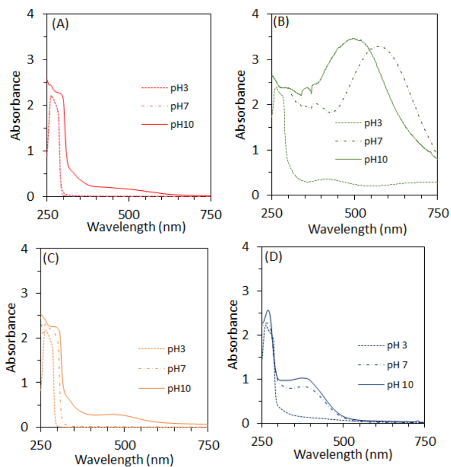
Fig 2-3 UV-Vis spectra of solutions containing (A) catechol, (B) \text{Fe}^{3+} -catecholate complexes, (C) \text{Al}^{3+} -catecholate complexes and (D) \text{Ti}^{4+} -catecholate complex
