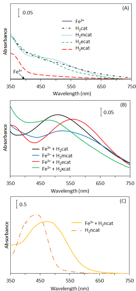
Fig. 5-2 UV-Vis spectra of solution containing (A) \text{Fe}^{3+} or ligand (except \text{H}_2\text{ncat} ) (B) \text{Fe}^{3+} and ligand (except \text{H}_2\text{ncat} ) and (C) \text{H}_2\text{ncat} with or without \text{Fe}^{3+}
