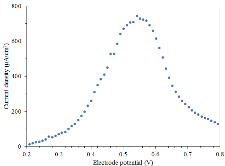
Fig. 4-10 Equilibrium current generated from the oxidative decomposition of \text{Fe}^{3+} -catecholate complex under different electrode potentials
