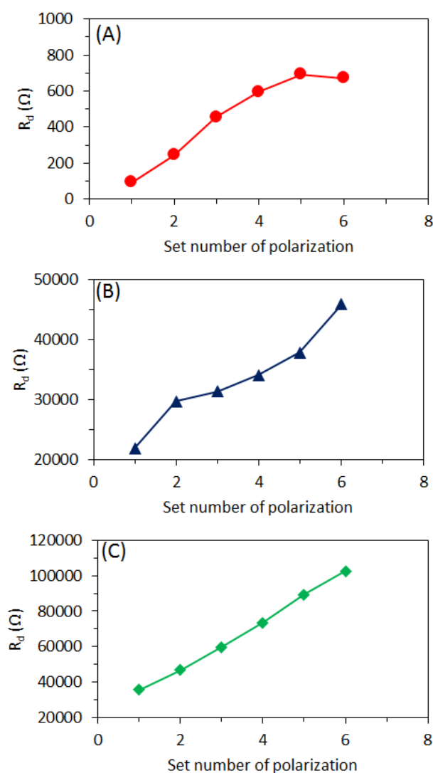
Fig. 2-8 Fitting results of R_d in the coating formed after each set of 10min-polarization in (A) Fe 3+ -catecholate complex, (B) Al 3+ -catecholate complex and (C) Ti 4+ -catecholate complex solutions
