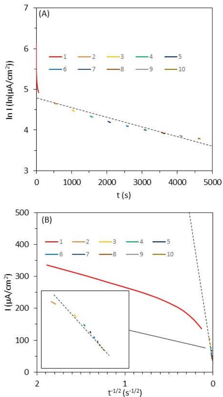
Fig. 4-7 (A) Relationship between \ln I and t and (B) relationship between I and t^{-1/2}
