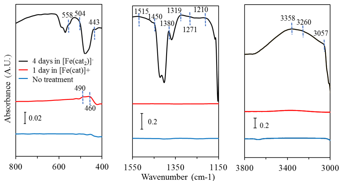
Fig. 3-4 ATR-FTIR spectra of pyrite before and after treatment with [\text{Fe}(\text{cat})]^+ for 1 day and [\text{Fe}(\text{cat})_2]^- for 4 days. Note variations in the vertical scale
