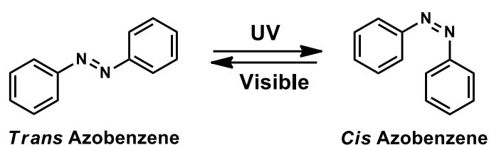
Figure1-1: Photoisomerization of azobenzene
