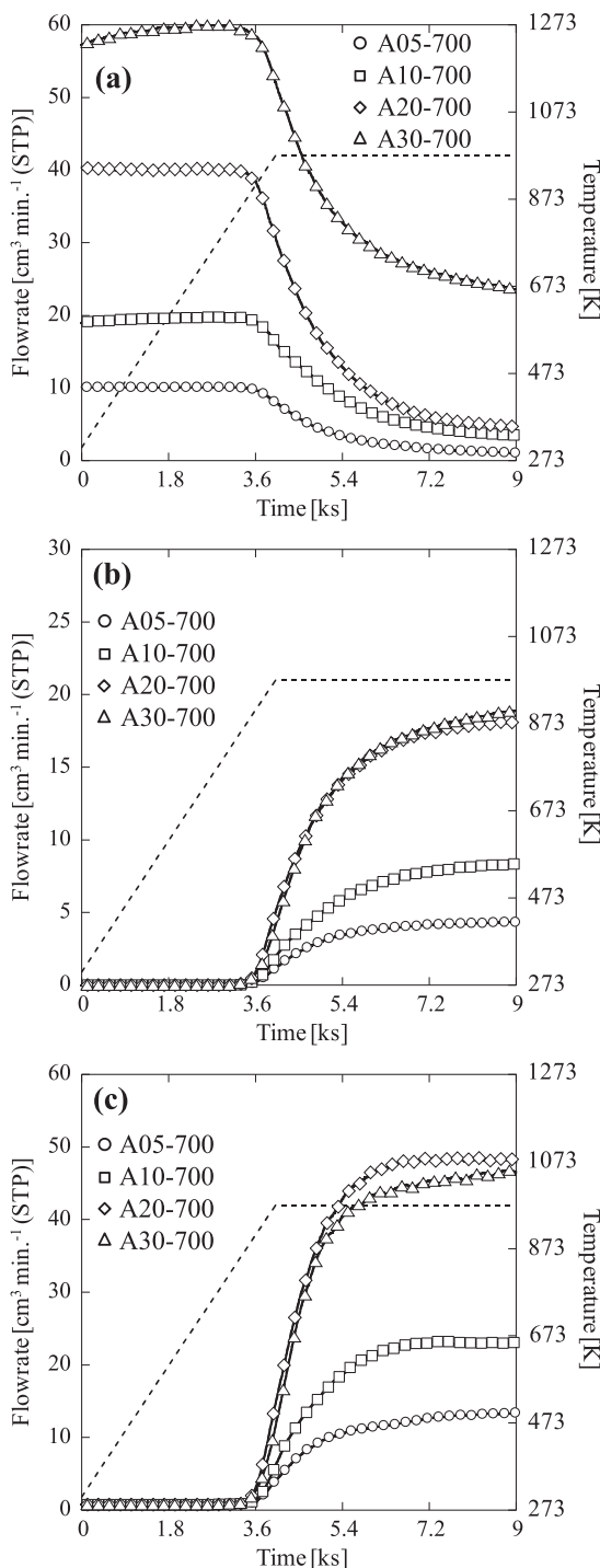
Fig. 6. Changes in the flow rate of (a) ammonia, (b) nitrogen, and (c) hydrogen at different ammonia inflow during heating up to 973 K and then holding at this temperature.
