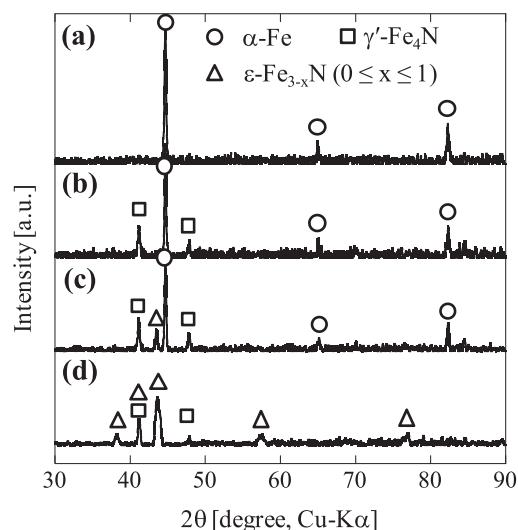
Fig. 7. XRD patterns of the samples reduced at different ammonia concentrations: (a) A05-700, (b) A10-700, (c) A20-700, and (d) A30-700.
