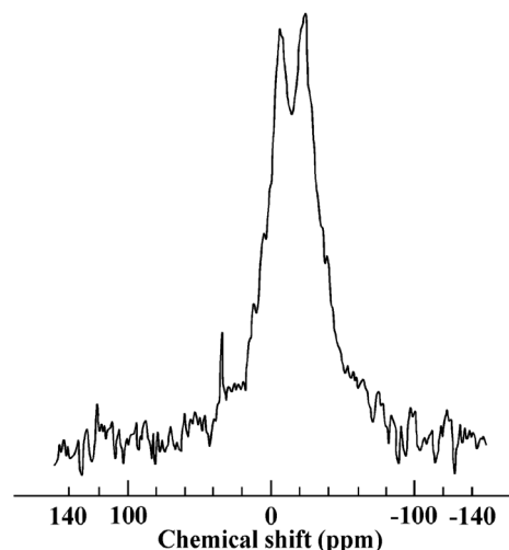
Fig. 5. Solid-state 23 Na-NMR spectrum for YRB coal.
