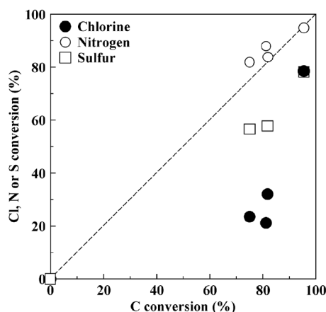
Fig. 10. Relationship between carbon conversion and chlorine, nitrogen or sulfur conversion during \text{O}_2 -blown entrained bed gasification under pressure.
