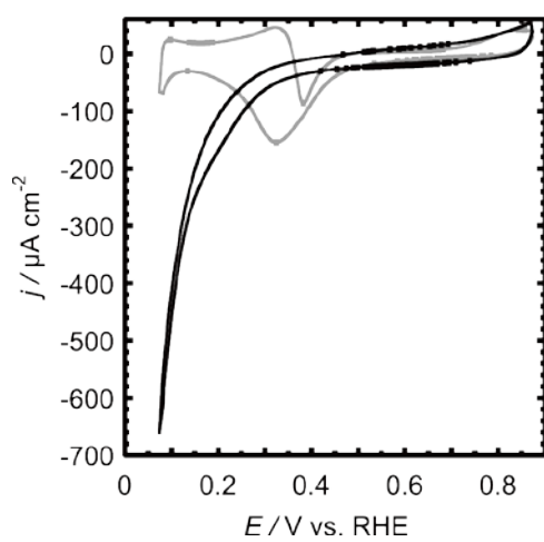
(c) Sn/PdPt(100)
