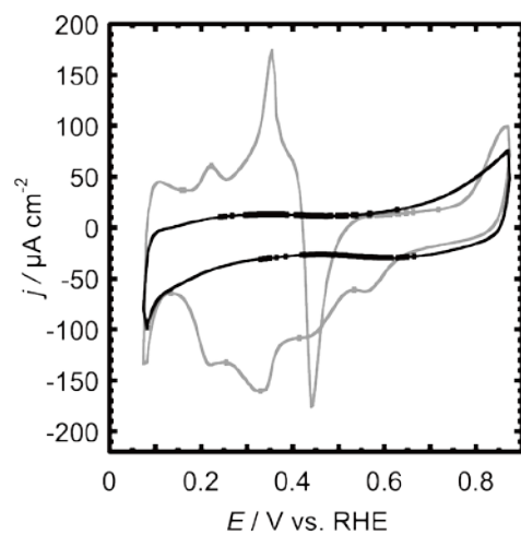
(c) Sn/PdPt(100)
