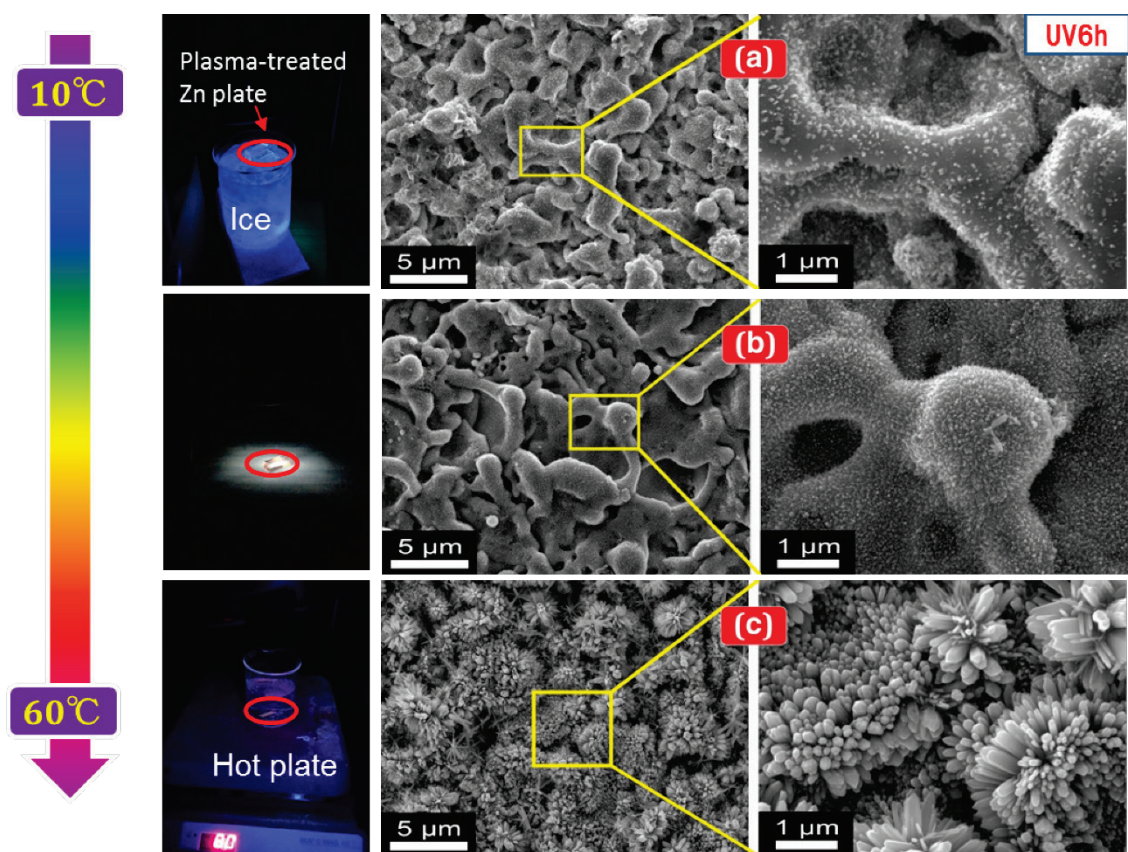
Figure 3.7 - Water temperature effect in ZnO crystallites growth under UV 6h irradiation. (a) Low-temperature (~10 °C). (b) Room temperature (~25 °C). (c) High-temperature (~60 °C).
