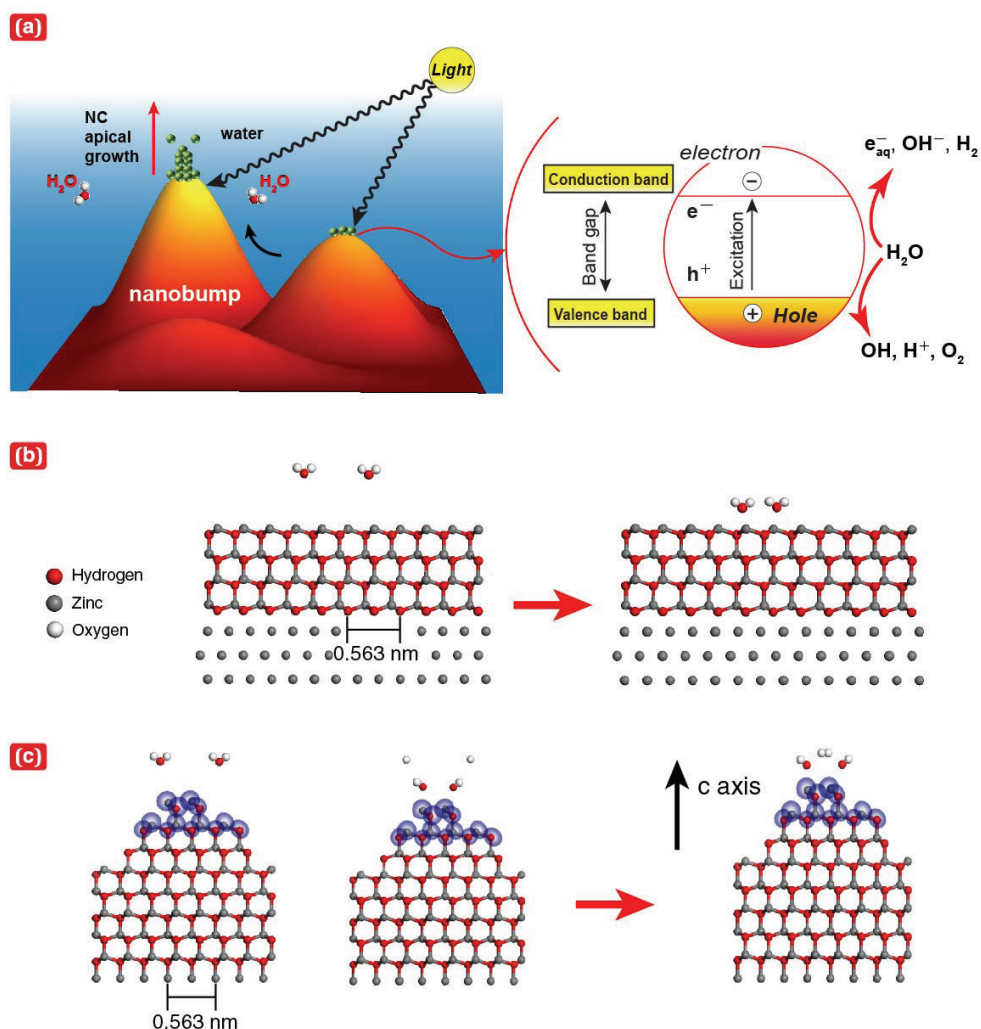
Figure 3.5 - Nanobumped surface effect in the SPSC model and simulation by molecular dynamical ab initio calculations. (a) A schematic of SPSC with a nanobumped surface. (b) H 2 O molecules with a flat surface of ZnO. Water molecules localise at stable places near the flat surface. (c) Water molecule stabilised on the top of a nanobump (radius of curvature, R = 0.5 nm). Electron density isosurfaces of 2.0 electron/Å 3 (purple coloured) are observed only near the top of a nanobump. The state was relaxed to a state where a H 2 molecule is formed by equilibrating the state with the dissociation of H 2 O molecules into OH and H.
