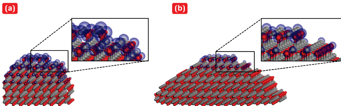
Figure 3.6 - Curvature radius dependence of the 1.7 electron/ \text{\AA}^3 electron density isosurfaces for nanobumped ZnO. (a-b) R = 1.0 and 2.0 nm, respectively. The isosurfaces are indicated by the purple coloured region. The larger radius of curvature resulted in decreased electron density at the apex.
