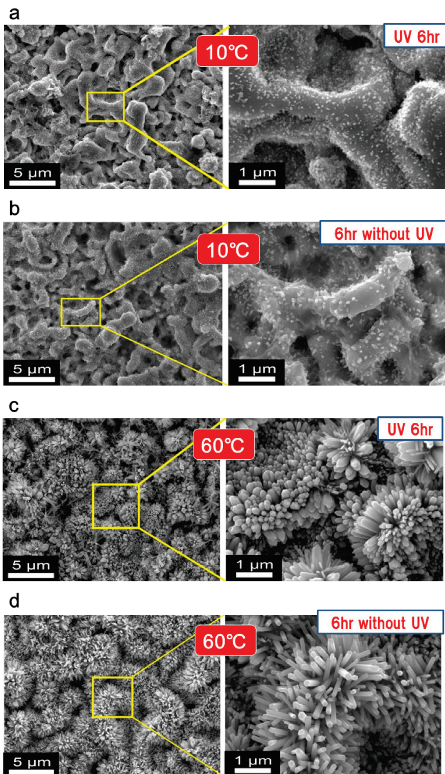
Figure 3.8 - Crystallites growth under UV and without UV conditions at elevated temperatures. (a) Zn UV 6h (Plasma 140 V, 10 min, T \approx 10 °C). (b) Zn without UV 6h (Plasma 140 V, 10 min, T \approx 10 °C). (c) Zn UV 6h (Plasma 140 V, 10 min, T \approx 60 °C). (d) Zn without UV 6h (Plasma 140 V, 10 min, T \approx 60 °C).
