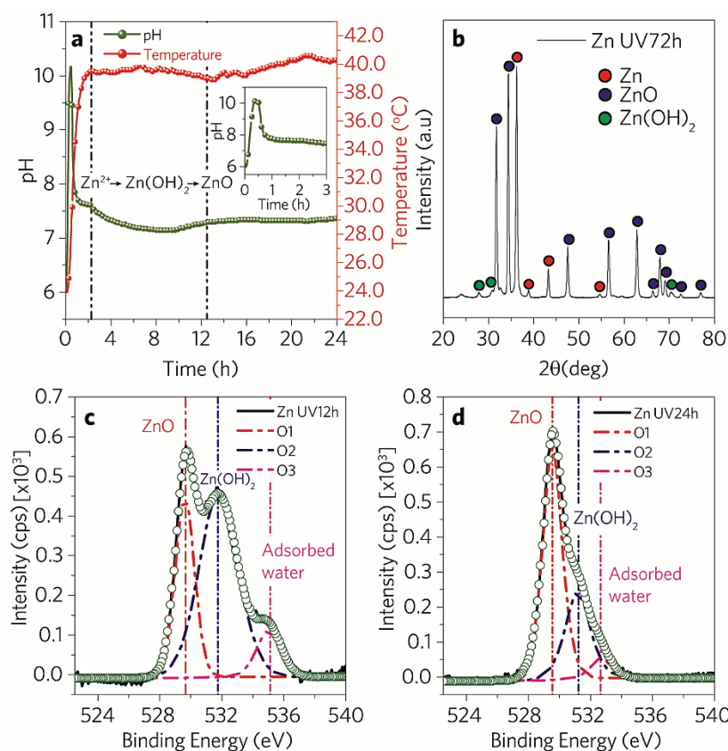
Figure 4.6 - SPSC photoreaction mechanism and surface structure analysis. (a) pH-T graph of UV 24h SPSC of ZnO NRs. The inset is a magnified view of the pH change in the ultrapure water over a period of 3 h. (b) XRD patterns of UV 72h specimen. (c-d) XPS O 1s peak of Zn UV 12h and UV 24h specimens deconvoluted into three Gaussian-Lorentzian peaks.
