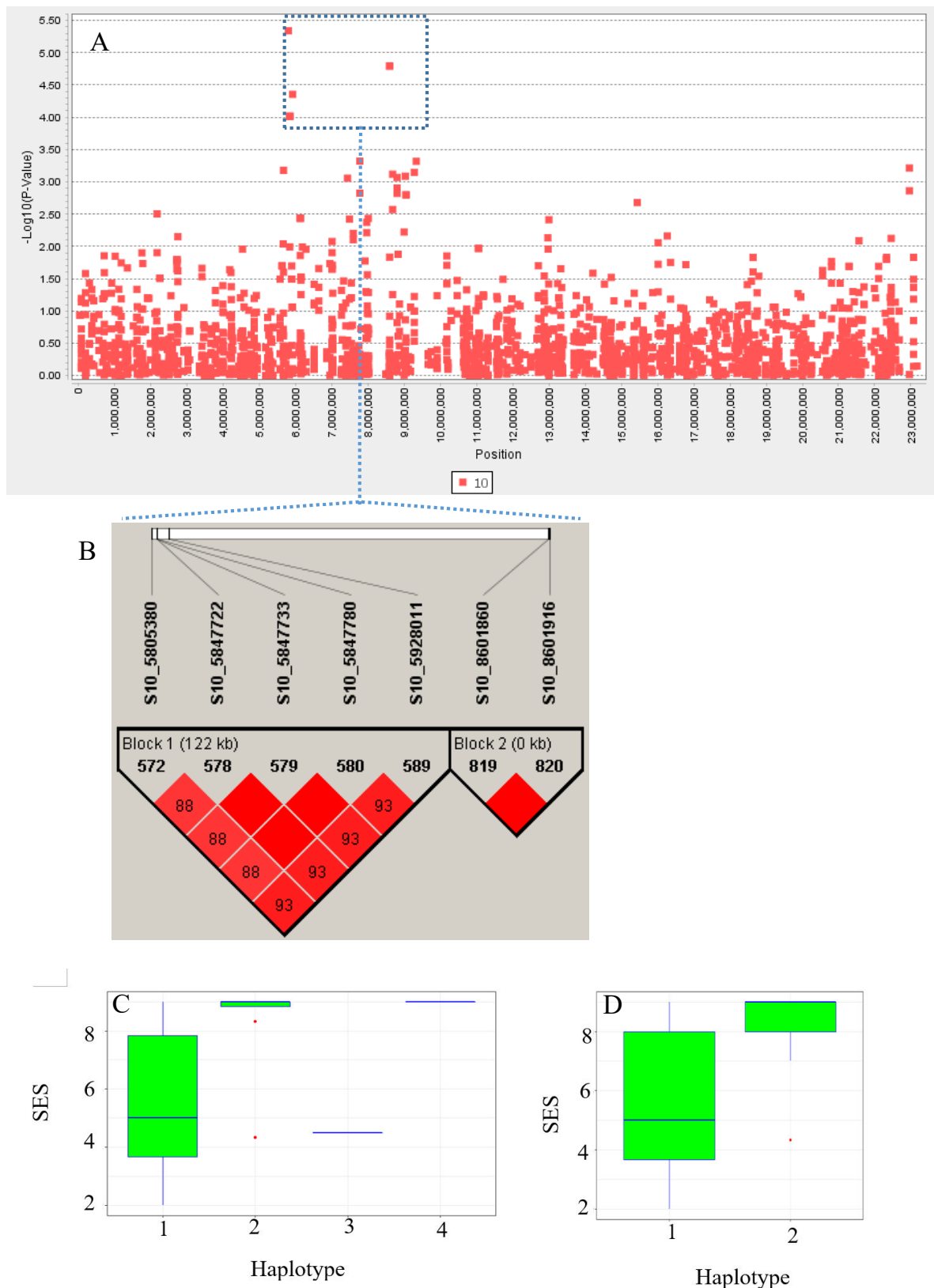
Figure 3.10. Analyses of significant SNP including the SNP peak for salinity traits on chromosome 10
