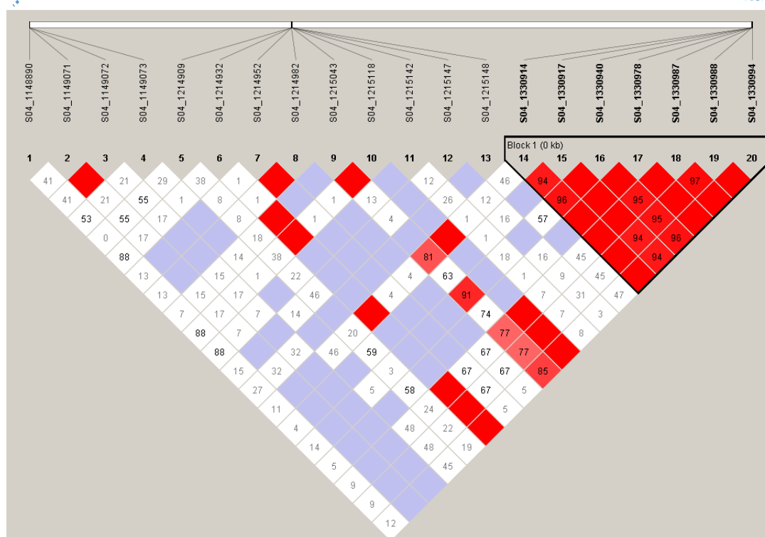
Figure 3.9. Analyses of the peak for salinity traits on chromosome 04
