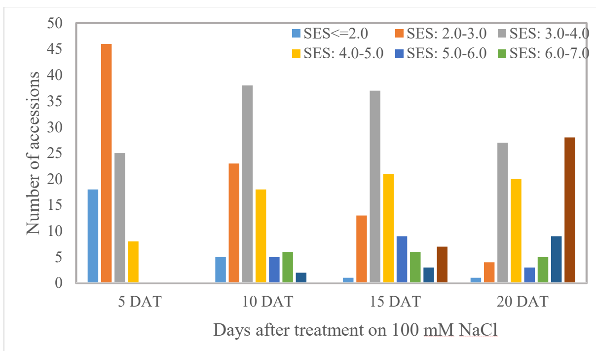
Fig 3.2. Number of accessions in difference categories
