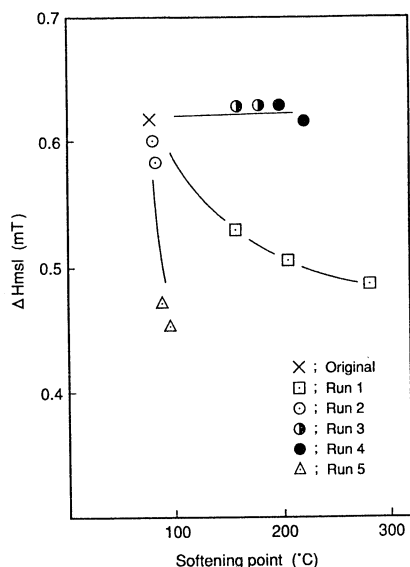
Fig.4 The variation of peak-to-peak line-width ( \Delta H_{\text{msl}} ) of pitches with softening point.
