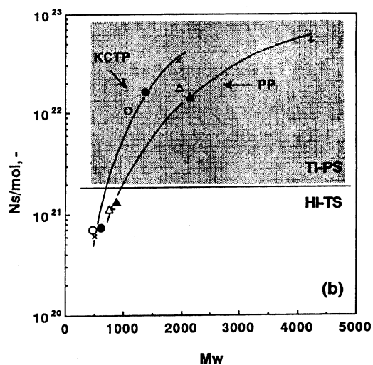
Fig.2 Relationships between average molecular weight ( Mw ) and spin concentration ( Ns/g : a), and mol spin concentration ( Ns/mol : b) for the fractionated pitches; KR : ×, KA : ○, KN : ●, PR : +, PA : △, PN : ▲
