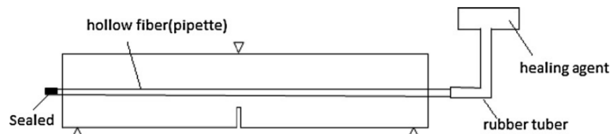
Fig. 1.5: Testing diagram of external healing agent supply system [10]
