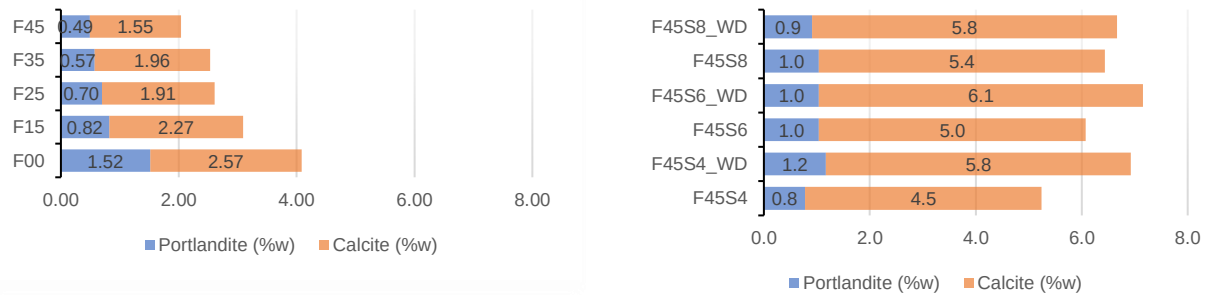
Fig. 2.16: Thermogravimetric analysis results [mass%] for portlandite content and calcite content
