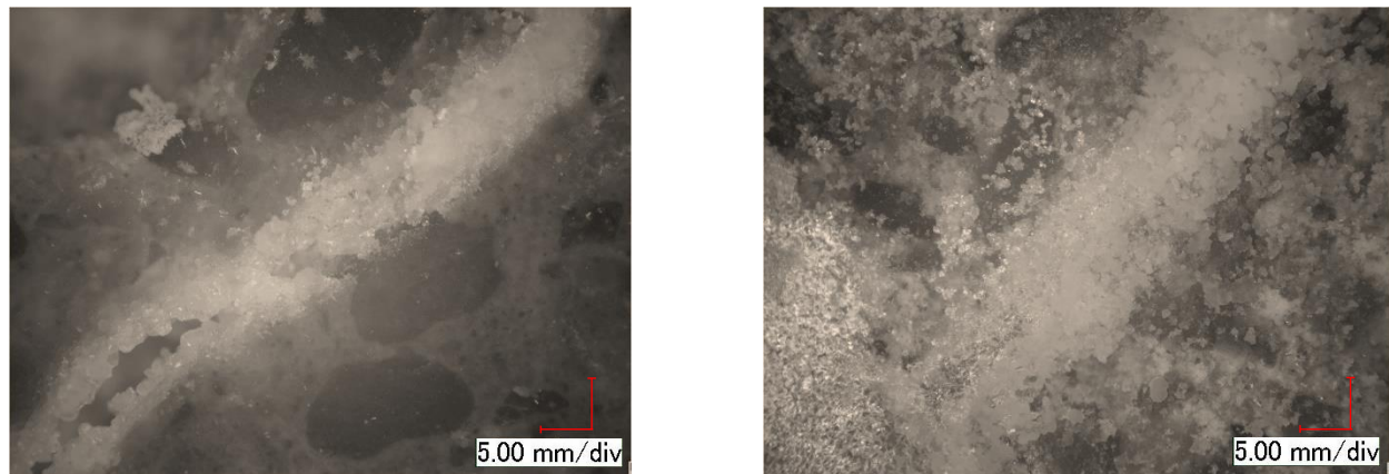
Fig. 3.15: Healed crack of F00 (left) and F00_WD (right)
