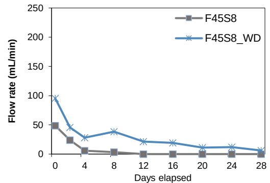
Fig. 2.12: Water discharge through cracks for F45S8 / F45S6_WD
