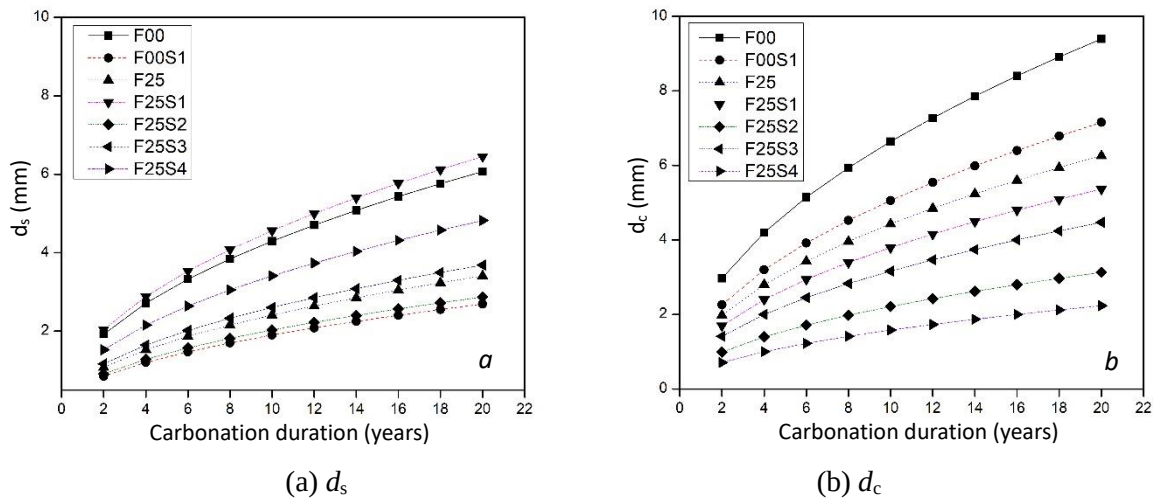
Fig. 4.3: Carbonation depths predicted until 20 years
