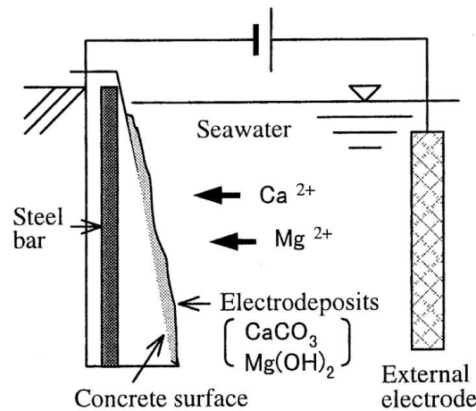
Fig. 1.7: Application of electrodeposition in marine structure [41]
