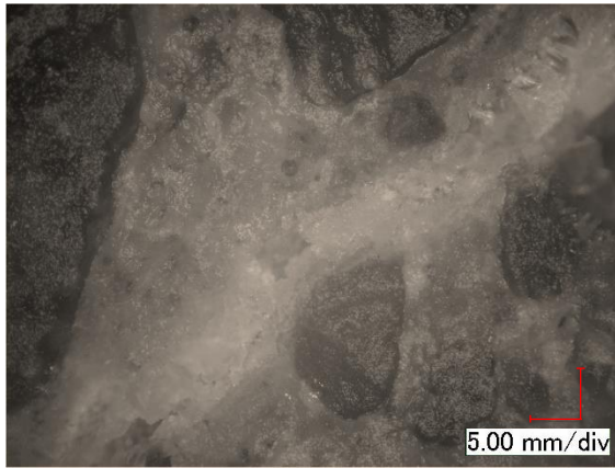
Fig. 3.16: Healed crack of RB20 (left) and RB20_WD (right)
