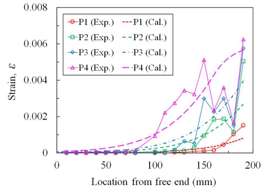
(b) Sato et al.'s model
