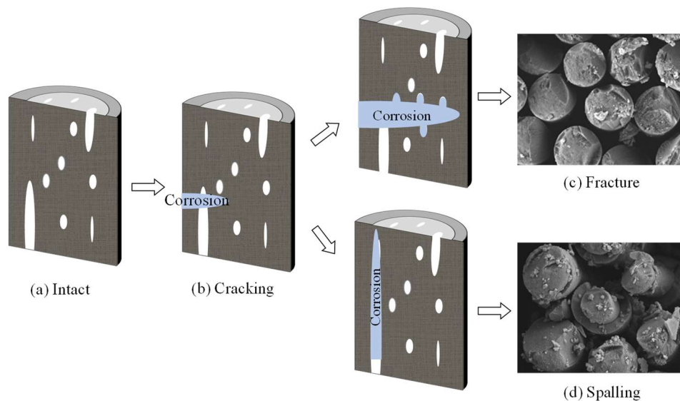
Fig. 4.12 Degradation of carbon filaments in the MFRCM subjected to anodic polarization
