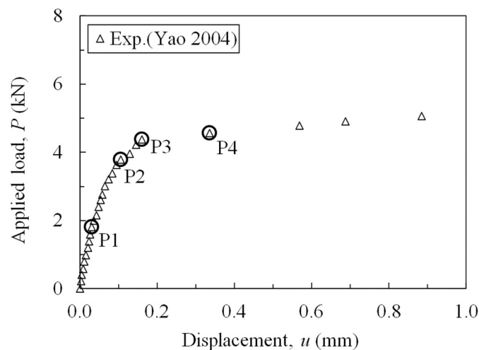
(a) The global force versus displacement curve
