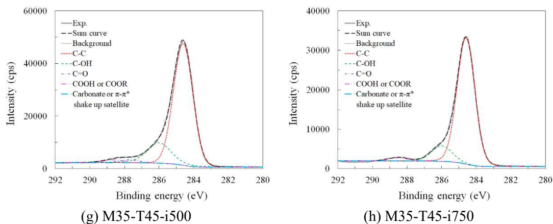
Fig. 4.9 Deconvolved C1s XPS spectra of carbon fabric in MFRCM composites without short carbon fibers
