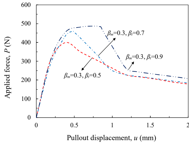
Fig. 3.18 The effect of \beta_t on P \sim u curves
