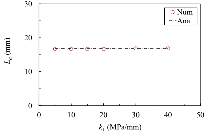
Fig. 2.14 The effect of k_l on L_a of carbon yarn in the cementitious matrix
