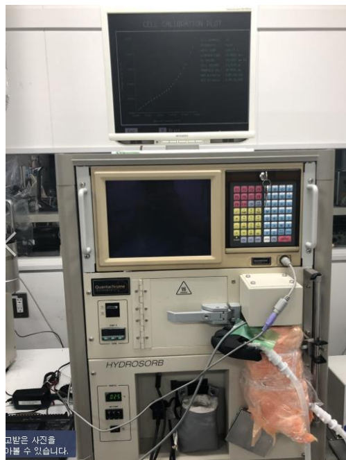
Fig. 2. 11 Actual feature of Quantachrome HYDROSORB 1000
