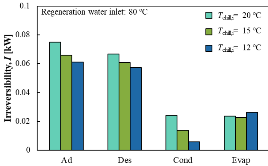
Fig. 6. 18 Irreversibility of each component according to temperature of chilled water
