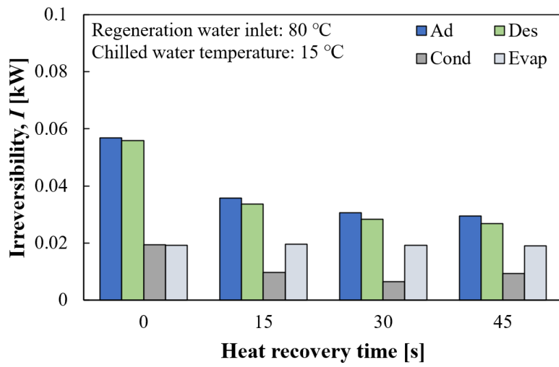
Fig. 6. 19 Irreversibility of each component according to heat recovery time
