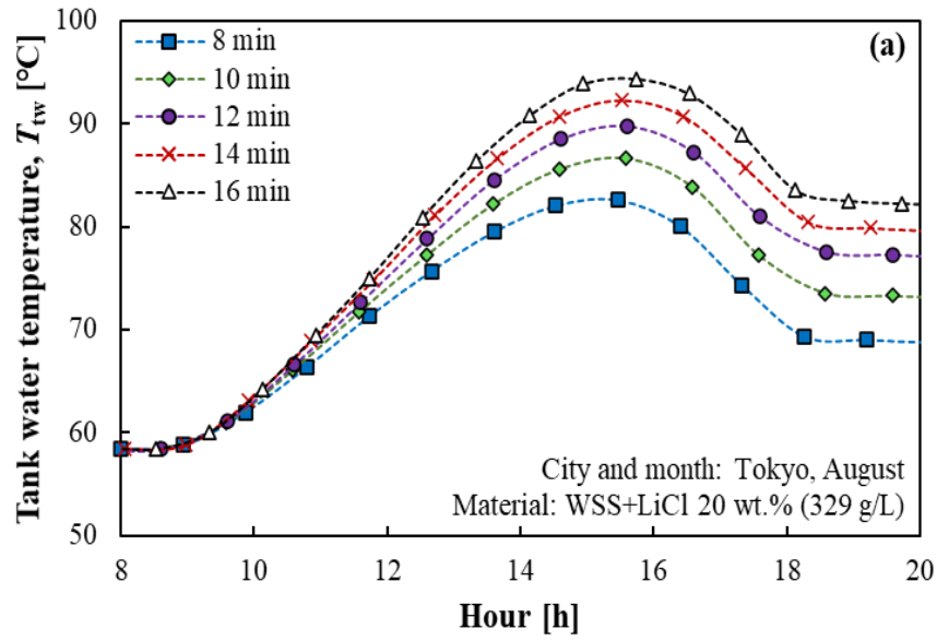
(a) Tank water temperature
