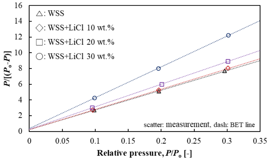
Fig. 2. 4 Typical B.E.T plot presenting straight line (Pure WSS and composites)
