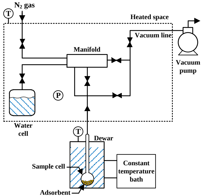
Fig. 2. 10 Schematic diagram of Quantachrome HYDROSORB 1000 [19]
