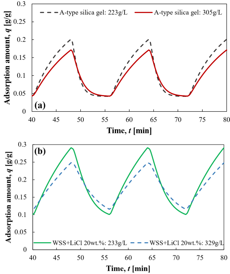
Fig. 4. 16 Comparison of adsorption amount according to filled density: (a) A-type silica gel, (b) WSS+LiCl 20 wt.%
