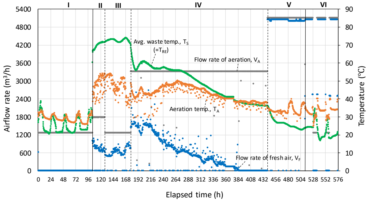
Figure 3-15 Profiles of operation variables of biocell reactor (BR-2) from 9/11/2017 to 10/5/2018
