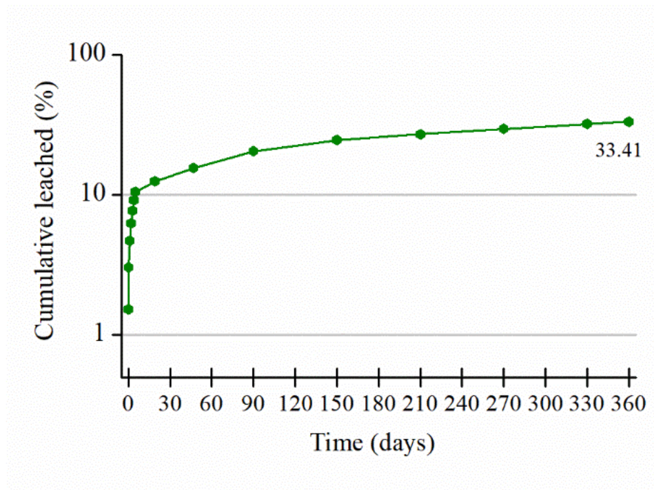
Figure 4-10 Cumulative leaching of \text{Cs}^+ from ordinary Portland cement with titanate adsorbent
