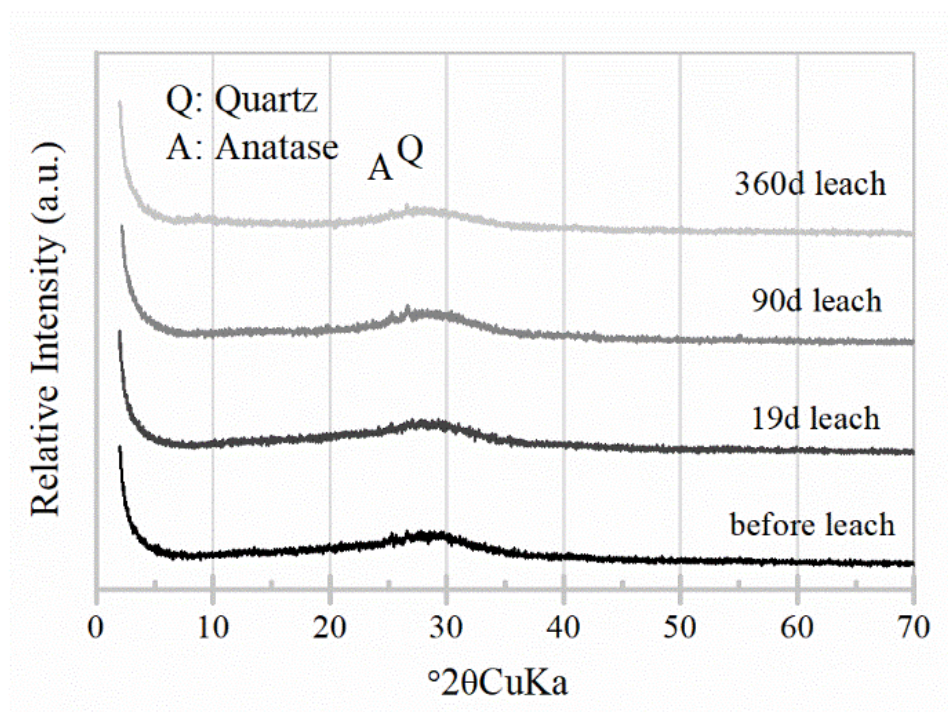
Figure 3-17 XRD patterns of K-geopolymer loaded Sr without spent titanate adsorbent before and after leaching for different durations as marked
