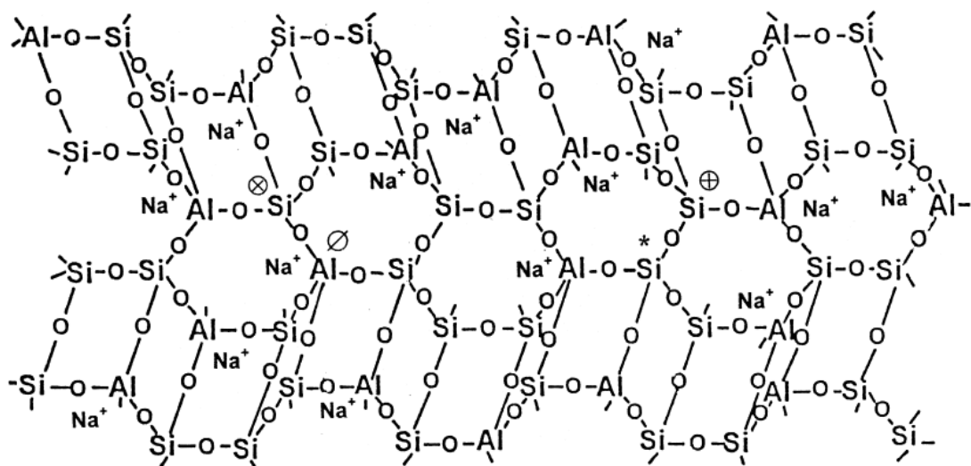
Figure 2-2 Three-dimensional framework structure for Na-polysialate polymer (Barbosa et al., 2000)
