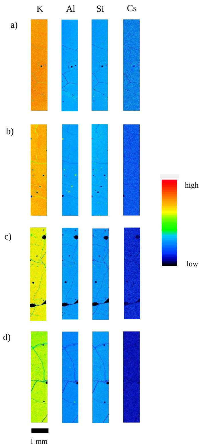
Figure 4-9 EPMA elemental maps of geopolymer specimens loaded Cs without titanate adsorbent; a) before, and after b) 19 days, c) 90 days, and d) 360 days of leaching in deionized
