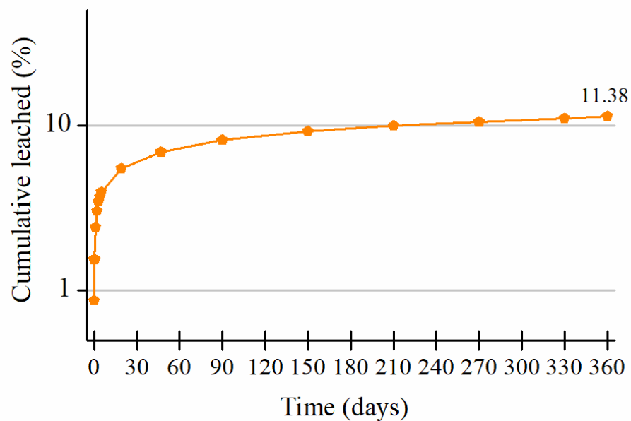
Figure 4-7 Cumulative leaching of \text{Cs}^+ from geopolymer without titanate adsorbent
