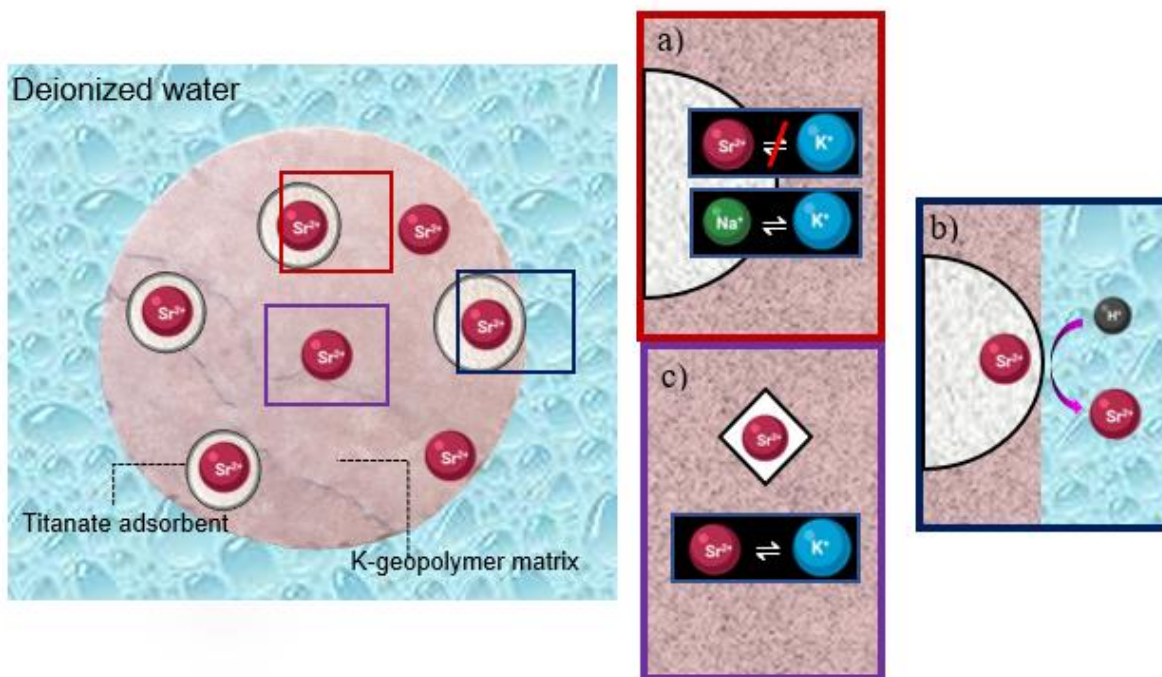
Figure 3-26 Schematic diagram of geopolymer matrix encapsulated titanate adsorbent adsorbed strontium, the interaction where a) between titanate adsorbent and geopolymer matrix inside specimen, b) the edge between titanate adsorbent and deionized water, c) geopolymer binder area
