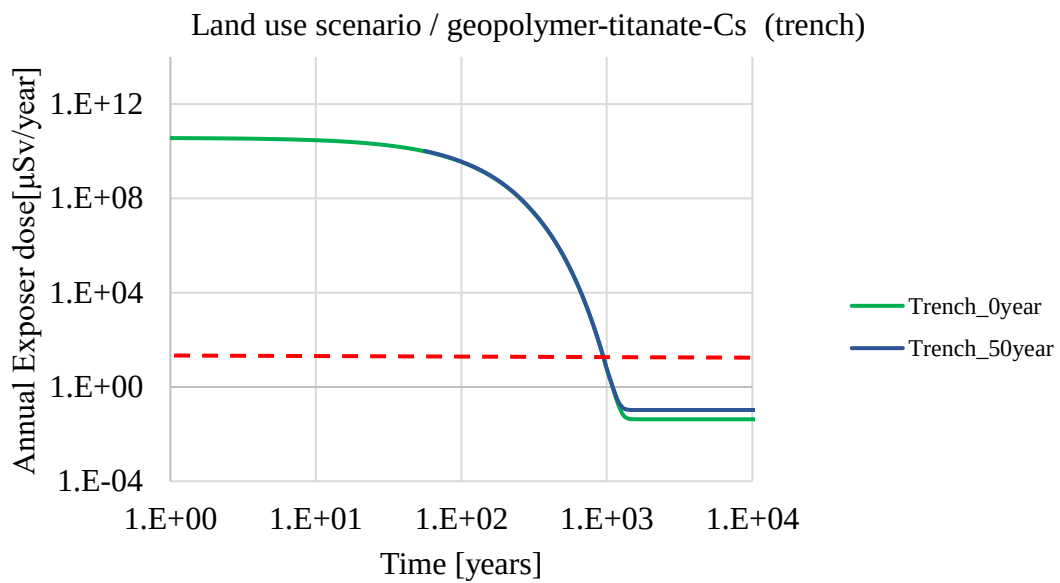
Figure 5-9 Annual radiation dose ( \mu\text{Sv/year} ) against time (years) of a geopolymertitanate-Cs specimen in the land use scenario for trench disposal
