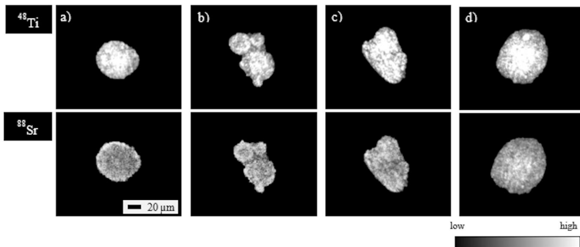
Figure 3-15 ^{48}\text{Ti} and ^{88}\text{Sr} isotope maps surrounding a titanate adsorbent particle in geopolymer specimens a) before, and after b) 19 days, c) 90 days, and d) 360 days of leaching in deionized water
