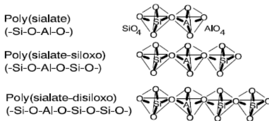
Figure 2-1 Geopolymer terminology (Davidovits, 1994)
