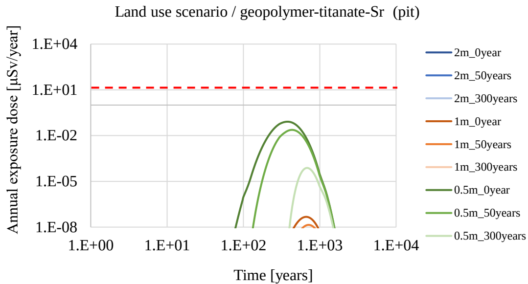
Figure 5-4 Annual radiation dose ( \mu\text{Sv}/\text{year} ) against time (years) of a geopolymer-titanate-Sr specimen in the land use scenario for pit disposal
