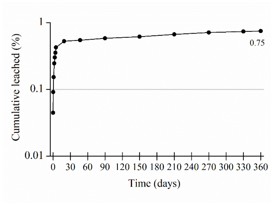
Figure 3-12 Cumulative leaching of \text{Sr}^{2+} from geopolymer mixed with titanate adsorbent, applying the ANSI/ANS 16.1 test method with full replacement of leachate at each sampling point shown
