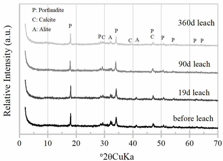
Figure 4-11 XRD patterns of ordinary Portland cement with spent titanate adsorbent loaded Cs before and after leaching for different durations as marked
