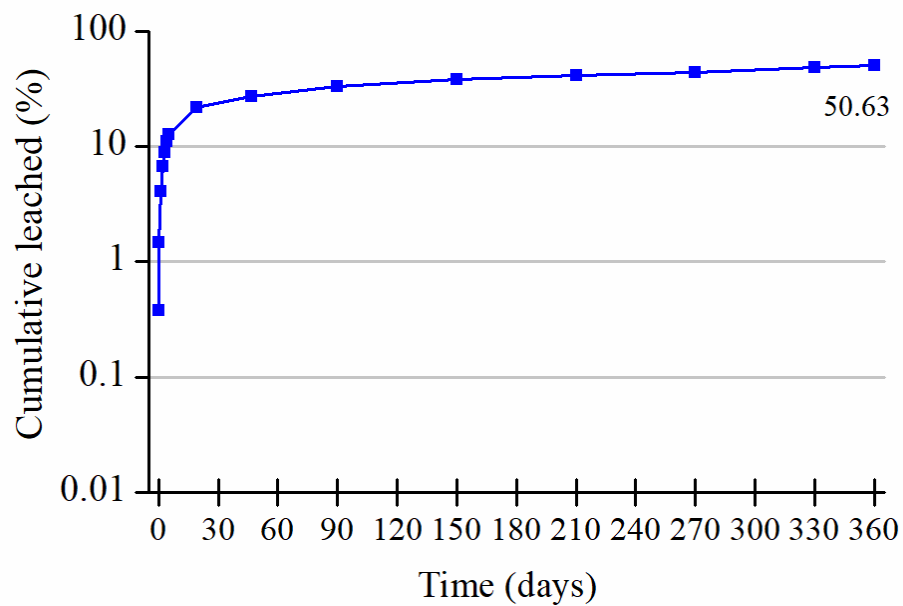
Figure 3-22 Cumulative leaching of \text{Sr}^{2+} from ordinary Portland cement without titanate adsorbent
