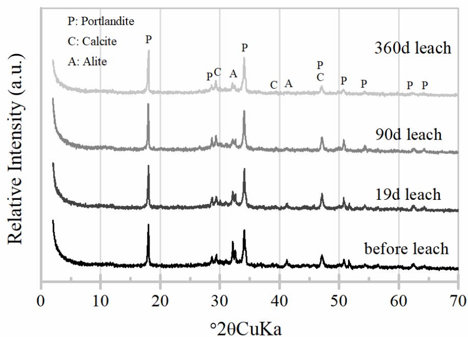
Figure 4-14 XRD patterns of ordinary Portland cement loaded Cs without spent titanate adsorbent before and after leaching for different durations as marked
