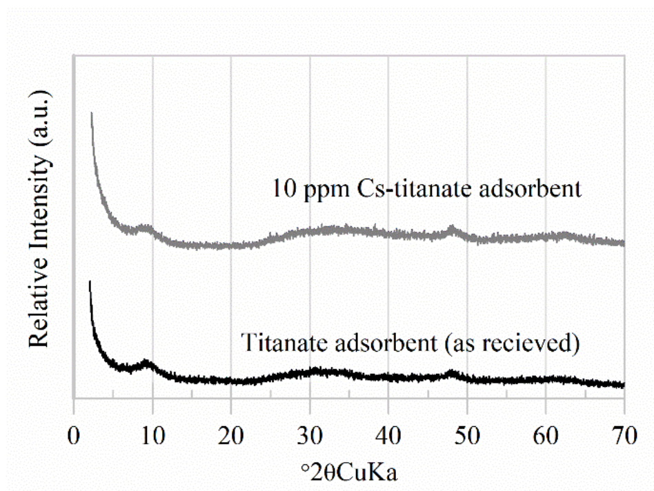
Figure 4-2 XRD patterns of titanate adsorbent before and after loading with Cs +
