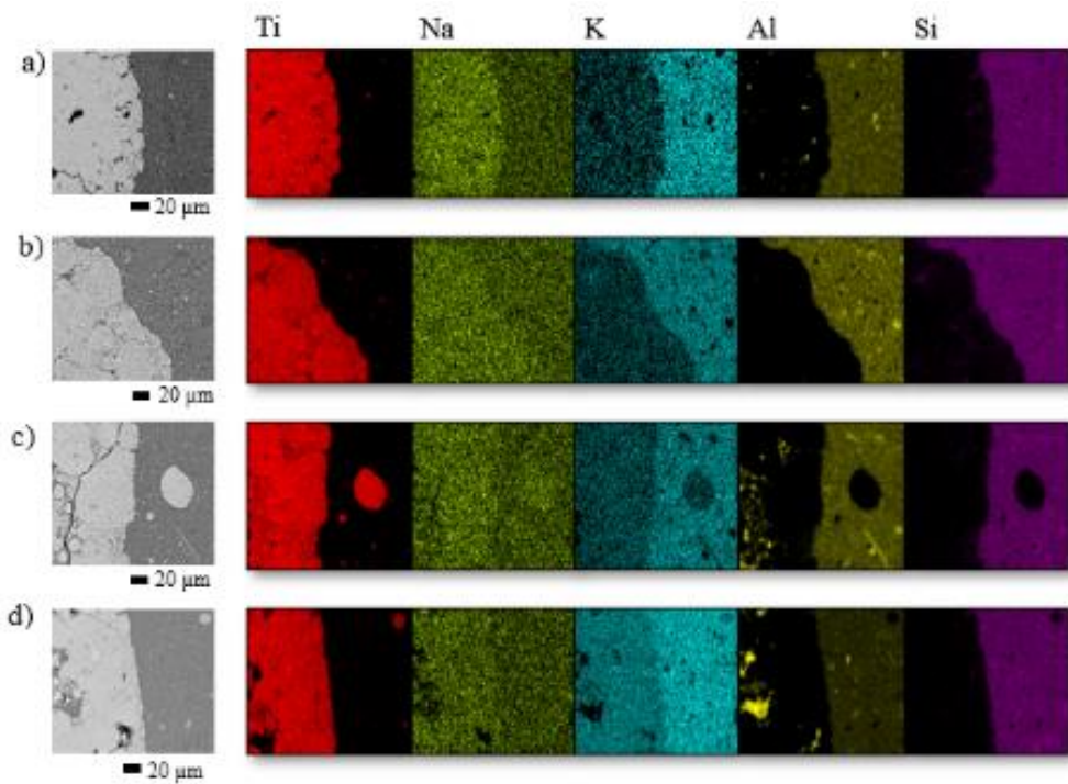
Figure 4-5 SEM images and elemental maps of geopolymer specimens with titanate adsorbent loaded Cs; a) before, and after b) 19days, c) 90days, and d) 360 days of leaching in deionized water
