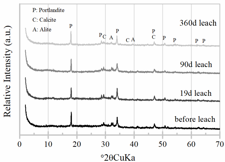
Figure 3-20 XRD patterns of ordinary Portland cement with spent titanate adsorbent loaded Sr before and after leaching for different durations as marked
