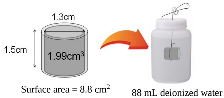
Figure 3-4 Schematic of leaching experiments
