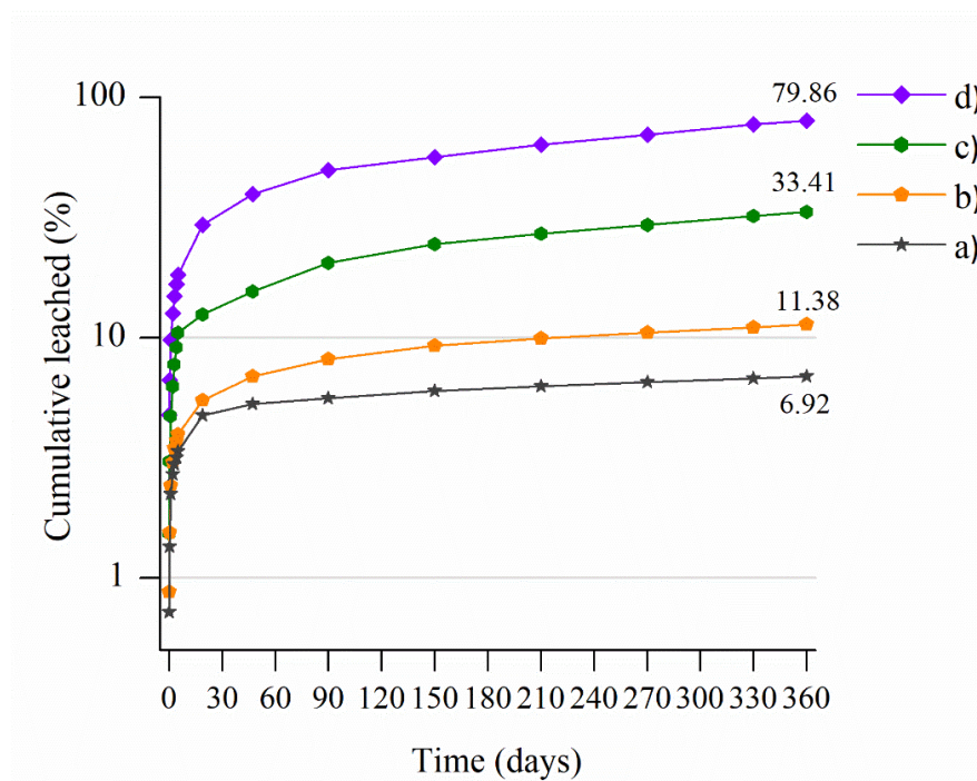
Figure 4-16 Cumulative leached percentage of \text{Cs}^+ from: a) geopolymer without adsorbent, b) geopolymer with adsorbent, c) cement with adsorbent, d) cement without adsorbent
