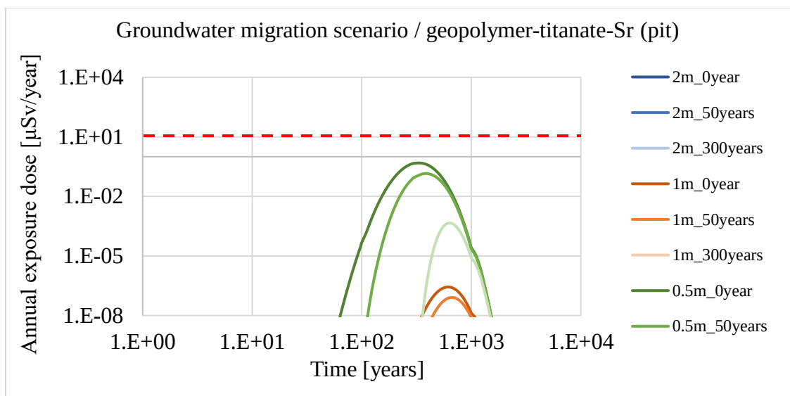
Figure 5-2 Annual radiation dose ( \mu\text{Sv}/\text{year} ) against time (years) of a geopolymers-titanate-Sr specimen in the groundwater migration scenario for pit disposal
