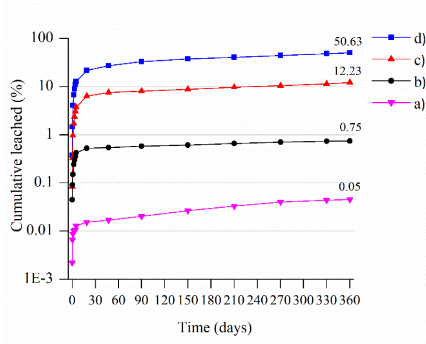
Figure 3-25 Cumulative leached percentage of \text{Sr}^{2+} from: a) geopolymer without adsorbent, b) geopolymer with adsorbent, c) cement with adsorbent, d) cement without adsorbent
