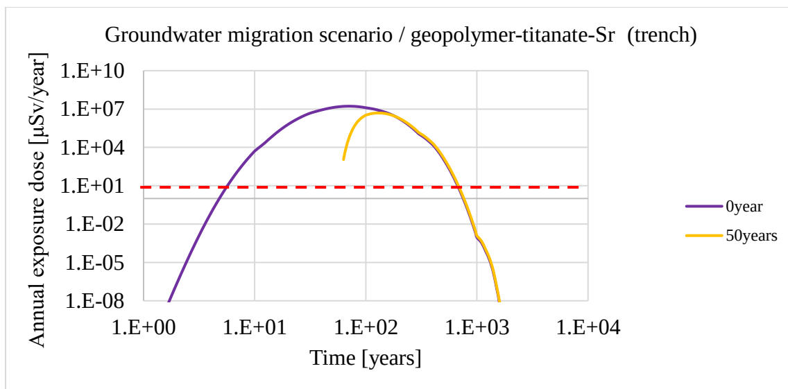
Figure 5-3 Annual radiation dose ( \mu\text{Sv}/\text{year} ) against time (years) of a geopolymers-titanate-Sr specimen in the groundwater migration scenario for trench disposal
