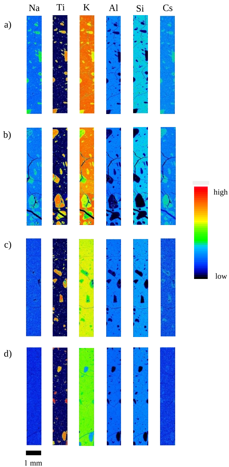
Figure 4-6 EPMA elemental maps of geopolymer specimens with titanate adsorbent loaded Cs; a) before, and after b) 19 days, c) 90 days, and d) 360 days of leaching in deionized water
