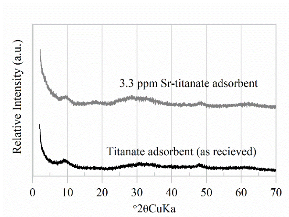
Figure 3-11 XRD patterns of titanate adsorbent before and after loading with \text{Sr}^{2+}
