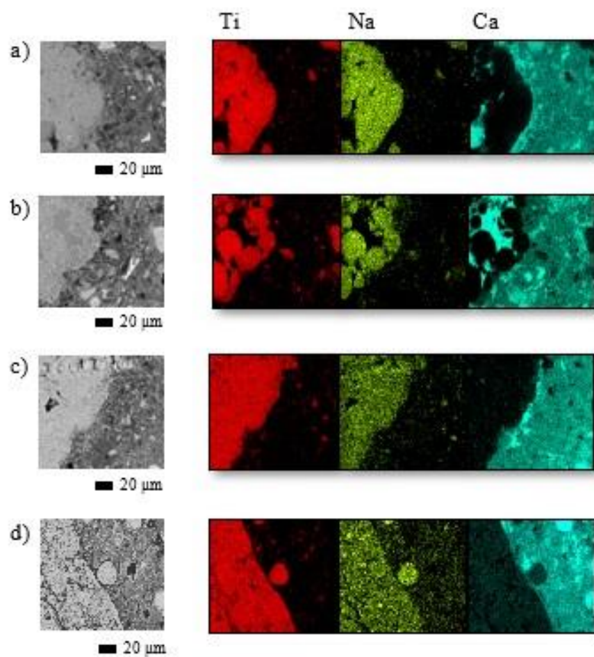
Figure 3-21 SEM images and elemental maps of ordinary Portland cement specimens with titanate adsorbent loaded Sr; a) before, and after b) 19days, c) 90days, and d) 360 days of leaching in deionized water
