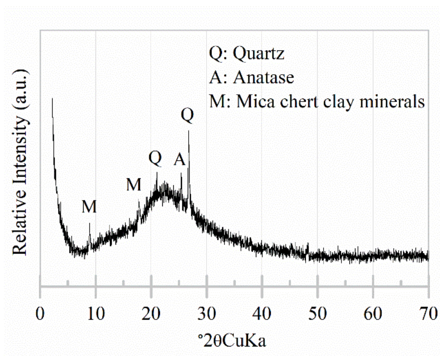
Figure 3-2 XRD pattern of the metakaolin precursor
