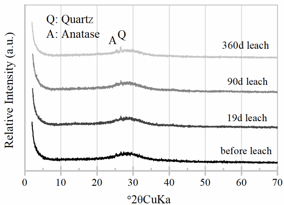
Figure 4-8 XRD patterns of K-geopolymer loaded Cs without spent titanate adsorbent before and after leaching for different durations as marked
