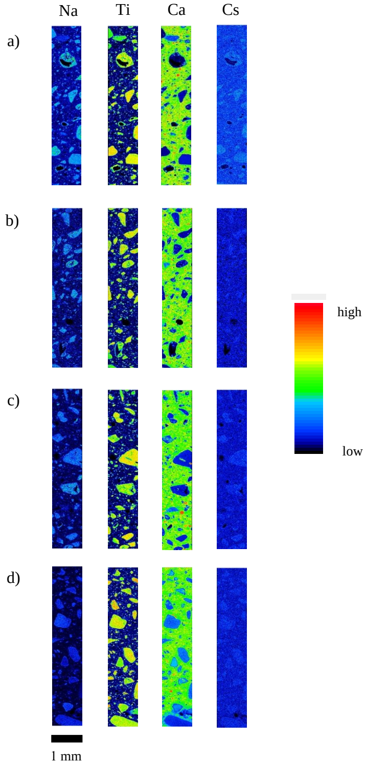
Figure 4-12 EPMA elemental maps of ordinary Portland cement specimens with titanate adsorbent loaded Cs; a) before, and after b) 19days, c) 90days, and d) 360 days of leaching in deionized water
