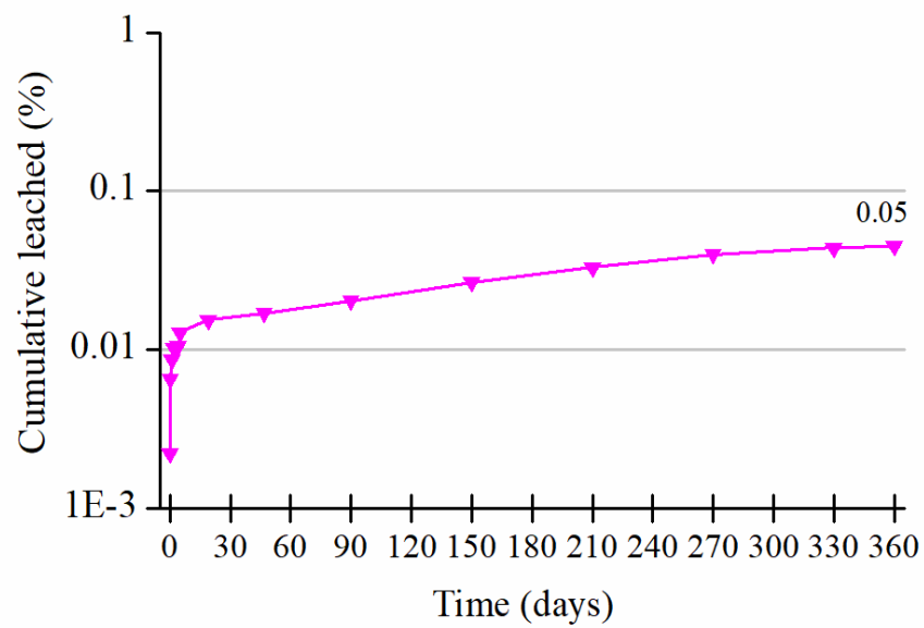
Figure 3-16 Cumulative leaching of \text{Sr}^{2+} from geopolymer without titanate adsorbent
