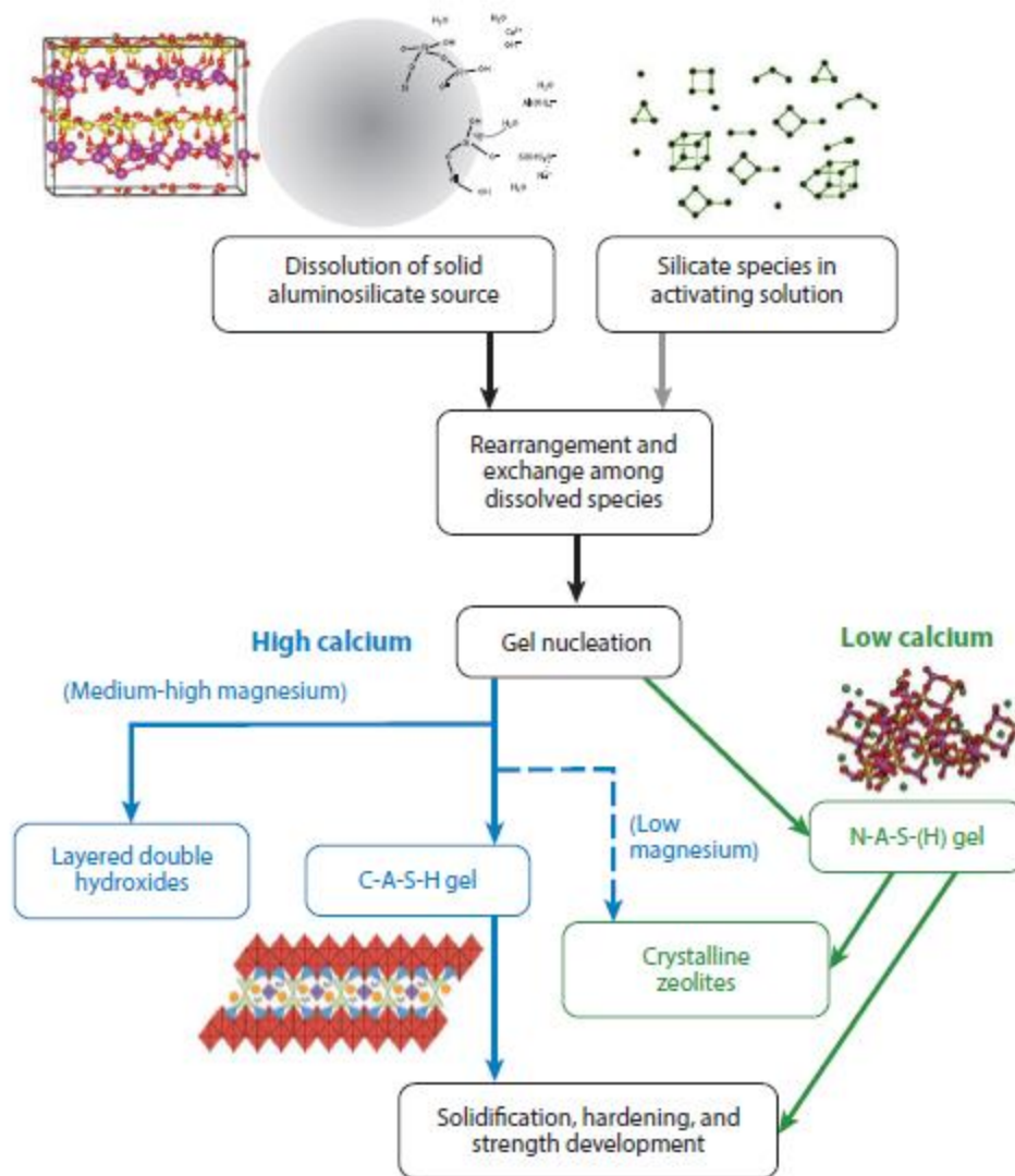
Figure 2-4 Process and reaction products of alkaline activation of a solid aluminosilicate precursor (Provis and Bernal, 2014)
