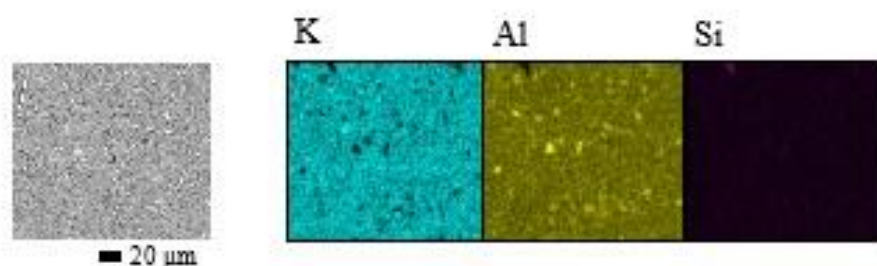
Figure 3-18 SEM images and elemental maps of geopolymer specimens loaded Sr without titanate adsorbent before leaching in deionized water
