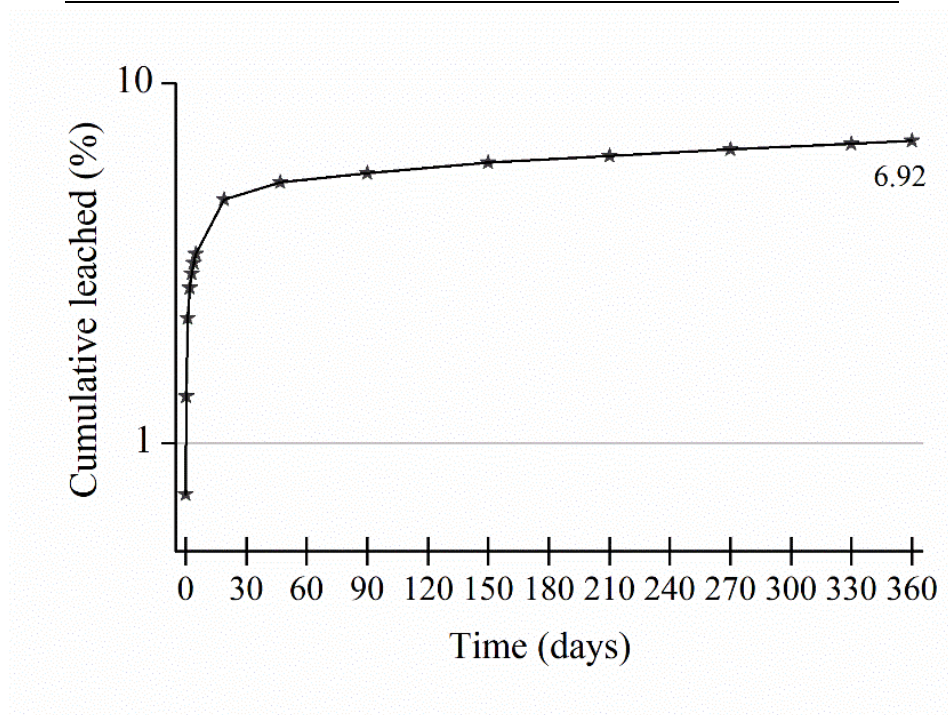
Figure 4-3 Cumulative leaching of \text{Cs}^+ from geopolymer mixed with titanate adsorbent, applying the ANSI/ANS 16.1 test method with full replacement of leachate at each sampling point shown
