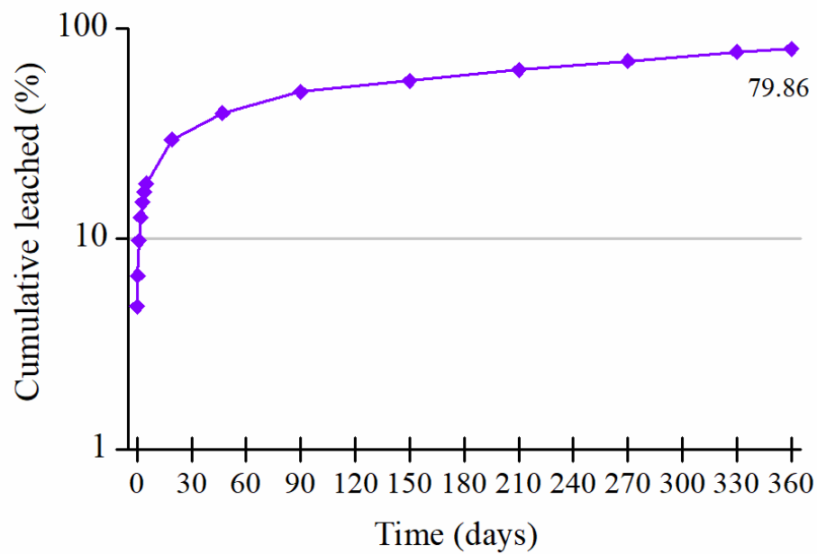
Figure 4-13 Cumulative leaching of \text{Cs}^+ from ordinary Portland cement without titanate adsorbent
