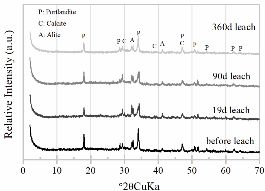
Figure 3-23 XRD patterns of ordinary Portland cement loaded Sr without spent titanate adsorbent before and after leaching for different durations as marked
