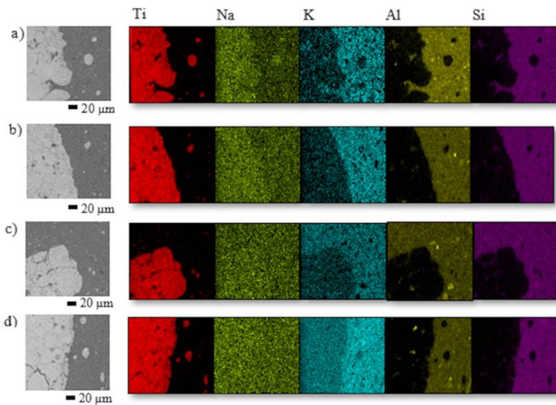
Figure 3-14 SEM images and elemental maps of geopolymer specimens with titanate adsorbent loaded Sr; a) before, and after b) 19days, c) 90days, and d) 360 days of leaching in deionized water
