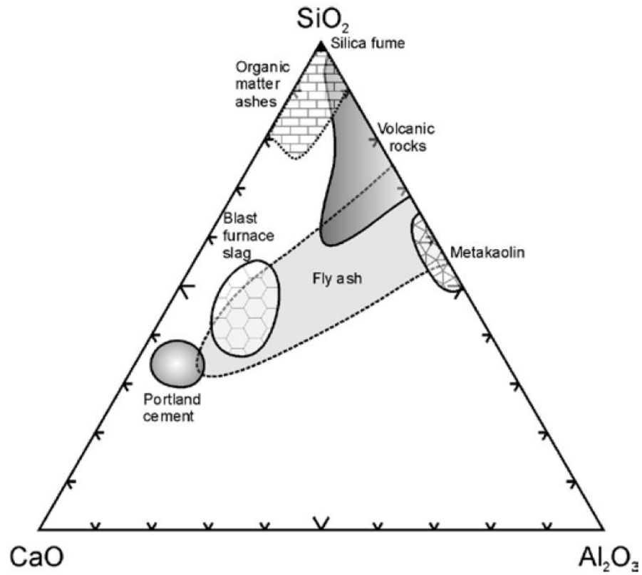
Figure 2-5 Ternary \text{CaO} - \text{SiO}_2 - \text{Al}_2\text{O}_3 diagram (wt%) of the major cementitious materials (Snellings et al., 2012)
