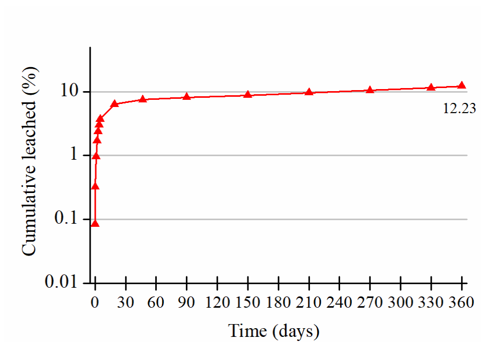
Figure 3-19 Cumulative leaching of \text{Sr}^{2+} from ordinary Portland cement with titanate adsorbent
