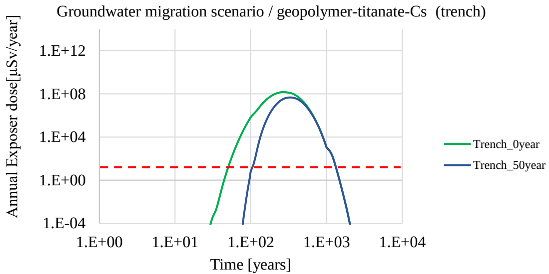
Figure 5-7 Annual radiation dose ( \mu\text{Sv/year} ) against time (years) of a geopolymertitanate-Cs specimen in the groundwater migration scenario for trench disposal
