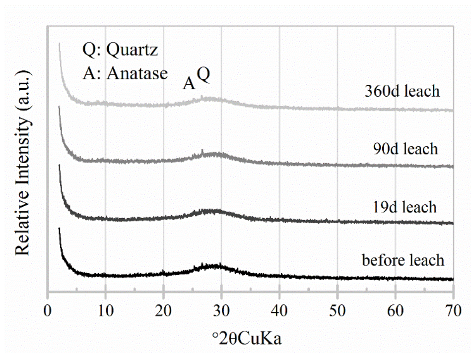
Figure 4-4 XRD patterns of K-geopolymer with spent titanate adsorbent loaded Cs before and after leaching for different durations as marked
