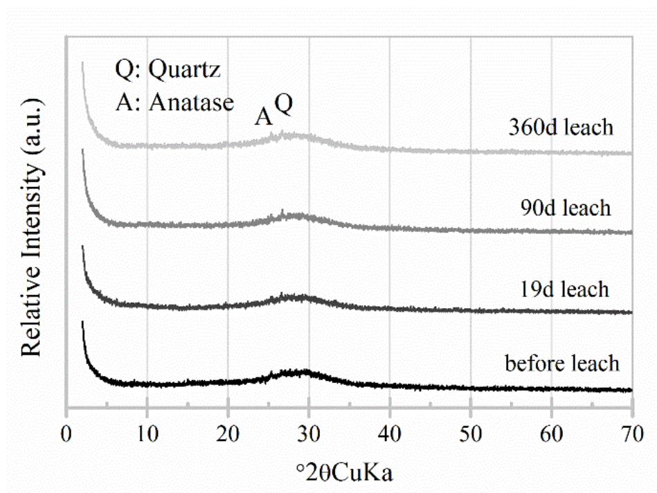
Figure 3-13 XRD patterns of K-geopolymer with spent titanate adsorbent loaded Sr before and after leaching for different durations as marked
