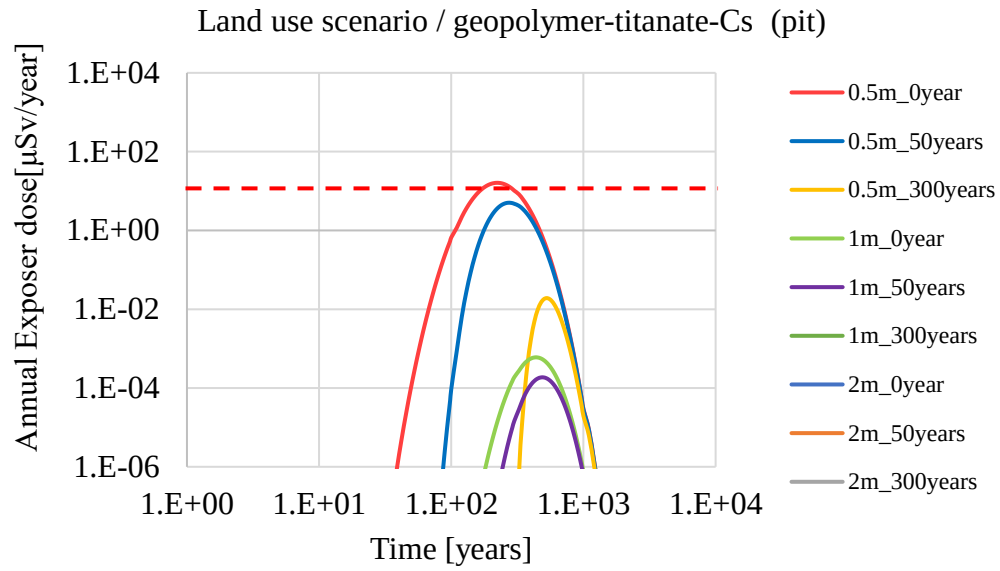
Figure 5-8 Annual radiation dose ( \mu\text{Sv/year} ) against time (years) of a geopolymertitanate-Cs specimen in the land use scenario for pit disposal
