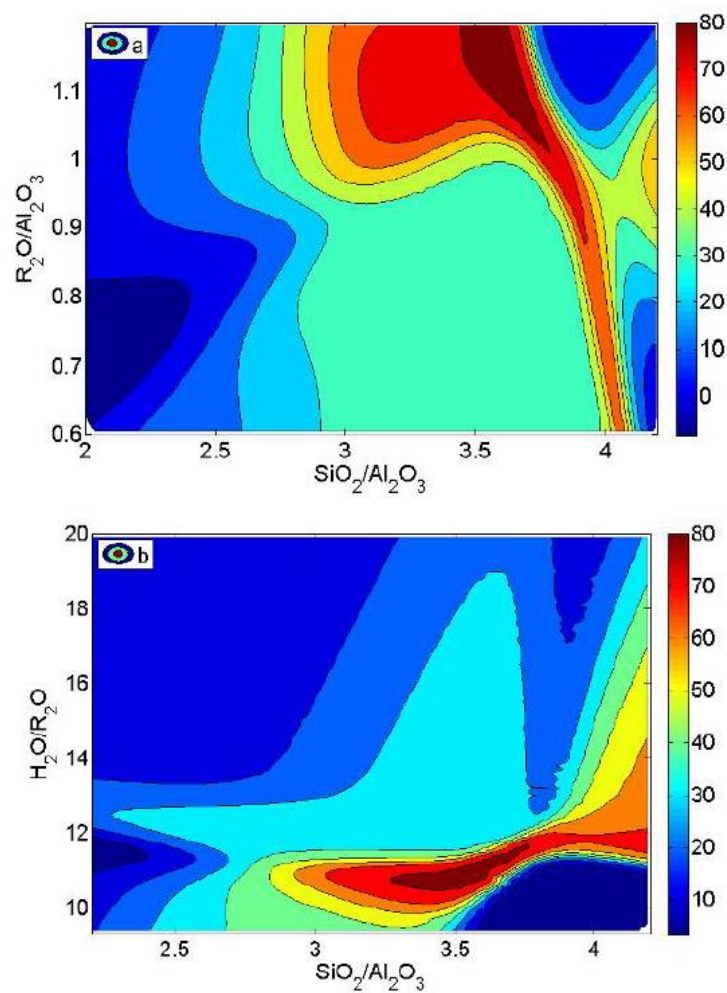
Figure 2-6 Filled contours plot of compressive strength (MPa) showing the effect of R_2O/Al_2O_3 (where R=Na or K), SiO_2/Al_2O_3 , and H_2O/R_2O molar ratios (Kamalloo et al., 2010)
