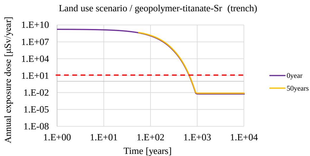
Figure 5-5 Annual radiation dose ( \mu\text{Sv}/\text{year} ) against time (years) of a geopolymer-titanate-Sr specimen in the land use scenario for trench disposal
