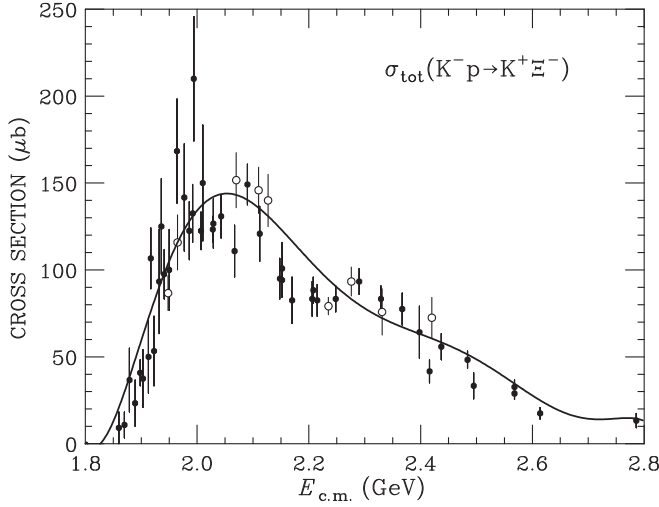
FIG. 2. Total cross section \sigma_{\text{tot}} for the K^-p \rightarrow K^+\Xi^- reaction as a function of the energy E_{\text{c.m.}} . The data are taken from the compilation of Flaminio et al. [20]. Open and solid circles denote the data for \sigma_{\text{tot}} with and without the measurements of d\sigma/d\Omega shown in Fig. 1, respectively.
