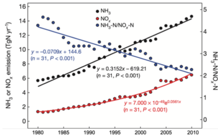
Fig. 1-4 Annual trends in the emission of \text{NH}_3 and \text{NO}_x and the ratios of \text{NH}_3\text{-N} to \text{NO}_x\text{-N} emission in China (Liu et al. 2013, the figure was partially modified).
