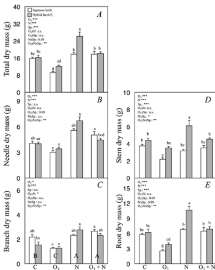
Fig. 3-1-1 Responses of dry mass at a whole plant level to O 3 and N loading.
