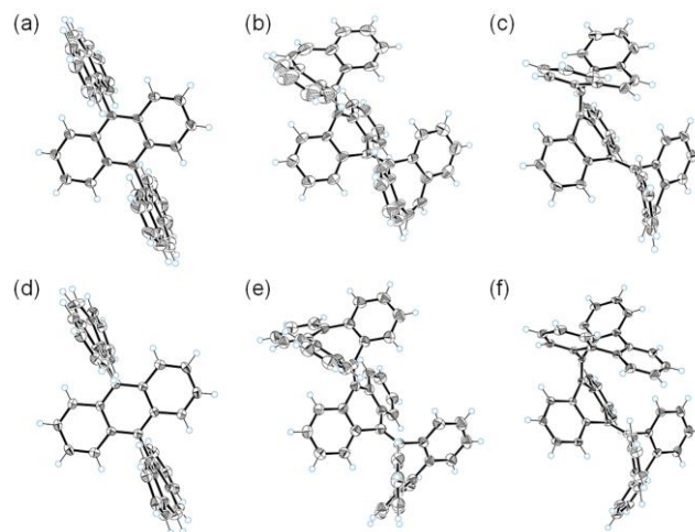
Figure 2. ORTEP drawings of (a) 1 2+ (BF 4 − ) 2 , (b) AA-1, (c) SA-1, (d) 1 2+ (SbCl 6 − ) 2 , (e) AA-2, and (f) SA-2. The counterions and solvent molecules are omitted for clarity. Thermal ellipsoids are shown at the 50% probability level.
