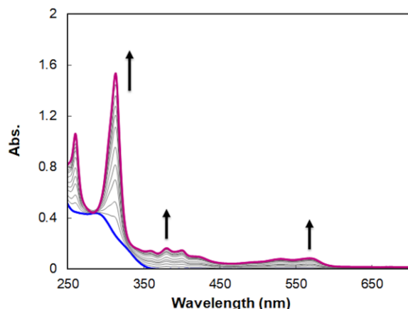
Figure 6. A change in the UV-vis spectrum of SA-1 (blue) to 1^{2+} (violet) upon constant current electrochemical oxidation (80 \mu A, every 2 min) in \text{CH}_2\text{Cl}_2/(\text{CF}_3)_2\text{CHOH} (9:1) containing 0.05 M \text{Bu}_4\text{NBF}_4 as a supporting electrolyte.
