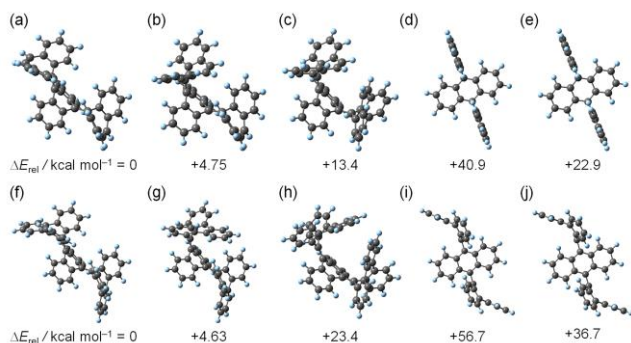
Figure 1. Optimized structures of (a) AA-1, (b) SA-1, (c) SS-1, (d) T-1, (e) TD-1 \cdot\cdot , (f) AA-2, (g) SA-2, (h) SS-2, (i) T-2, and (j) TD-2 \cdot\cdot based on DFT calculations at the (U)B3LYP/6-31G* level.
