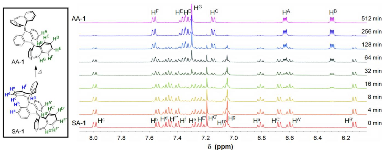
Figure 3. A change in ^1\text{H} NMR spectrum of SA-1 in \text{DMSO}-d_6 at 170^\circ\text{C} .
