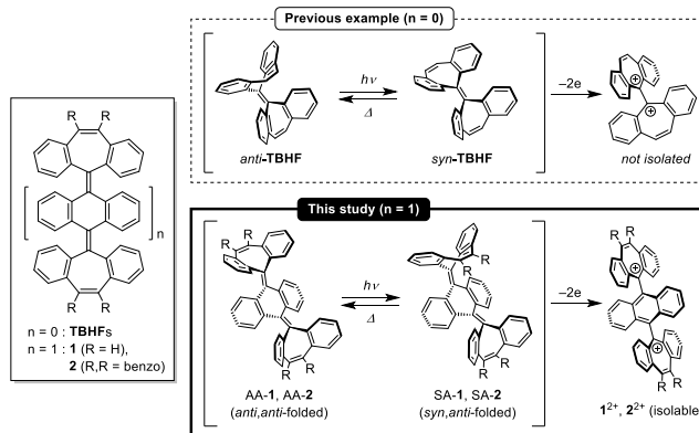
Scheme 1. Molecular design for 1 and 2 .
