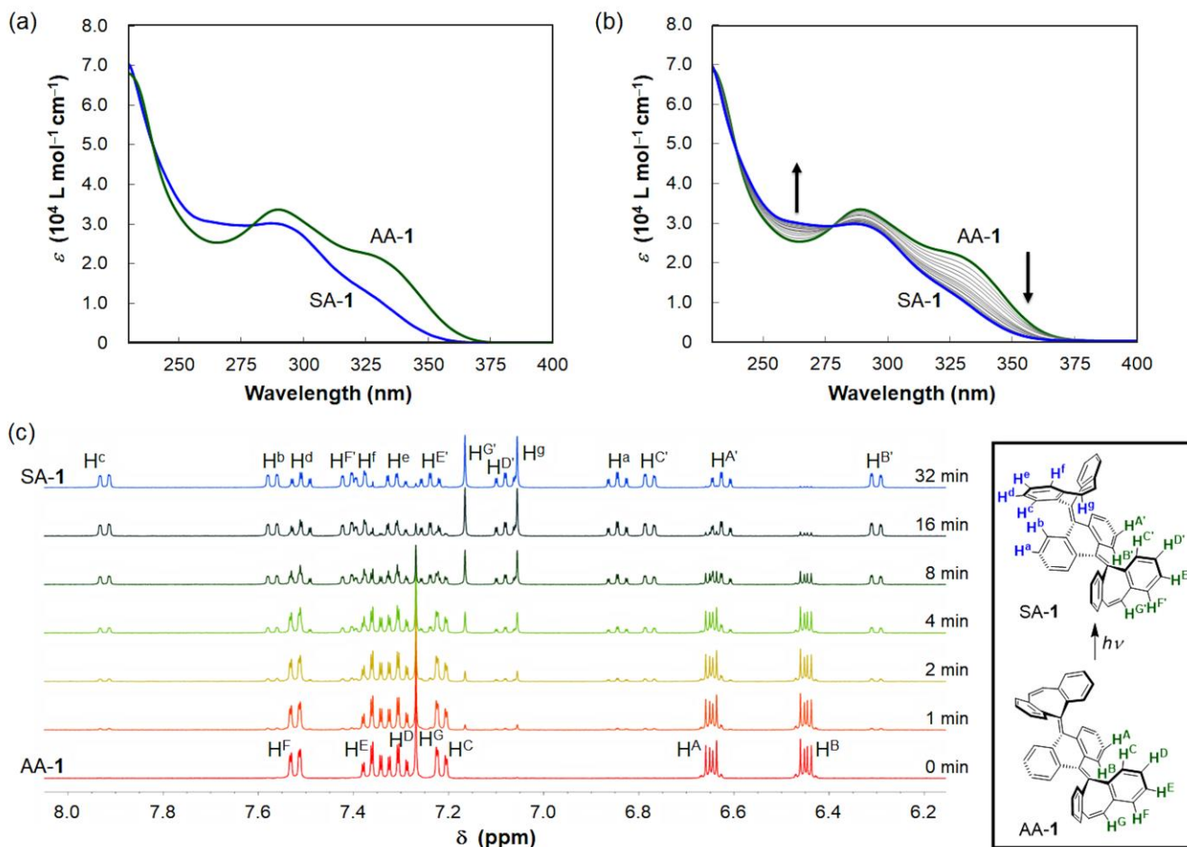
Figure 4. (a) UV-vis spectra of AA-1 (green) and SA-1 (blue) in CH 2 Cl 2 . (b) A change in UV-vis spectrum of AA-1 (green) to SA-1 (blue) in CH 2 Cl 2 (0-20 min, every 2 min; 20-40 min, every 4 min) and (c) a change in 1 H NMR spectrum of AA-1 in CD 2 Cl 2 upon photoirradiation at 365 nm [spectrofluorometer: 150 W Xe lamp, slit width (b) 5 nm and (c) 10 nm].
