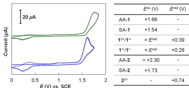
Figure 5. Cyclic voltammograms of AA-1 (green) and SA-1 (blue) in CH 2 Cl 2 containing 0.1 M Bu 4 NBF 4 as a supporting electrolyte (scan rate 0.5 V s -1 , Pt electrode). The second cycles are shown by dotted line. The redox potentials for these hydrocarbons are summarized in the table (scan rate 0.1 V s -1 ). The irreversible half-wave potentials were estimated from the anodic peak potentials ( E_{\text{pa}} ) as E^{\text{ox}} = E_{\text{pa}} - 0.03 or the cathodic peak potentials ( E_{\text{pc}} ) as E^{\text{red}} = E_{\text{pc}} + 0.03 .
