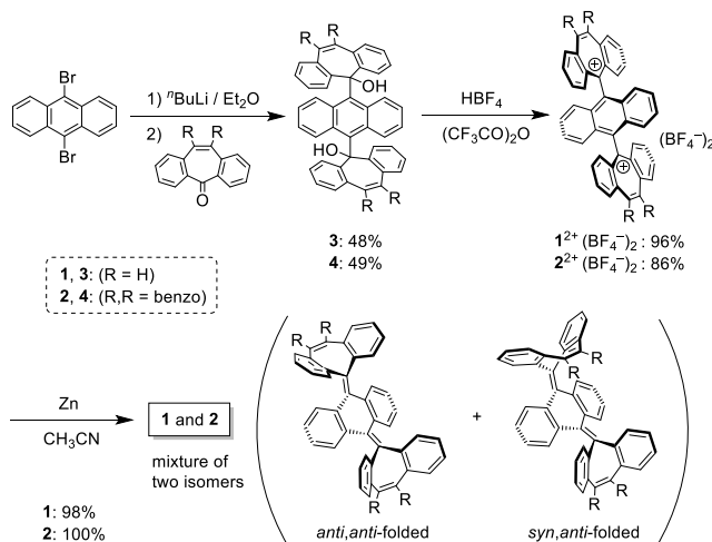
Scheme 2. Preparation scheme for 1 and 2 .
