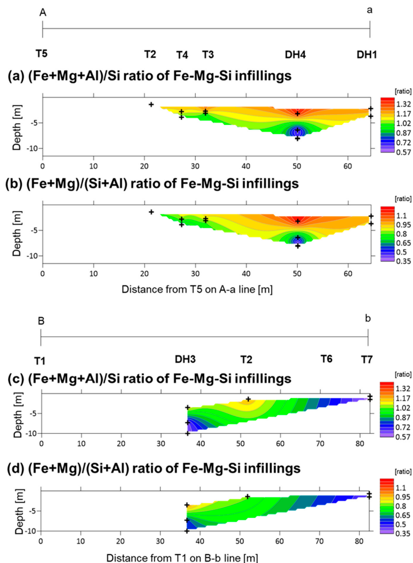
Figure 9. Distribution of the median of (\text{Fe} + \text{Mg} + \text{Al})/\text{Si} (panels a and c) and median of (\text{Fe} + \text{Mg})/(\text{Si} + \text{Al}) (panels b and d) ratios of the Fe-Mg-Si infillings along depth in the study areas: (a,b) section A-a; and (c,d) section B-b. Plus signs show the locations of the analyzed samples.
