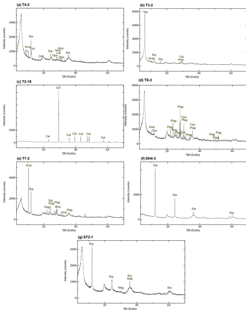
Figure A1. XRD profile of randomly oriented samples: (a) T4-2; (b) T3-2; (c) T2-18; (d) T8-3; (e) T7-2; (f) DH4-3; (g) ST2-1; Srp—serpentine; Opx—orthopyroxene; Amp—amphibole; Tc—talch; Chl: chlorite; Cal—calcite; Tob—14 Å tobermorite; Plag—plagioclase; Cpx—clinopyroxene; Mag—magnetite.
