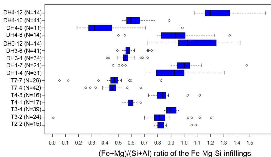
Figure A4. The (\text{Fe} + \text{Mg})/(\text{Si} + \text{Al}) ratio of Fe-Mg-Si inclusions in each sample. Results are expressed as box and whisker plots. Legends are the same as for Figure A3.
