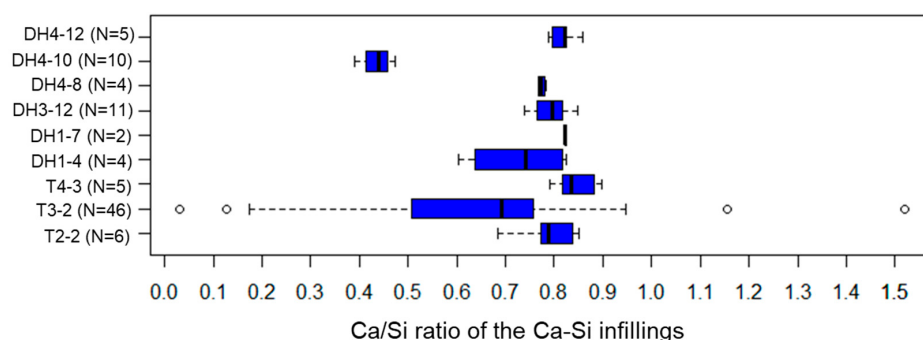
Figure A5. The Ca/Si ratio of Ca-Si inclusions in each sample. Results are expressed as box and whisker plots. Legends are the same as for Figure A3.
