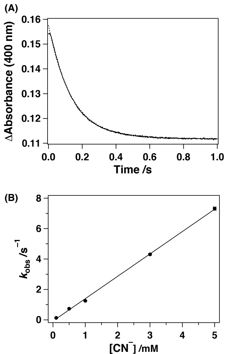
Figure S4. Cyanide binding to the ferric heme-Arg92 HutZ mutants. (A) Typical time course of absorbance changes at 400 nm upon mixing 5 \mu\text{M} protein with 1 mM cyanide in 50 mM Tris-HCl and 150 mM NaCl (pH 8.0). (B) Plots of calculated k_{\text{obs}} versus cyanide concentration.
