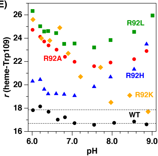
Fig. 8. Fluorescence spectra of the ferric (A) R92A, (B) R92L, (C) R92H and (D) R92K mutant HutZ s in the absence (blue lines) and presence of heme (red lines) at pH 6.0–9.0. Spectra were recorded with excitation at 295 nm. The sample concentration was 3 \mu\text{M} . (E) pH dependence of the distance between heme and Trp109 estimated by quenching of tryptophan fluorescence by energy transfer efficiency and the Förster distance using equation 2.
