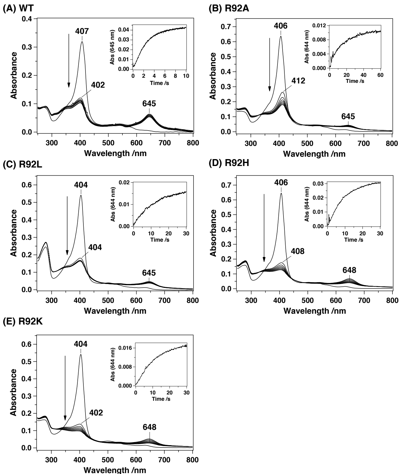
Fig. 7. Heme degradation reaction of the heme-Arg92 HutZ mutants with \text{H}_2\text{O}_2 (0.2 mM) in 50 mM sodium phosphate and 150 mM NaCl (pH 6.0). Spectra were recorded before the addition of \text{H}_2\text{O}_2 and at 1-min intervals for 15 min after the addition of ascorbic acid: (A) heme-WT, (B) heme-R92A, (C) heme-R92L, (D) heme-R92H, and (E) heme-R92K. The insets show the time course of absorbance at 644 nm after the addition of \text{H}_2\text{O}_2 obtained by stopped-flow method.
