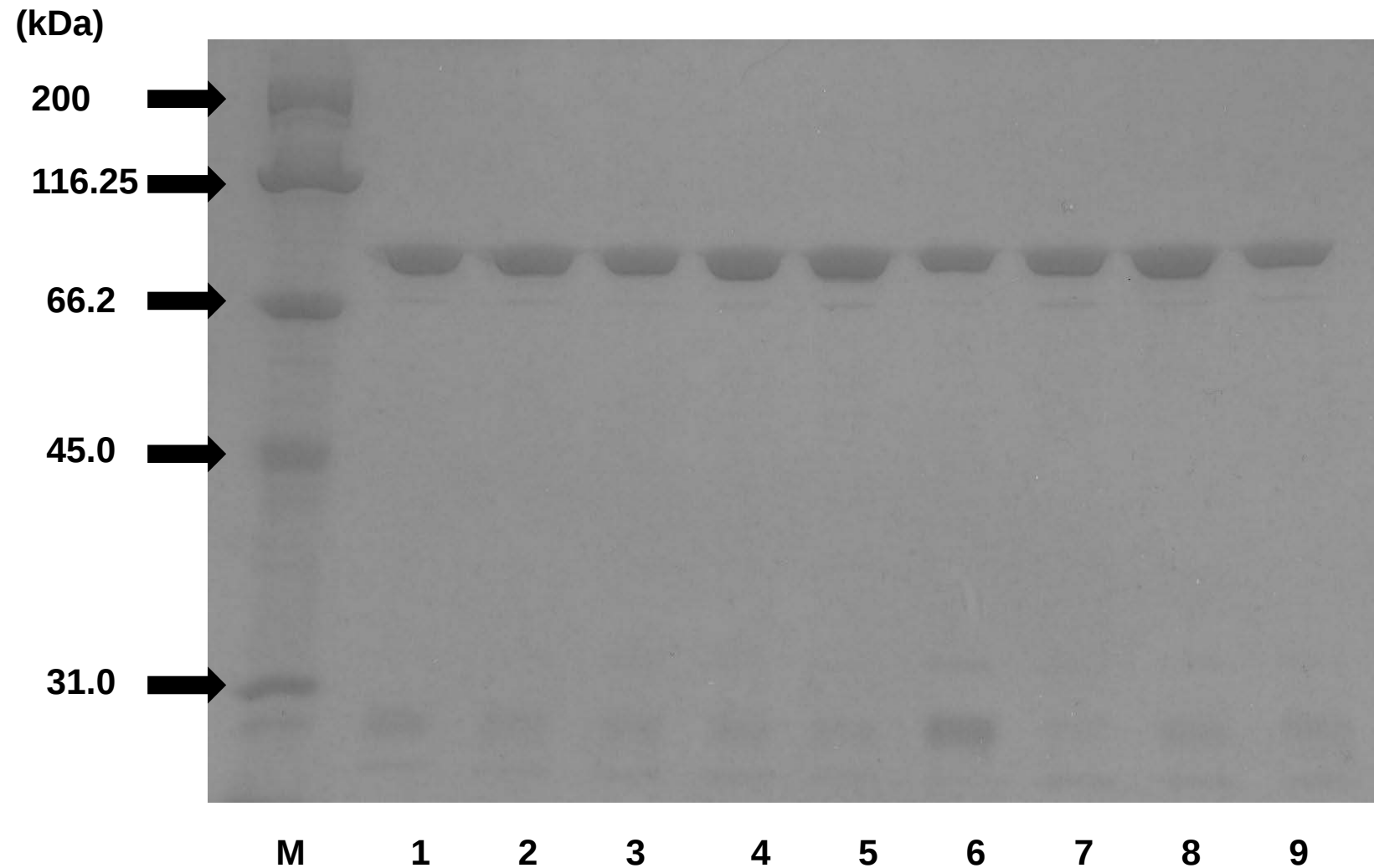
Supplementary Fig. S3 SDS-PAGE of the wild-type and mutated AvIDHs. Three \mu\text{g} of protein was applied to each lane. Lane M, marker proteins; lane 1, wild-type AvIDH; lane 2, AvY598H; lane 3, AvP624A; lane 4, AvL665M; lane 5, AvE676T; lane 6, AvP709A; lane 7, AvP718T; lane 8, AvF733L; lane 9, AvP739N.
