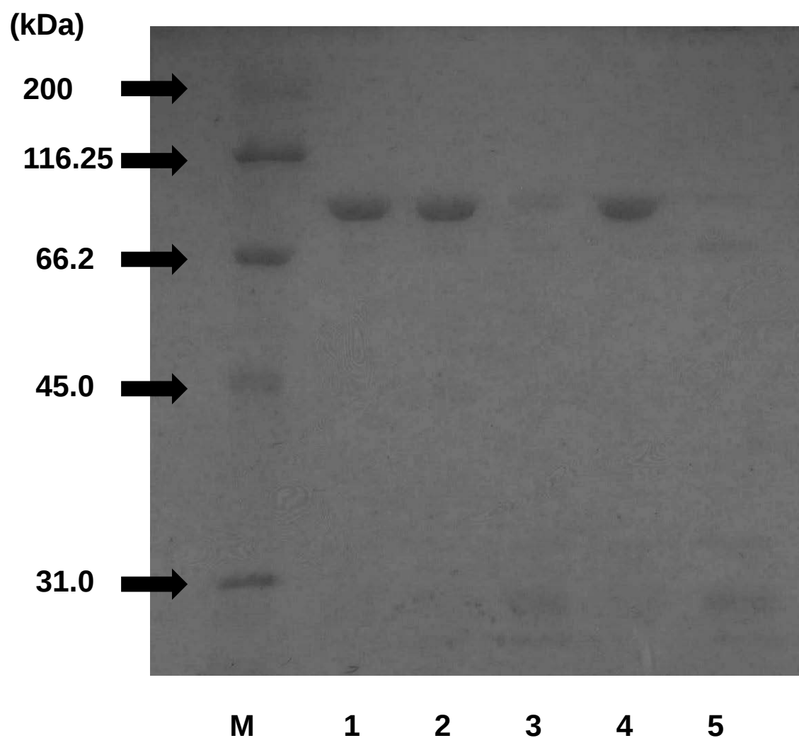
Supplementary Fig. S4 SDS-PAGE of the wild-type PmIDH and multiple mutants. Three \mu g of protein was applied to each lane. Lane M, marker proteins; lane 1, wild-type PmIDH ; lane 2, PmH600YL735F ; lane 3, PmH600YN741P ; lane 4, PmL735FN741P ; lane 5, PmH600YL735FN741P .
