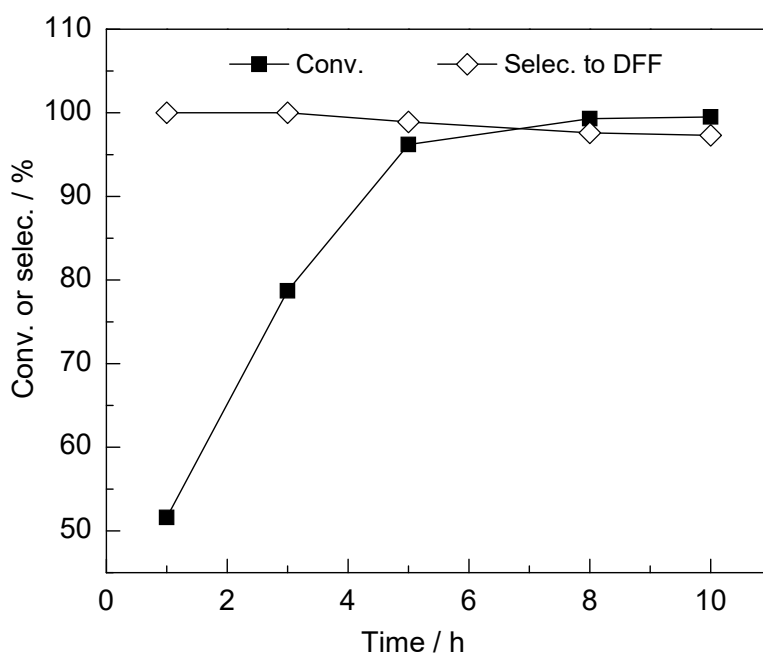
Fig. 4. HMF conversion and DFF selectivity on the FeN x /C-900 catalyst as a function of reaction time. Reaction conditions: HMF (0.25 mmol, 32 mg), (0.1 g), DMF (10 mL), 100 °C, and O 2 (0.5 MPa).
