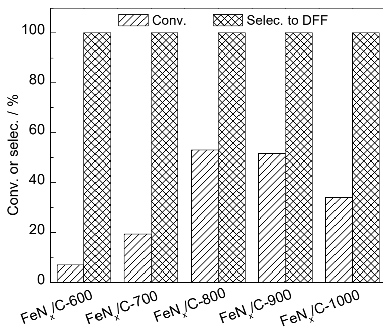
Fig. 2. HMF conversion and DFF selectivity on the FeN x /C- T catalysts by different pyrolysis temperatures. Reaction conditions: HMF (0.25 mmol, 32 mg), FeN x /C- T (0.1 g), DMF (10 mL), 100 °C, 1 h, and O 2 (0.5 MPa).
