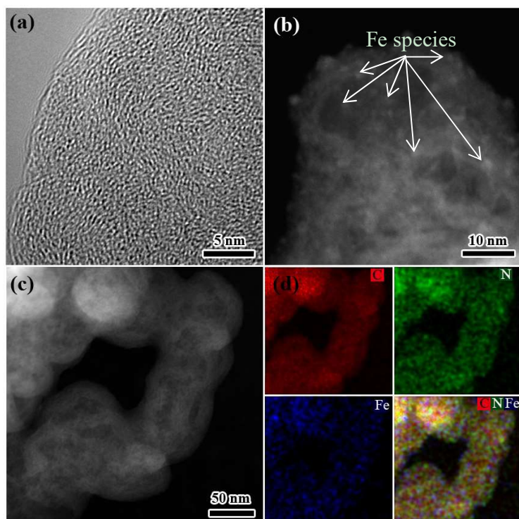
Fig. 1. TEM and HAADF-STEM images of FeN x /C-900. (a) bright-field image, (b) and (c) dark-field images, and (d) STEM mapping image.
