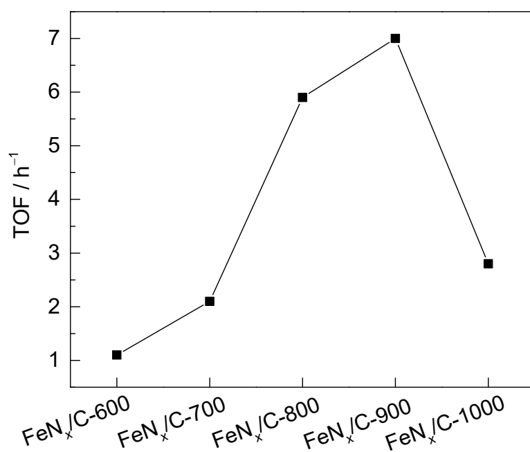
Fig. 3. The TOF value of HMF oxidation on the \text{FeN}_x/\text{C}-T catalysts by different pyrolysis temperatures.
