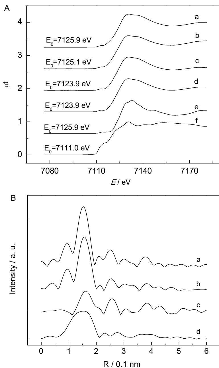
Fig. 8. (A) The normalized XAFS profiles and (B) the k^3 -weighted Fourier transform EXAFS profiles at Fe K-edge of different samples. (a) FeN x /C-900, (b) FeN x /C-800, (c) FeN x /C-700, (d) FeN x /C-600, (e) Fe 2 O 3 , and (f) Fe foil.
