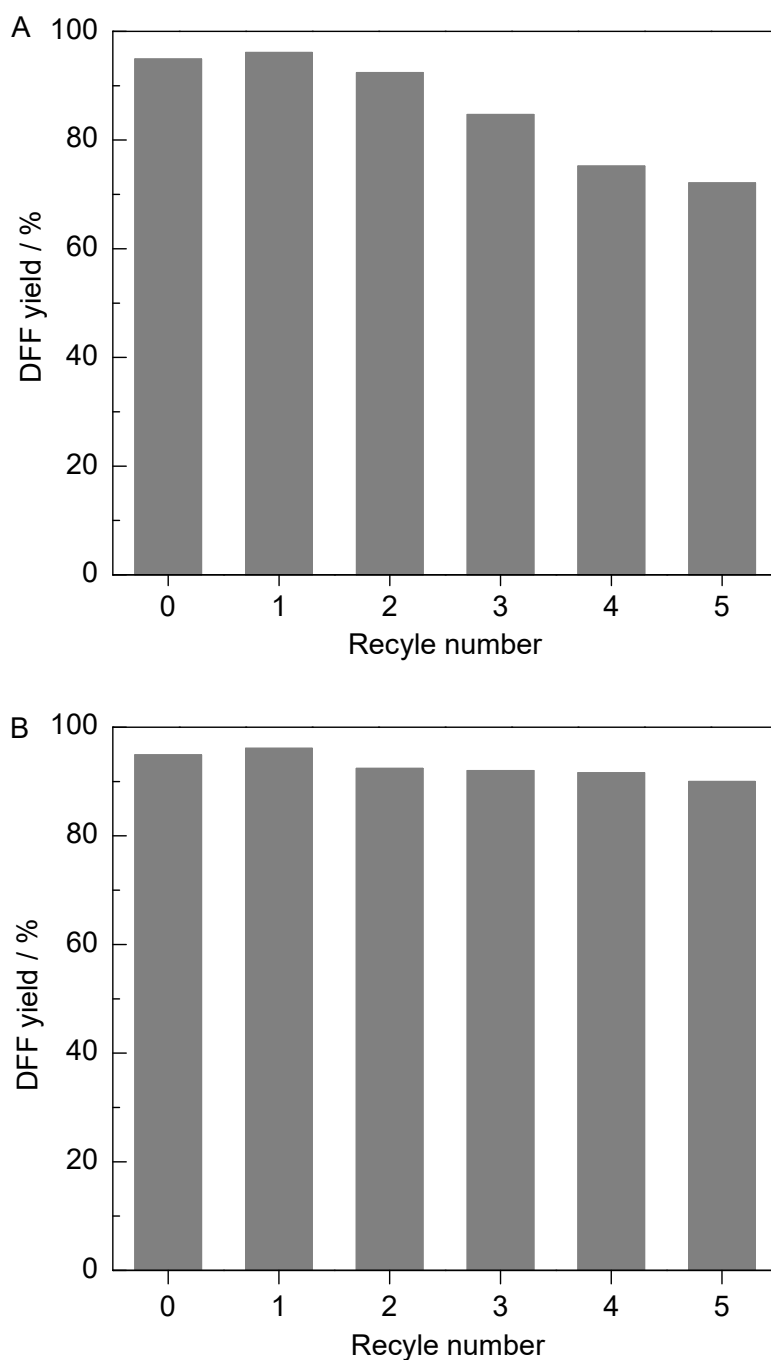
Fig. 9. Recycling results of the Fe N x /C-900 catalyst for the HMF oxidation. Reaction conditions: HMF (0.25 mmol, 32 mg), Fe N x /C-900 (0.1 g), DMF (10 mL), 100 °C, 5 h, and O 2 (0.5 MPa). (A) The Fe N x /C-900 catalyst was reused after calcination in N 2 at 900 °C for 1 h and (B) the Fe N x /C-900 catalyst after the 3rd run was calcined in 3%NH 3 /N 2 for 1 h at 900 °C and
