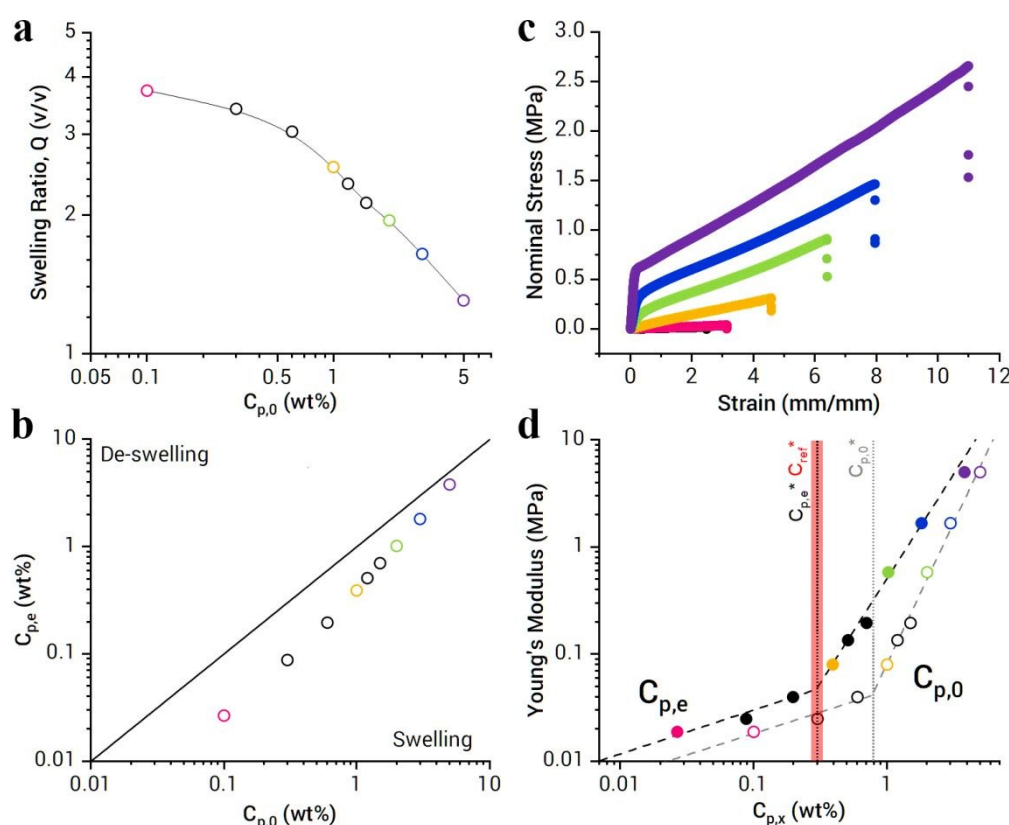
Figure 5. Influence of PBDT concentration. a) Swelling ratio versus as-prepared PBDT concentration. b) A plot comparing equilibrium and as-prepared concentration, C_{p,e} versus C_{p,0} , which demonstrates the relative swelling nature of each composition. As the PBDT concentration increases, swelling decreases. c) Stress-strain curves of PBDT/PAAm gels with different concentrations of PBDT in the hydrogel matrix. Colors correspond with the concentrations from a) and b). d) Relationship between Young's modulus of PBDT/PAAm gels and PBDT concentration, either C_{p,0} or C_{p,e} . The symbols represent the average of 3-5 samples and in all cases error bars are smaller than the symbol size. Red vertical band represents the literature overlap concentration, C_{ref}^* of PBDT. Vertical dotted black and gray lines represent the apparent critical concentrations of PBDT in either the equilibrium condition C_{p,e}^* or as-prepared condition C_{p,0}^* , respectively. Dashed trend lines are drawn as guides for the eye. All samples were equilibrated in 0.15 M ZrCl_2O solution.
