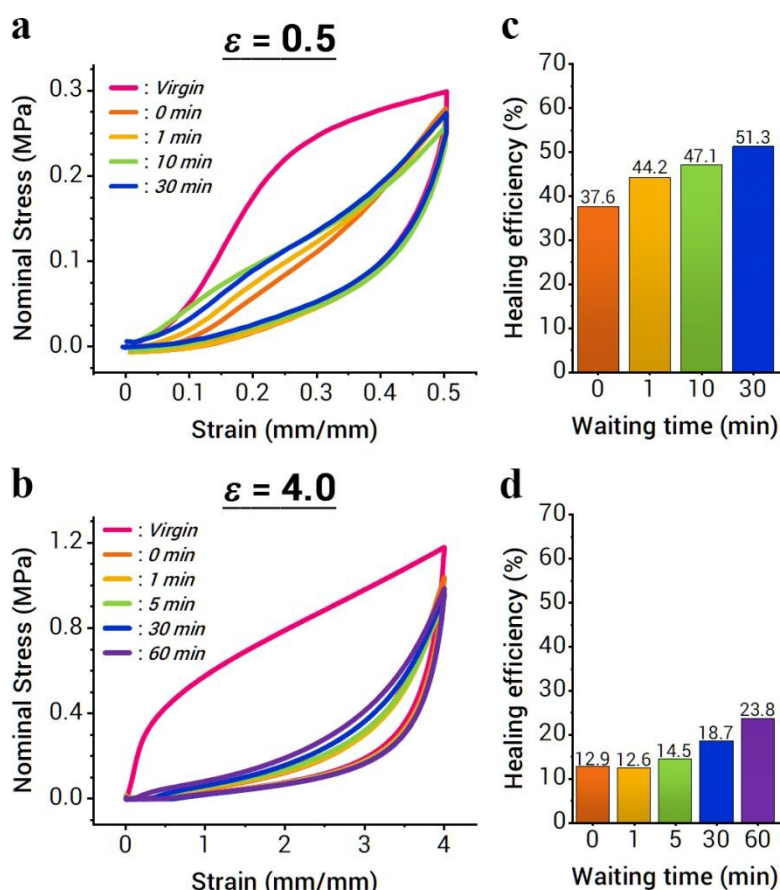
Figure 4. Cyclic loading / unloading test of the 3% PBDT/PAAm gels after equilibration in 0.15 M \text{ZrCl}_2\text{O} solution. Stress-strain curves for cycle testing at strains of (a) 0.5 or (b) 4.0 with different waiting times after testing. Healing efficiency at a maximum strain of (c) 0.5 and (d) 4.0 was estimated by comparing the mechanical hysteresis of the first cycle test to the cycle tests after various waiting times.
