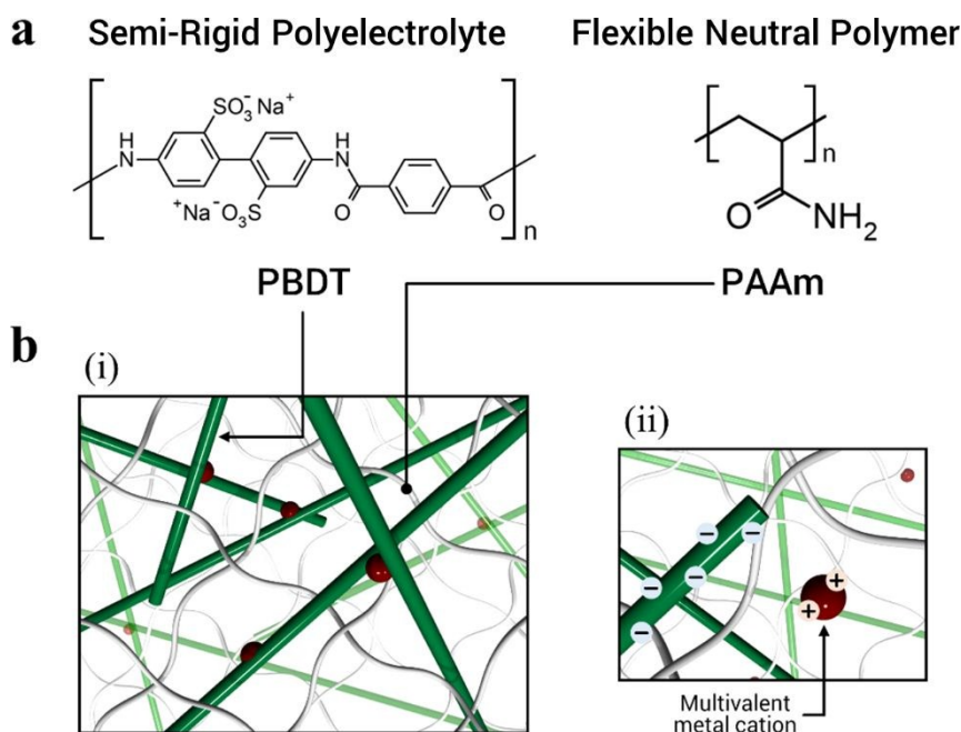
Figure 1. Fabrication concept for one-pot DN hydrogels utilizing a semi-rigid polymer-based physical sacrificial network. a) Chemical structures of the semi-rigid polyelectrolyte, PBDT, and flexible neutral polymer, polyacrylamide (PAAm). b) (i) Schematic illustration of the semi-rigid polymer network formed inside the stretchable polymer network via immersion in multi-valent ion solutions. The persistence length of PBDT is ~100 times greater than PAAm, and therefore is depicted as rod-like for illustration purposes. (ii) Crosslinking of the sacrificial network occurs by physical bonding between the negatively charged PBDT and positively charged ions. The green chains, grey chains and red spheres represent the PBDT, PAAm and multi-valent ions, respectively.
