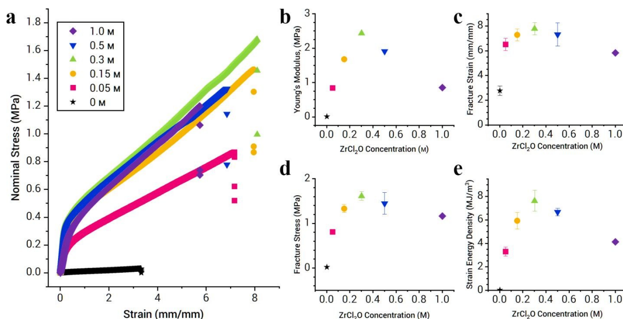
Figure 3. Mechanical properties of the 3% PBDT/PAAm gels immersed in \text{ZrCl}_2\text{O} solutions from 0 to 1 M. a) Stress-strain curves. b) Young's modulus. c) Strain at break. d) Stress at break. e) Strain energy density. The error bars are standard deviation from the results of 3-5 samples and are present unless the error bars are smaller than the symbol size.
