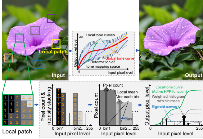
Fig. 1. Proposed algorithm's conceptual framework. We directly calculate smoothed local tone curve as sum of sigmoid functions, for each local patch which is computed from intensity stacked histogram.
