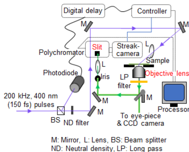
Figure 1. Optical setup for the time-resolved PL micro-spectroscopy.
