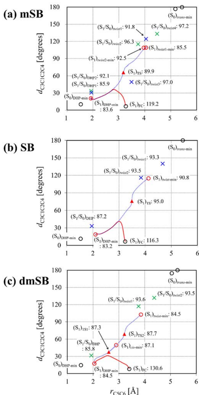
Figure 4. The minima, TSs, and MECI structures and the reaction pathways in the S_1 state for (a) mSB, (b) SB [31], and (c) dmSB [39] projected onto two-dimensional coordinate space in terms of r_{C5C6} and d_{C3C1C2C4} . The S_1 -minima and S_1 -TS are depicted by red circles and red triangles, respectively; the H-pyramidal S_1/S_0 -MECIs are given by blue cross marks, and the Me-pyramidal S_1/S_0 -MECIs are given by green cross marks. The S_0 -minima are also given by black circles. The meta-IRC path from the FC point is denoted by a solid red line, and the IRC paths are denoted by a blue dotted line. The S_1 energies (in kcal/mol) relative to (S_0)_{cis-min} are given for the respective structures.
