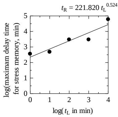
Fig. 3 Maximum delay time for stress memory with duration of preload application t_L for dry Shirahama Sandstone. Strain was measured by a clip gage.
