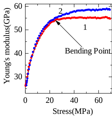
5 Fig. 14 An example of stress-tangent modulus curve pairs for specimen V-1.
