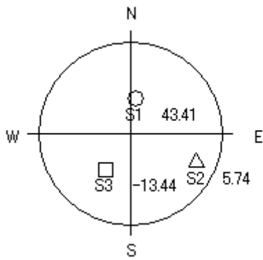
2 Fig. 13 Stereo projection of the stress state (MPa) measured using the pilot hole wall displacement method at AK 3 tunnel onto the lower hemisphere.
