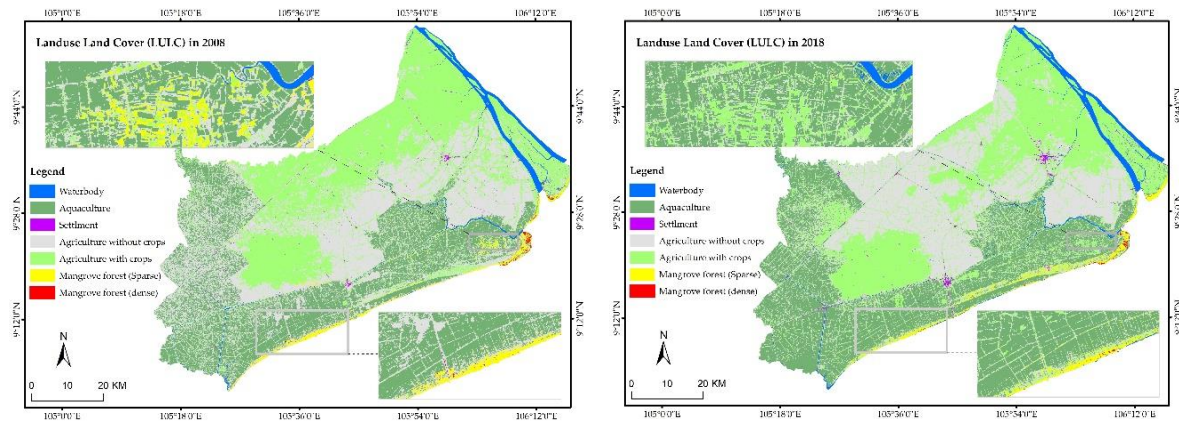
Figure 4. The LULC classification maps of Soc Trang and Bac Lieu provinces of the years 1988, 1998, 2008, and 2018, based on MLC of Landsat 5 TM (1988, 1998 and 2008) and Landsat 8 OLI (2018) images.
