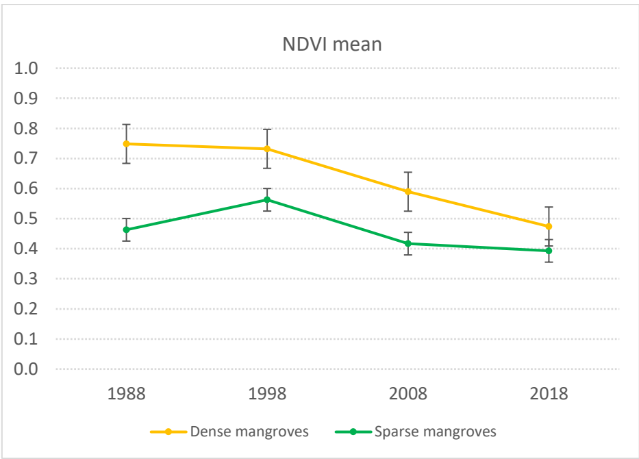
Figure 6. The NDVI mean values of dense and sparse mangroves in the years 1988, 1998, 2008, and 2018 (standard deviation values in table A5)
