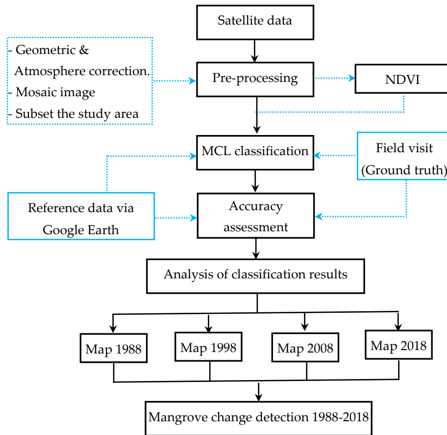
Figure 3. Flowchart of the methodology of the study.
