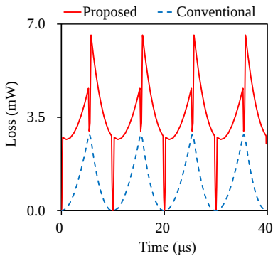
Fig. 16. Transient losses of 10-turn reactor in test circuit 2
