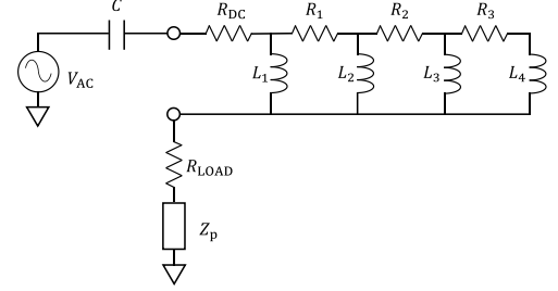
Fig. 13. Test circuit 1 for transient analysis
