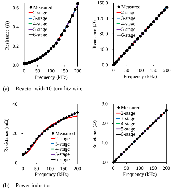
Fig. 11. Frequency dependence of reactor and power inductor
