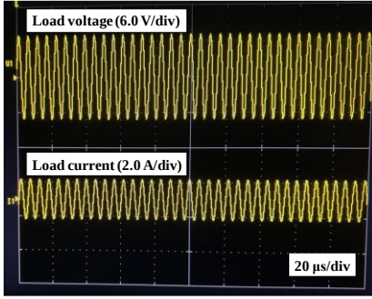
(a) Measured results of load voltage and load current
