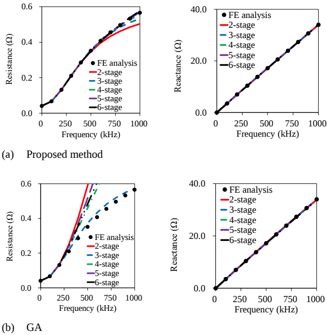
Fig. 9. High-frequency characteristics of equivalent circuits obtained with proposed method and GA
