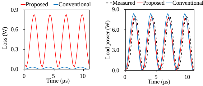
(b) Loss of 10-turn reactor
