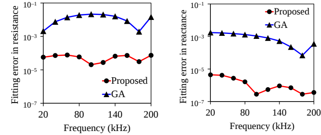
Fig. 5. Fitting errors with 4-stage circuit
