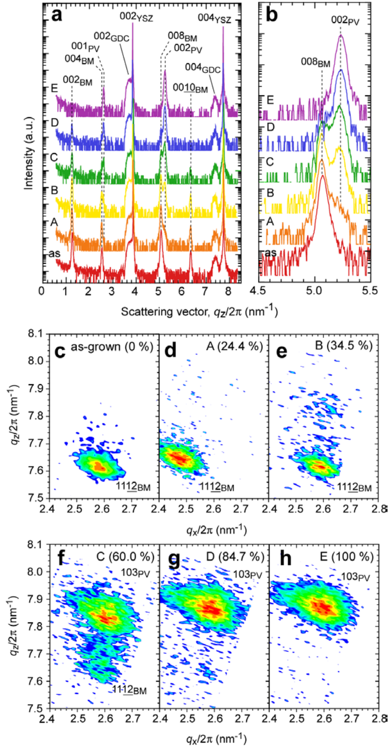
Figure 2. X-ray diffraction analyses of SrCoO x films with various oxidation states. (a) Out-of-plane XRD patterns. Intense diffraction peaks of 00 l_{\text{BM}} or 00 l_{\text{PV}} are seen together with 00 l_{\text{GDC}} /00 l_{\text{YSZ}} , indicating strong c -axis orientation of the films. (b) Magnified XRD pattern. With increasing the oxidation state, the peak position changed from 008 BM to 002 PV . (c)–(h) RSMs around 1112 BM or 103 PV . Although the diffraction spot was 1112 BM when the oxidation state is lower than 34.5 %, it changed into 103 PV when the oxidation state was greater than 60 %.
