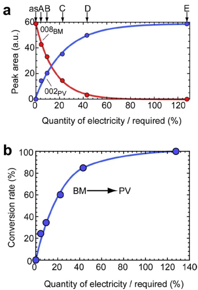
Figure S4. Calculation of the conversion rate from BM-SrCoO 2.5 into PV-SrCoO 3 . (a) Changes in the diffraction peak area of (red) 008 BM -SrCoO 2.5 and (blue) 002 PV -SrCoO 3-δ as a function of the quantity of electricity over required electricity. The required electricity is 9.6 mC. With increasing the electricity, the peak area of 002 PV increases rapidly and saturates whereas that of 008 BM decreases rapidly and approaches to zero. (b) Conversion rate from BM-SrCoO 2.5 into PV-SrCoO 3-δ . We assumed that sample E was fully oxidized. The conversion rate was calculated as (peak area of 002 PV )/(peak area of 002 PV for sample E ).
