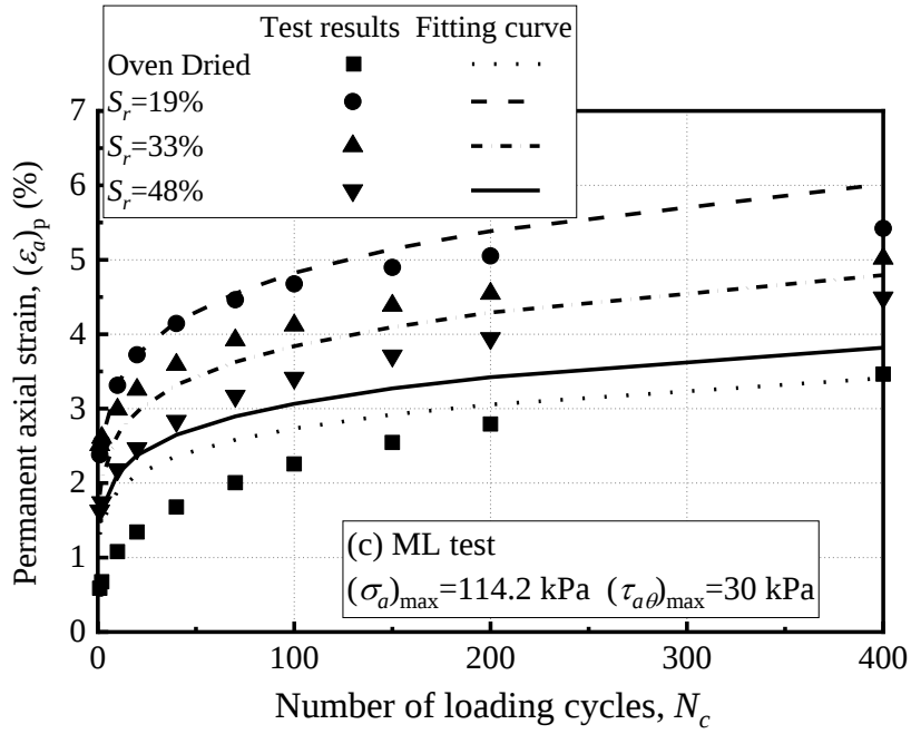
(c) ML test ((\tau_{a\theta})_{\max}=30 kPa)
