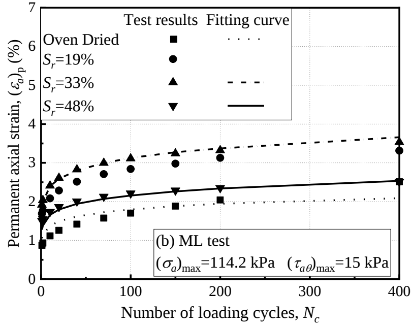
(b) ML test ((\tau_{a\theta})_{\max}=15 kPa)
