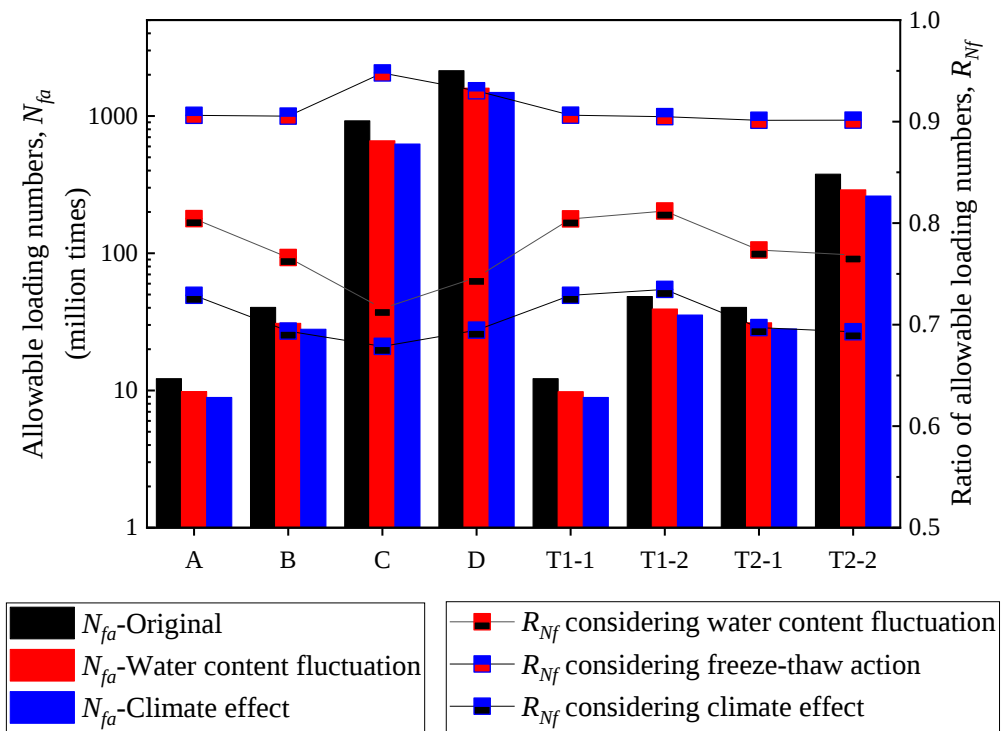
Figure 6-14 Fatigue life against rutting of eight test pavement structures
