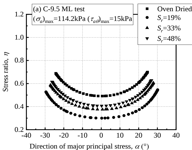
(a) C-9.5 ML test ((\tau_{a\theta})_{\max} = 15 \text{ kPa})
