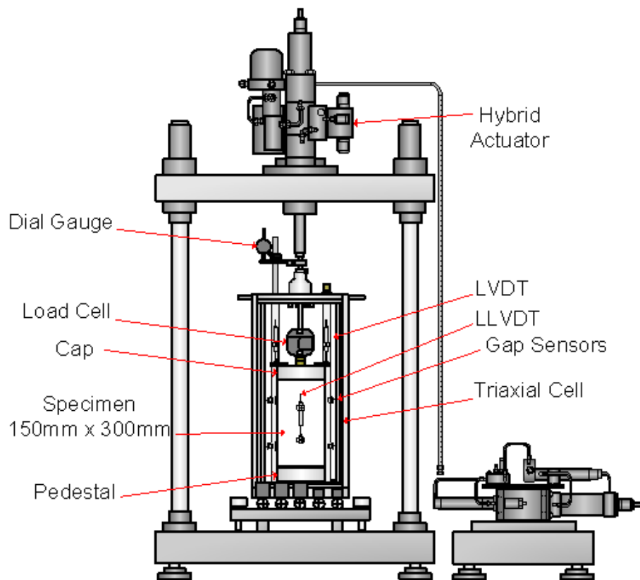
(a) Schematic diagram of test apparatus
