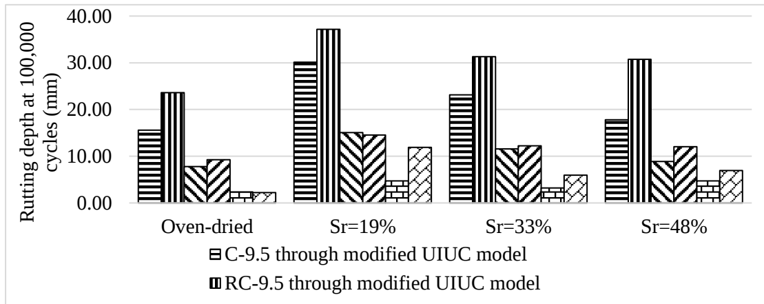
Figure 5-10 Computation of rutting depth using modified UIUC model
