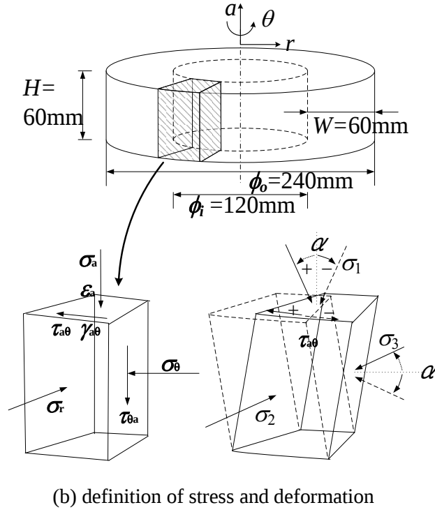
Figure 5-1 Multi-ring shear apparatus (after Ishikawa et al., 2011)
