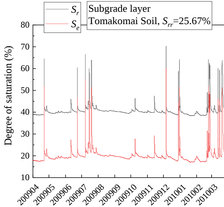
Figure 4-13 Long-term field measured degree of saturation of subgrade layer
