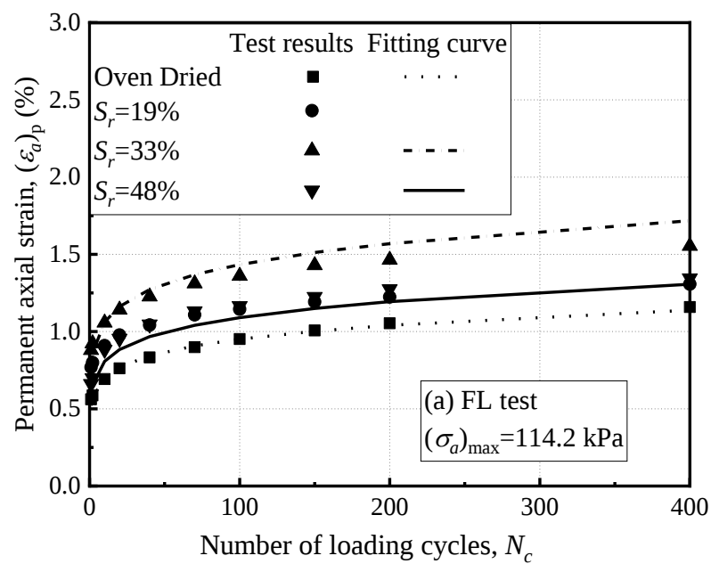
(a) FL test
