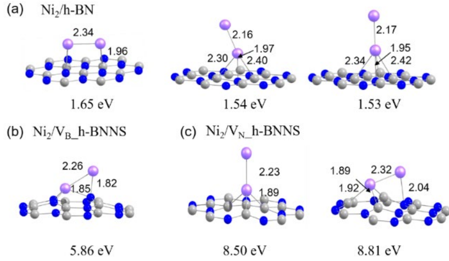
Fig. 4. Adsorption of \text{Ni}_2 on (a) pristine h-BN, (b) \text{V}_\text{B} -h-BNNS and (c) \text{V}_\text{N} -h-BNNS. The interatomic distances are given in Å. The adsorption energies of \text{Ni}_2 on surface are shown below the geometrical structure.
