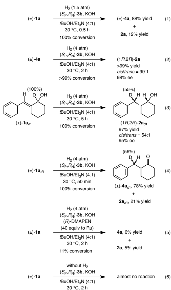
Scheme 3. Experiments for Mechanistic Consideration (S/C = 300).
