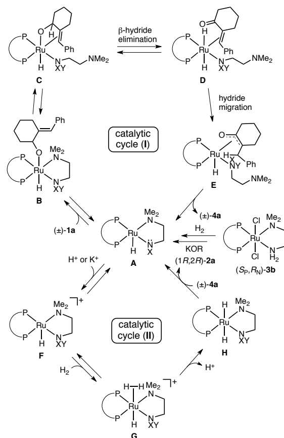
Scheme 4. Plausible Mechanism of the Isomerization–Hydrogenation Sequential Reaction of (\pm)\text{-1a} by a Ru catalytic system with Dual Roles. P–P = (S)-DM-SEGPHOS; X, Y = H or K; \text{NH}_2\text{—NMe}_2 = (R)-DMAPEN.
