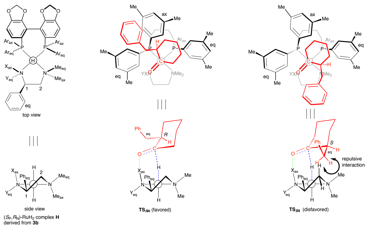
Figure 1. Structure of RuH 2 species H derived from (S P , R N )- 3b and diastereomeric TS-models in the hydrogenation of (±)- 4a through DKR (catalytic cycle (II)). Some aromatic groups and substituents in the TSs are omitted for clarity. X, Y = H or K. Ar = 3,5-(CH 3 ) 2 C 6 H 3 .
