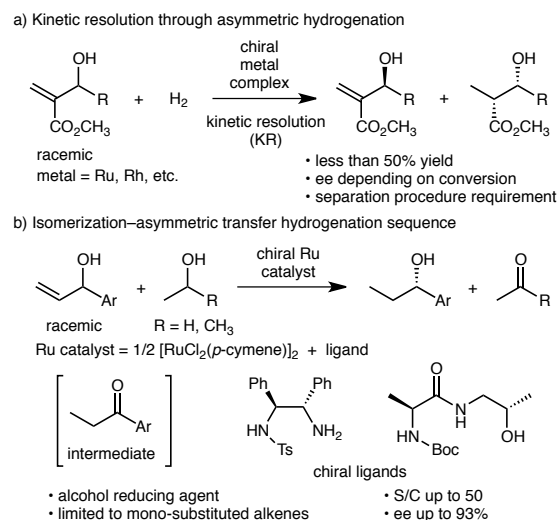
Scheme 2. Previous Works on the Formation of Optically Active Saturated Alcohols through Asymmetric (Transfer) Hydrogenation of Racemic Allylic Alcohols.
