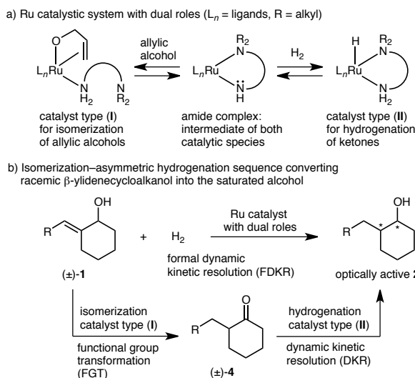
Scheme 1. Isomerization–Asymmetric Hydrogenation Sequence from Racemic Secondary Allylic Alcohols to the Optically Active Saturated Alcohols Using a Ru Catalyst with Dual Roles.
