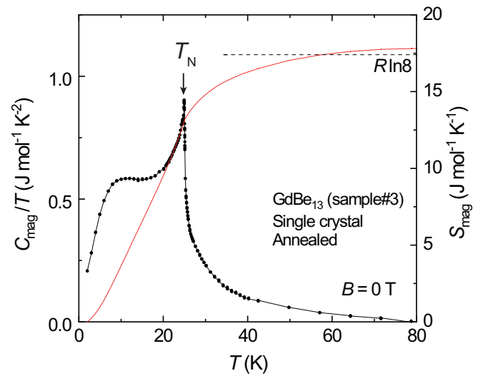
FIG. 3. Temperature dependence of C_{\text{mag}}/T (left axis) and S_{\text{mag}} (right axis) in \text{GdBe}_{13} at zero magnetic field. The horizontal dashed line represents the full entropy value of R\ln 8 for J = 7/2 .
