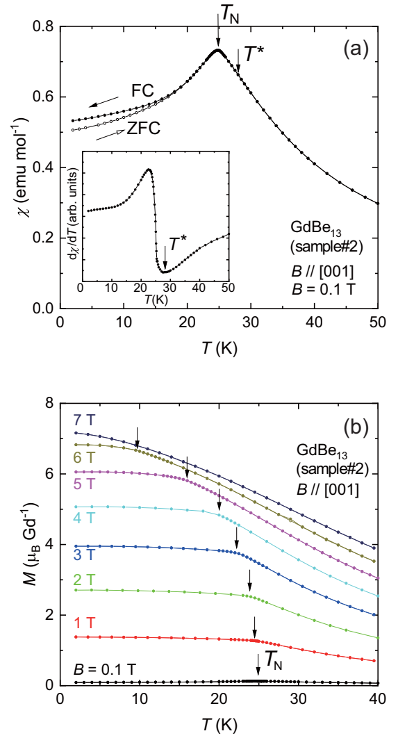
FIG. 6. (a) Temperature dependence of the magnetic susceptibility \chi(T) [= M(T)/B] for \text{GdBe}_{13} below 50 K at B = 0.1 T applied along [001]. The open and closed symbols represent the data upon ZFC and FC processes, respectively. The inset shows d\chi/dT as a function of T at 0.1 T. (b) Temperature dependence of the magnetization M(T) at several fields up to 7 T for B \parallel [001] .
