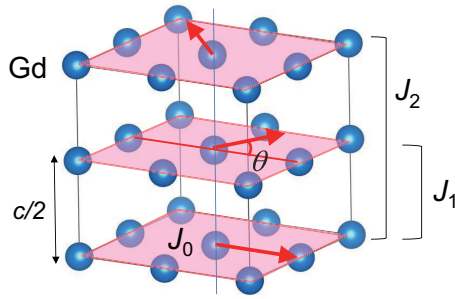
FIG. 9. Generic helical structure of \text{GdBe}_{13} . The Heisenberg exchange interactions J_0 , J_1 , and J_2 are indicated in this figure. \theta is the turn angle of the magnetic moment between adjacent layers. The distance between adjacent layers corresponds to a half of the lattice constant of the FCC lattice.
