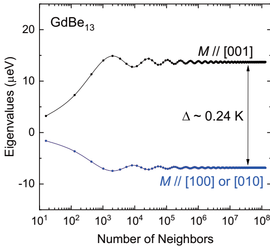
FIG. 11. Convergence behavior of the eigenvalues of the Fourier transform of the dipole interaction tensor J_{\alpha\beta}(\mathbf{q}_0) in \text{GdBe}_{13} with respect to number of neighbor ions. The definition of J_{\alpha\beta}(\mathbf{q}_0) is referred to Ref. [39].
