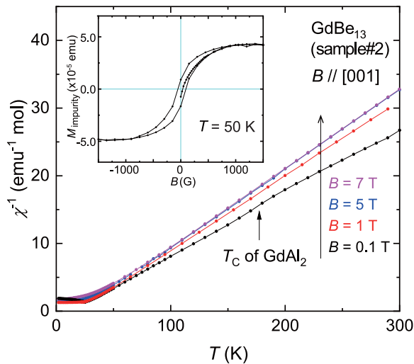
FIG. 12. Temperature dependence of the inverse magnetic susceptibility \chi^{-1}(T) at B = 0.1, 1, 5 , and 7 T in \text{GdBe}_{13} for the annealed sample 2. B is applied along the [001] direction. The closed arrow located at 175 K indicates T_C of \text{GdAl}_2 . The inset shows M_{\text{impurity}} vs magnetic field near zero field at 50 K. M_{\text{impurity}} was obtained by subtracting the paramagnetic component from M of the measured sample.
