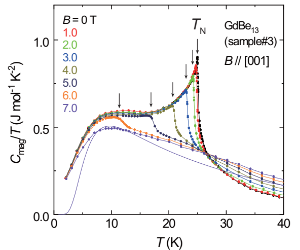
FIG. 4. Temperature dependence of C_{\text{mag}}/T for \text{GdBe}_{13} at several magnetic fields up to 7 T. The magnetic field is applied along the [001] axis. The solid curve represents the calculation result of the Schottky specific heat assuming the splitting of the J = 7/2 octet.
