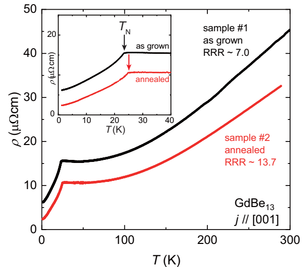
FIG. 1. Temperature dependence of the electrical resistivity \rho(T) of \text{GdBe}_{13} for the as-grown and annealed single-crystalline samples. The inset shows the enlarged view below 40 K. The arrows indicate the transition temperature T_N .
