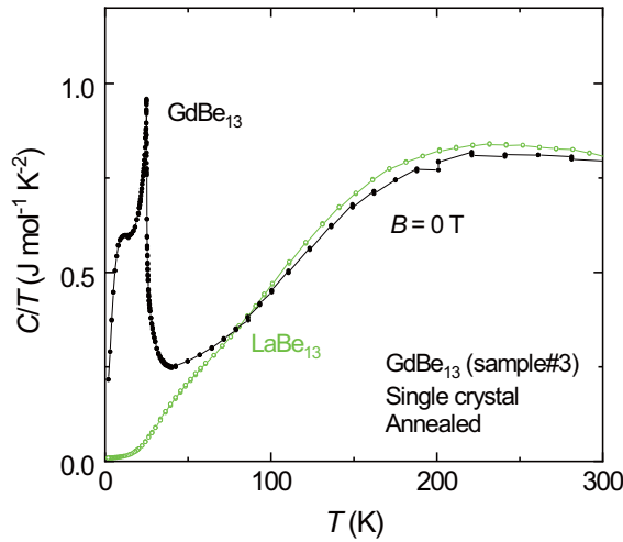
FIG. 2. Temperature dependence of C/T for \text{GdBe}_{13} (closed circles) and \text{LaBe}_{13} (open circles) [15] below 300 K at zero field.
