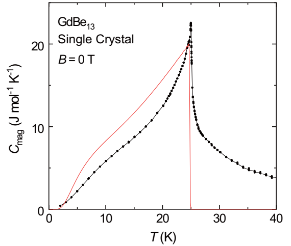
FIG. 10. Magnetic contribution to the specific heat C_{\text{mag}} as a function of temperature for GdBe 13 at B = 0 T. The red line represents the data obtained from the MF calculation based on the results in the present \chi(T) measurements.
