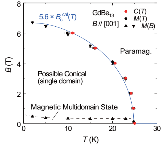
FIG. 8. Magnetic field-temperature ( B - T ) phase diagram of \text{GdBe}_{13} for B \parallel [001] , constructed from the M and C measurements using the annealed single crystals. The dashed curve is guide to the eye, while the solid curve indicates 5.6 \times B_c^{\text{cal}}(T) obtained by the MF calculation (see text).
