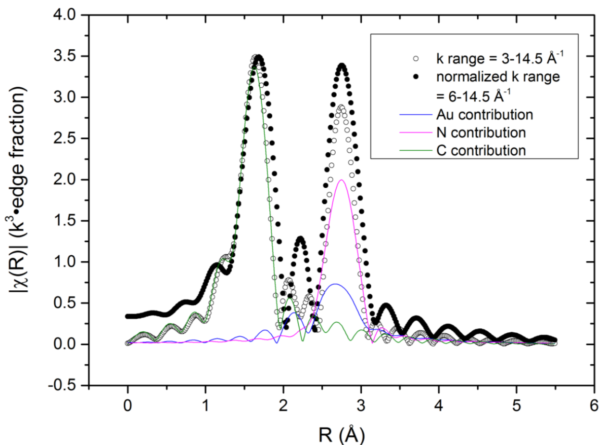
Figure 4.12 Contribution of each shell to the spectrum both complete k range and high k range.
