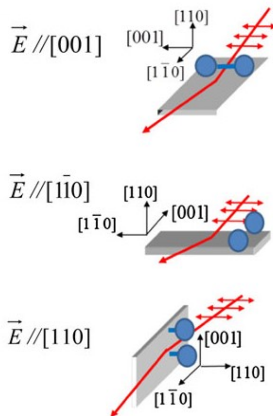
Figure 3.3 Three possible orientations for PTRF-XAFS measurements. Red arrows show the electric vector direction [4].
