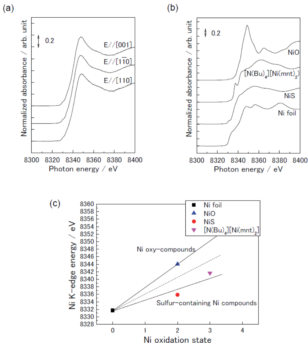
Figure 3.8 (a) Ni K-edge XANES spectra of Ni/o-MBA/TiO 2 (110) in three different polarization directions. (b) Ni K-edge XANES spectra of reference compounds which are Ni metal (Ni foil), oxy-compound with Ni-O bonds (NiO) and sulfur-containing compounds with Ni-S bonds (NiS and [N(Bu) 4 ][Ni(mnt) 2 ]). (c) Plot of Ni K-edge energies for the reference compounds as a function of oxidation state. The dotted line shows the intermediate one between the lines corresponding to the oxy- and sulfur-containing compounds.
