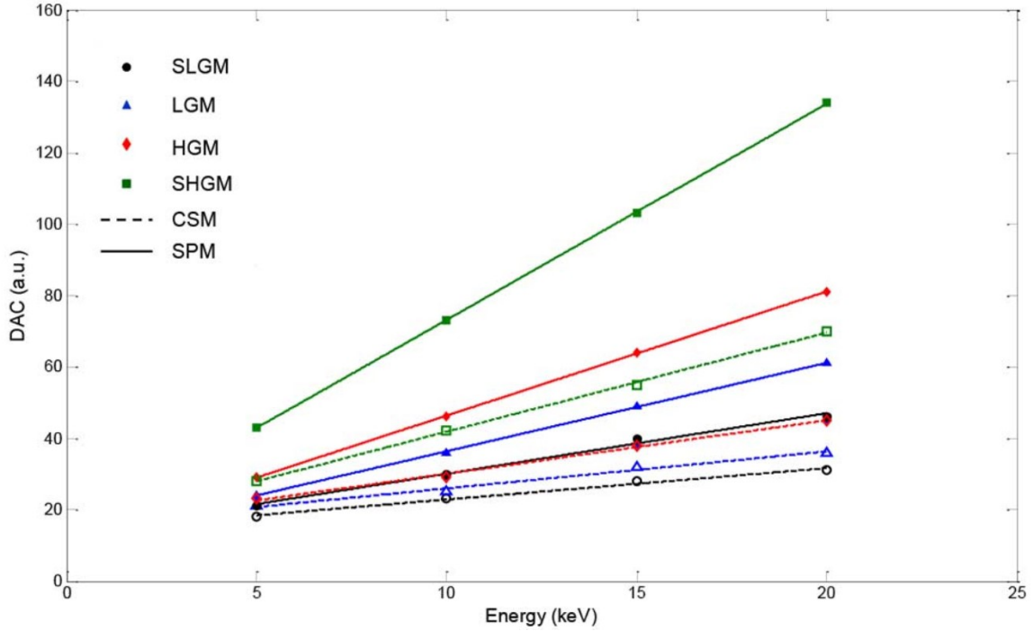
Figure 2.5 Linearity response (markers) and fits (lines) of the detector at different energies for Single Pixel Mode (solid line) and Charge Summing Mode (dash lines) for each of the four gains [1].
