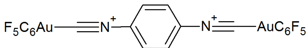
Figure 4.1 molecular structure of 1 or (\text{C}_6\text{F}_5\text{Au})_2(\mu\text{-1,4-diisocyano benzene}) .
