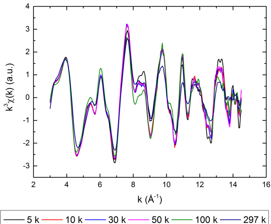
Figure 4.7 XAFS oscillation of various temperature of measurements.
