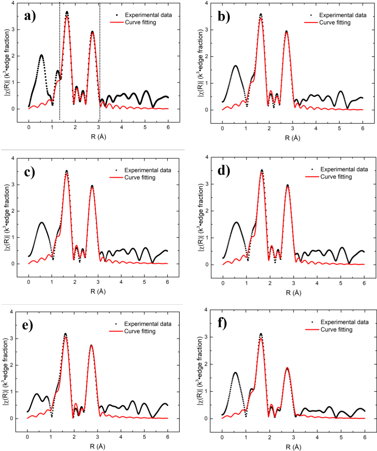
Figure 4.8 R space curve fitting of each measurement temperature a) 5 K, b) 10 K, c) 30 K, d) 50 K, e) 100 K, and f) 297 K. The dotted lines indicate the fitting range.
