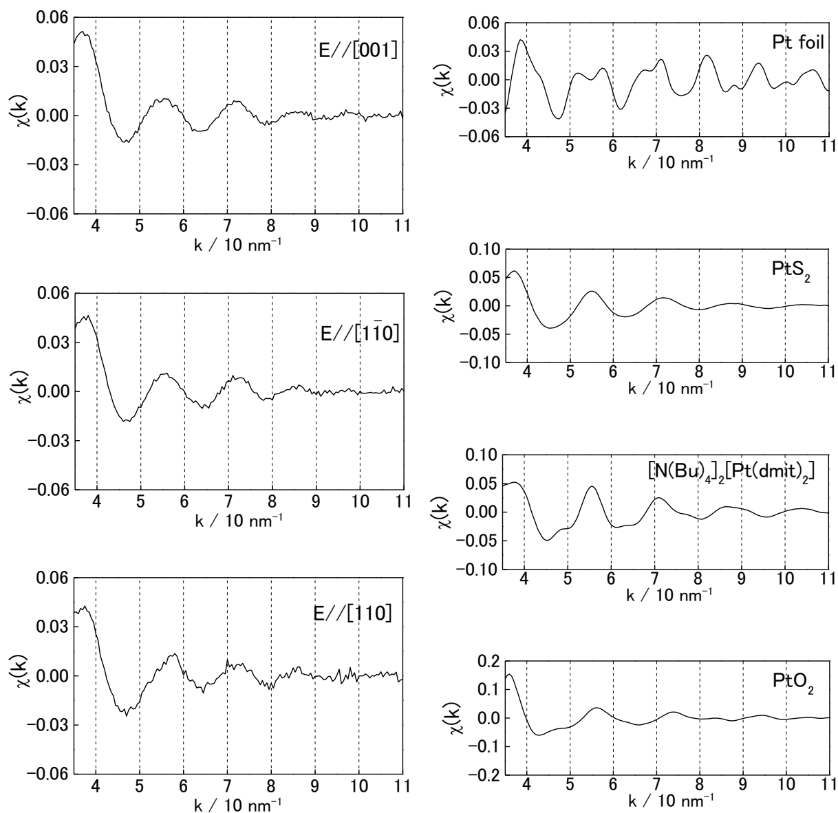
Figure 3.10 (a) Pt L_3 -edge XAFS spectra of Pt/o-MBA/TiO 2 (110) obtained at three different polarization directions. (b) Pt L_3 -edge XAFS spectra of reference samples (Pt foil, platinum sulfide (PtS 2 ), bis(tetrabutylammonium) bis(1,3-dithiole-2-thione-4,5-dithiolato) platinum(II) ([N(Bu) 4 ] 2 [Pt(dmit) 2 ]), and platinum oxide (PtO 2 )).
