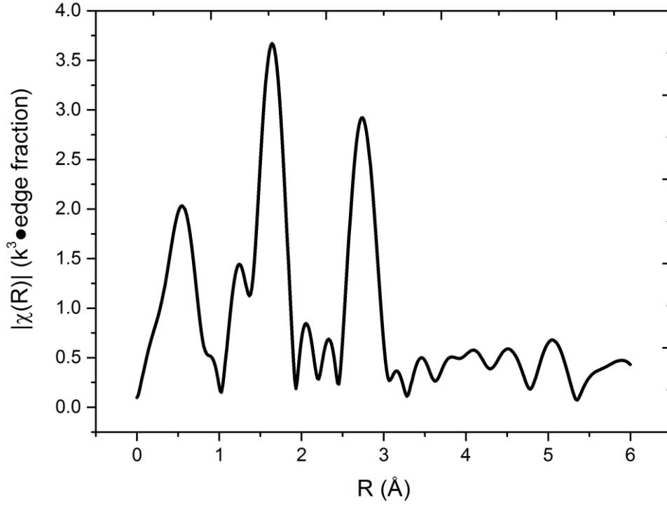
Figure 1.6 Fourier transformation of spectrum in figure 1.4.
