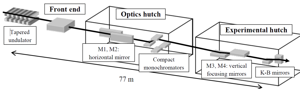
Figure 5.2 Schematic of the beamline BL36XU [3].
