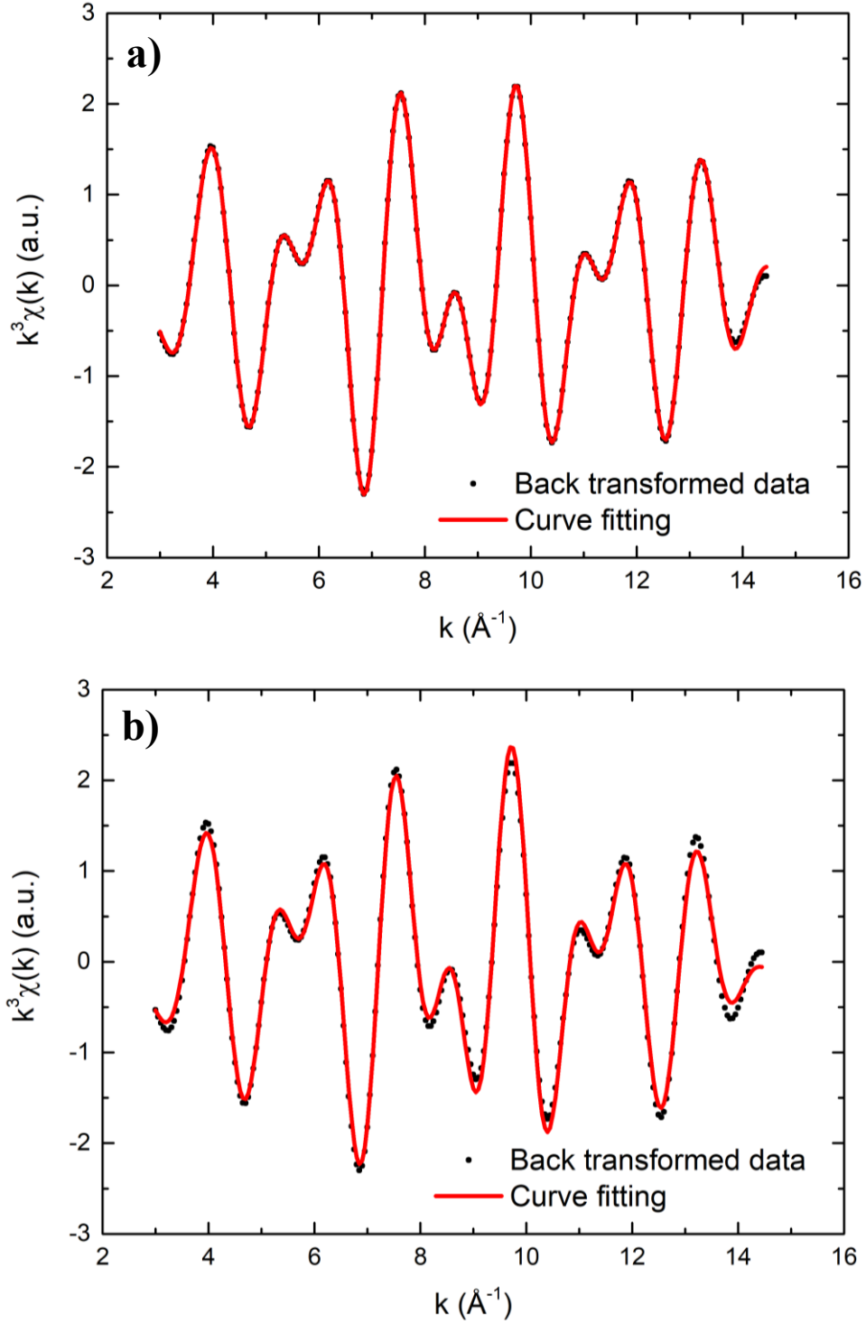
Figure 4.11 The same results as shown in figure 4.10 but in back k space or inverse Fourier transform.
