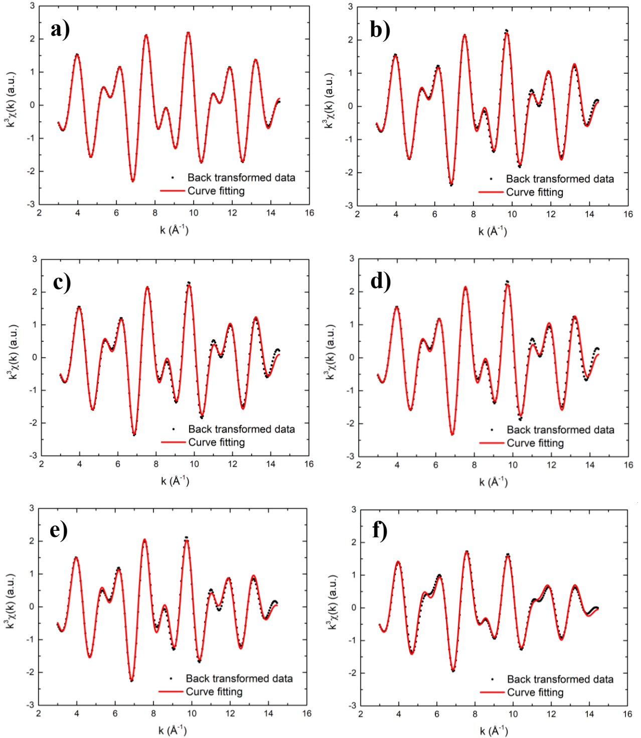
Figure 4.9 Back k -space or inverse Fourier transform curve fitting of each measurement temperature a) 5 K, b) 10 K, c) 30 K, d) 50 K, e) 100 K, and f) 297 K.
