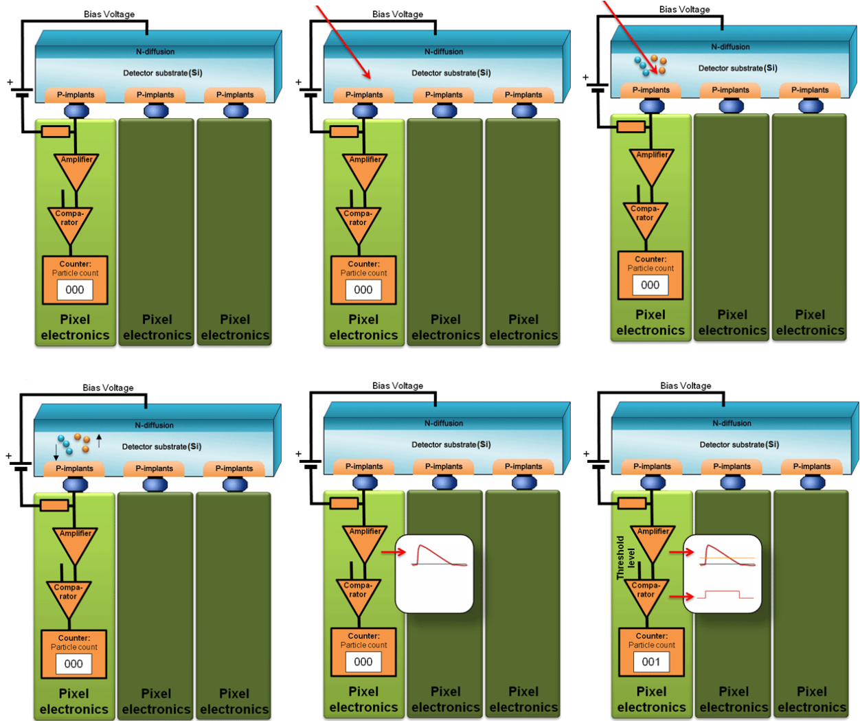
Figure 2.4 Principle of the phonon counting in a single pixel [2]. (From left to right, from top to bottom) The radiation generates electron-hole pairs (charge) in the sensor. The charge is collected to the appropriate pixel, amplified and compared with a pre-set comparator level (energy threshold). The counter is increased if the detected pulse is above the energy level.
