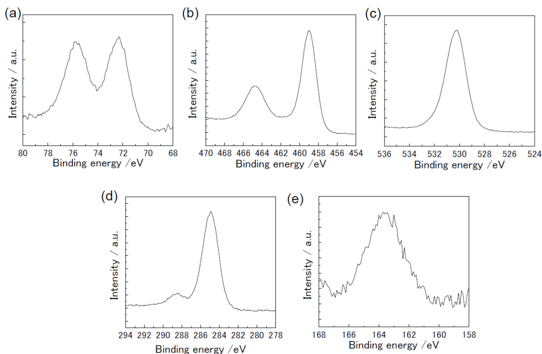
Figure 3.9 (a) \text{Pt}4f , (b) \text{Ti}2p , (c) \text{O}1s , (d) \text{C}1s and (e) \text{S}2p XPS spectra of Pt/ o -MBA/ \text{TiO}_2(110) .
