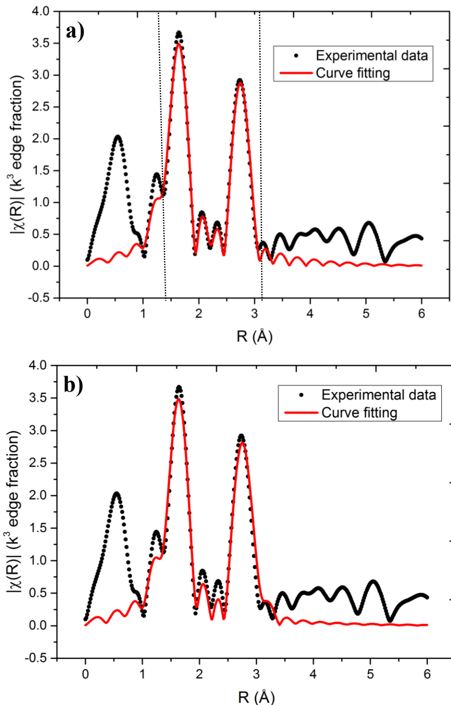
Figure 4.10 a) The curve fitting results of the 5 K data as shown in figure 4.6 (a) (include gold atom in the fitting) b) The result when exclude gold atom in the fitting. The dotted lines indicate the fitting range.
