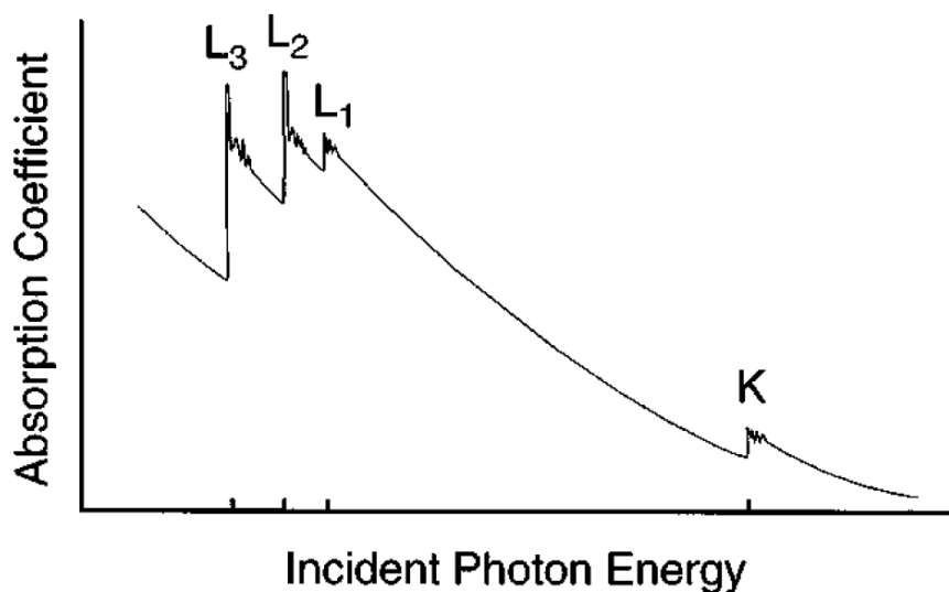
Figure 1.1 Schematic view of x-ray absorption coefficient as a function of incident photon energy. Four x-ray edges are shown: K, L_1 , L_2 , and L_3 . Note that the overall decrease in absorption as a function of energy is punctuated by four sharps, step-function-like increases at each edge. Above each edge are the oscillatory wiggles known as the EXAFS.
