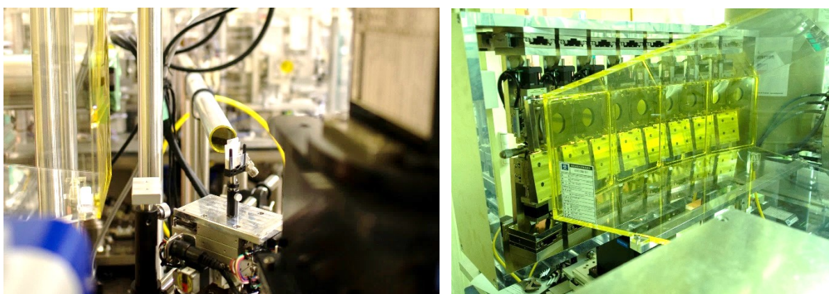
Figure 5.3 Pictures of experimental setup. Left: Sample stage, Right: Crystal Analyzers.
