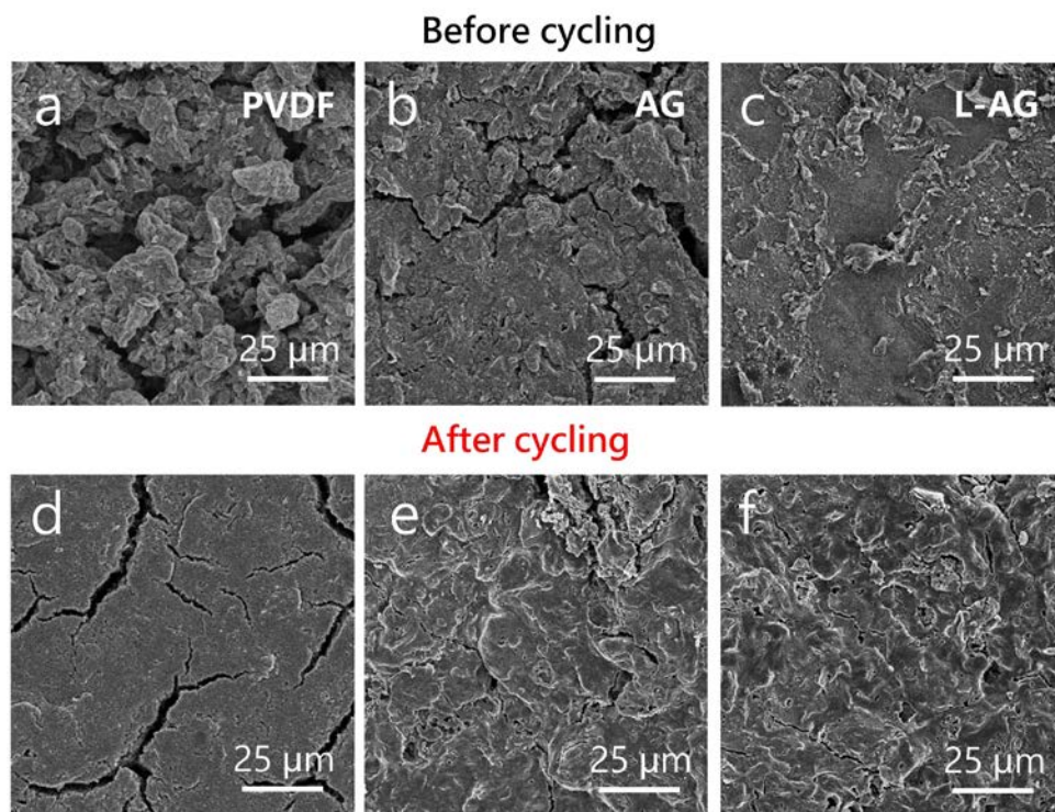
Figure 3. SEM images of the electrodes with PVDF, AG and L-AG binders before (a-c) and after the cycling (d-f).
