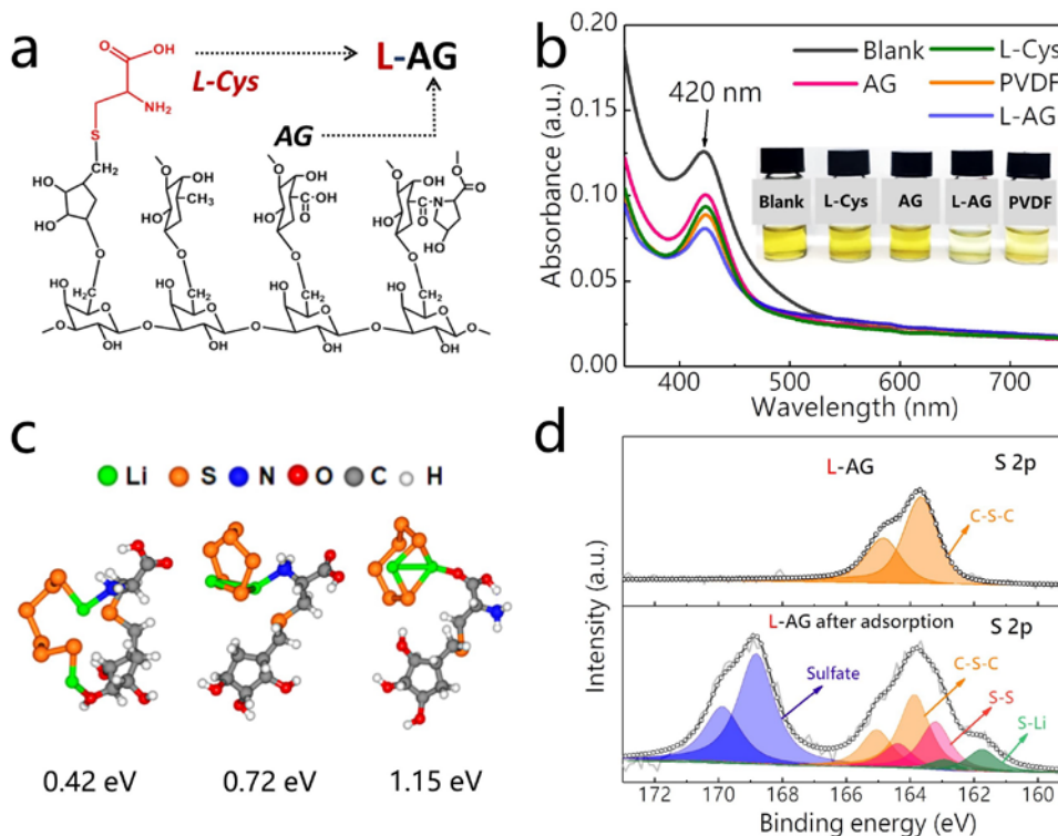
Figure 1. (a) The chemical structure of L-AG. (b) Photos of the Li 2 S 6 (1 mM) adsorption by L-Cys, AG, L-AG and PVDF in DOL/DME solution and the UV-Vis curves of Li 2 S 6 solution before and after adsorption. (c) Adsorption geometries and binding energies of Li 2 S 6 on the -NH 2 and -COOH groups in L-AG. (d) The S 2p XPS profiles of L-AG and L-AG after Li 2 S 6 adsorption.
